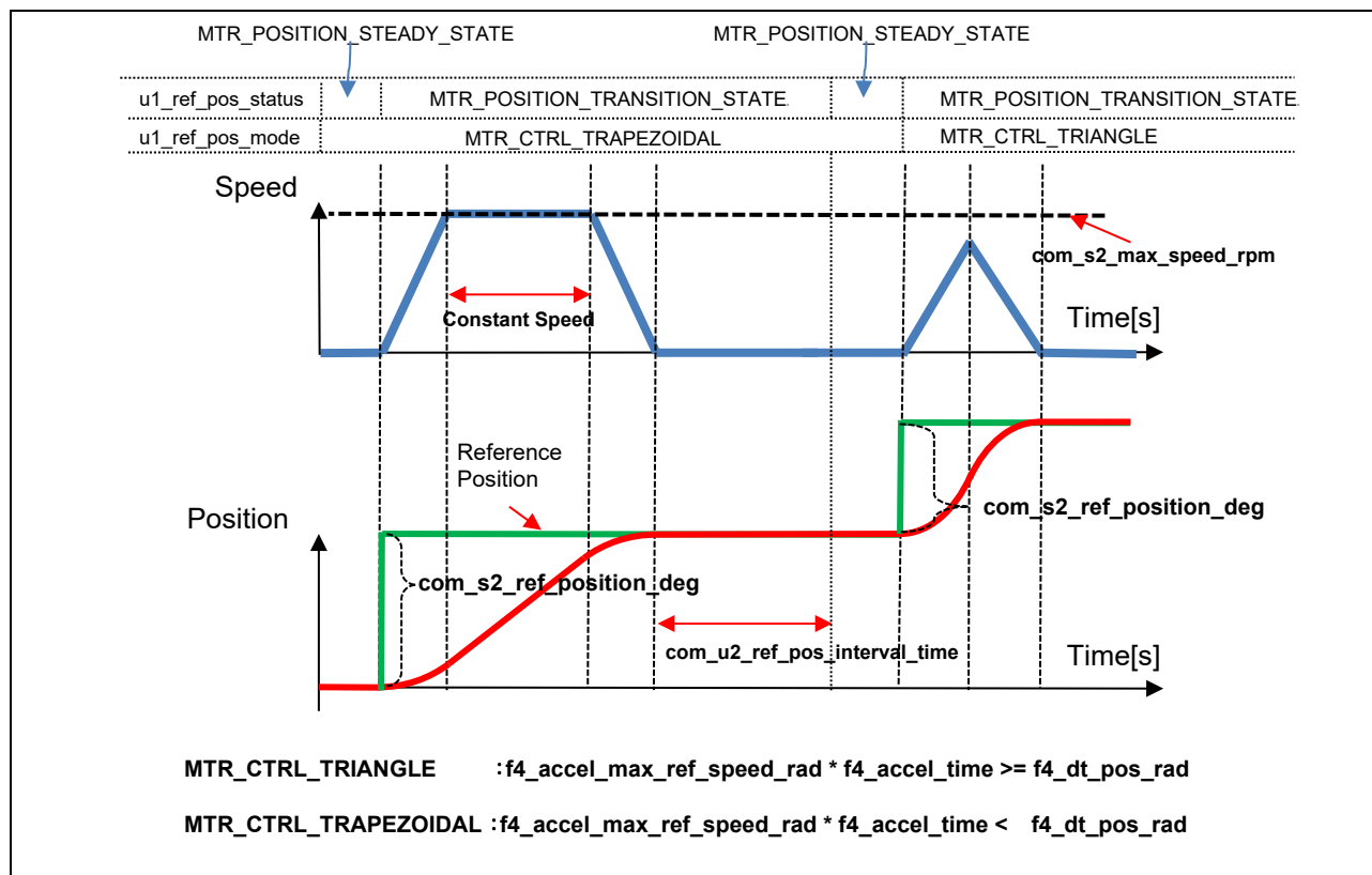
Figure 3-1 Position Profile Generation
