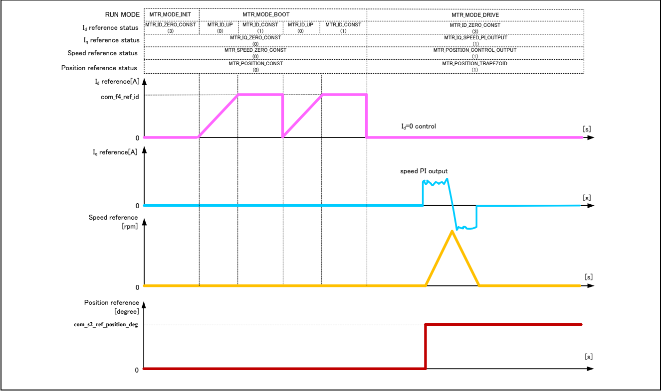
Figure 3-6 Startup Position Control of Vector Control PMSM with Encoder Software
