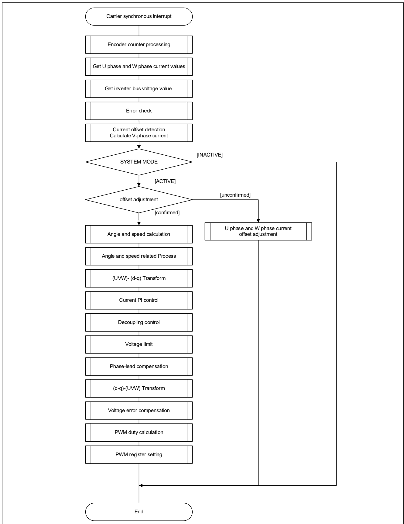
Figure 3-10 Carrier Synchronous Interrupt Handling (100 [μs])
