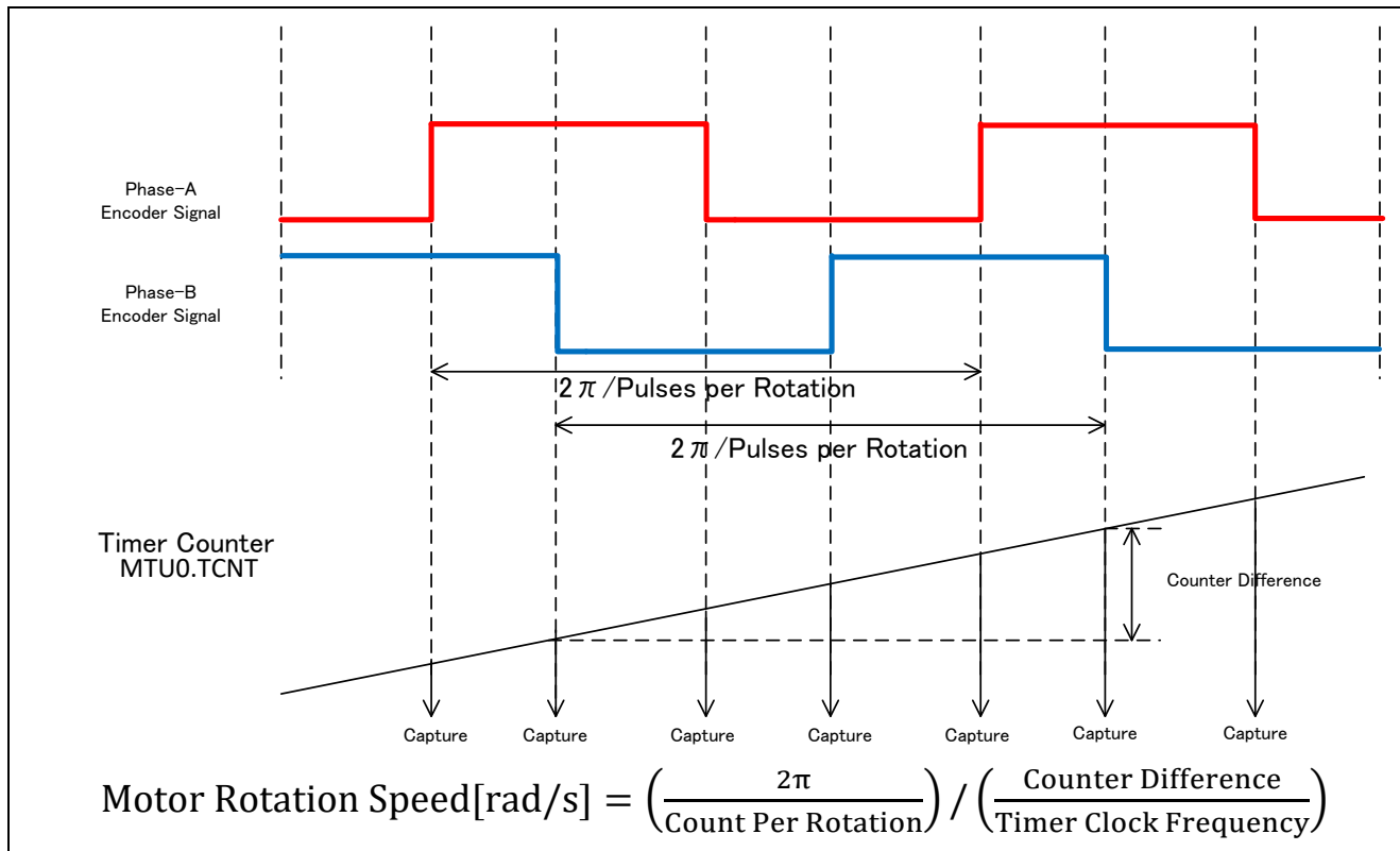
Figure 3-2 Speed Calculation using Encoder
