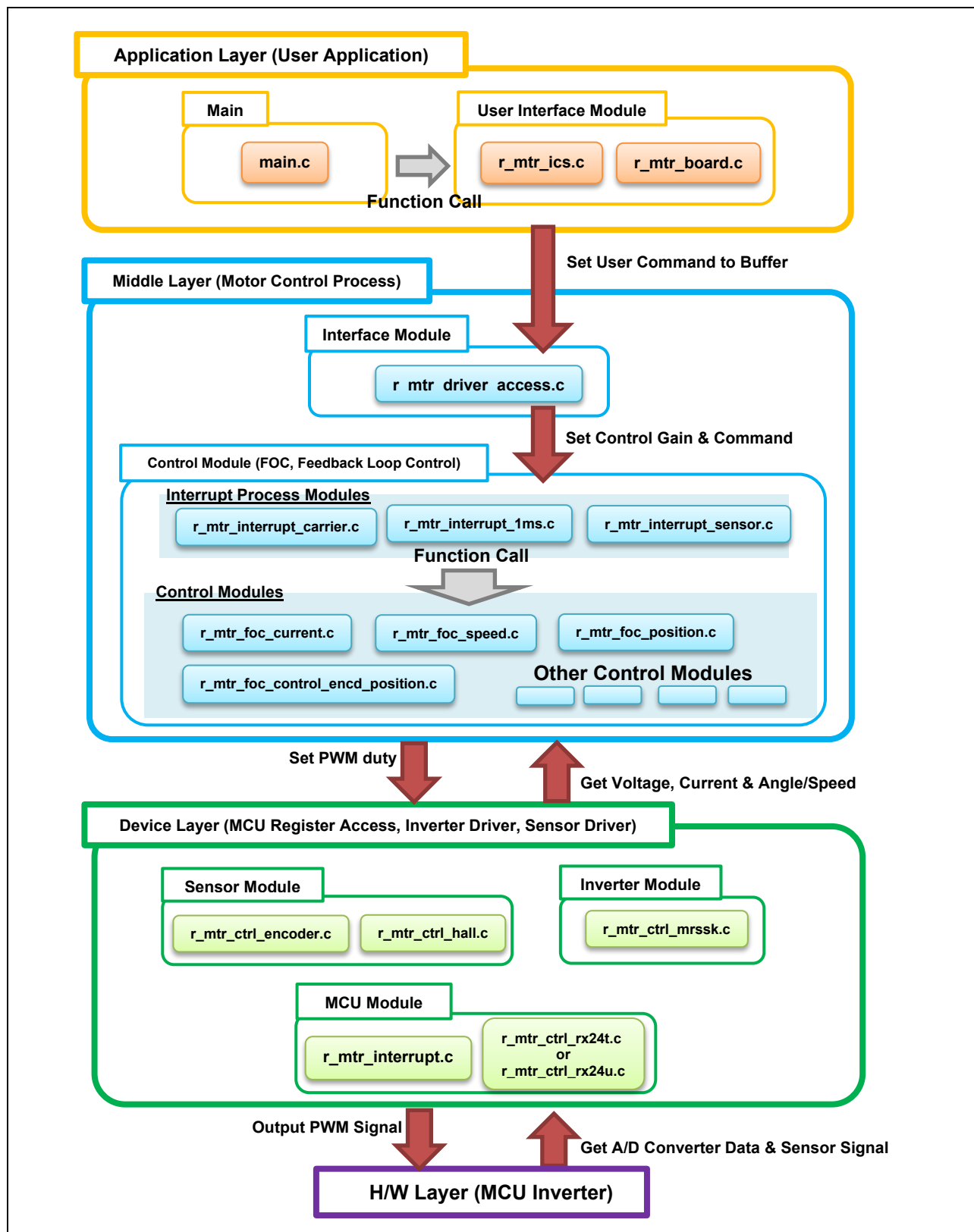
Figure 2-4 Module Configuration
