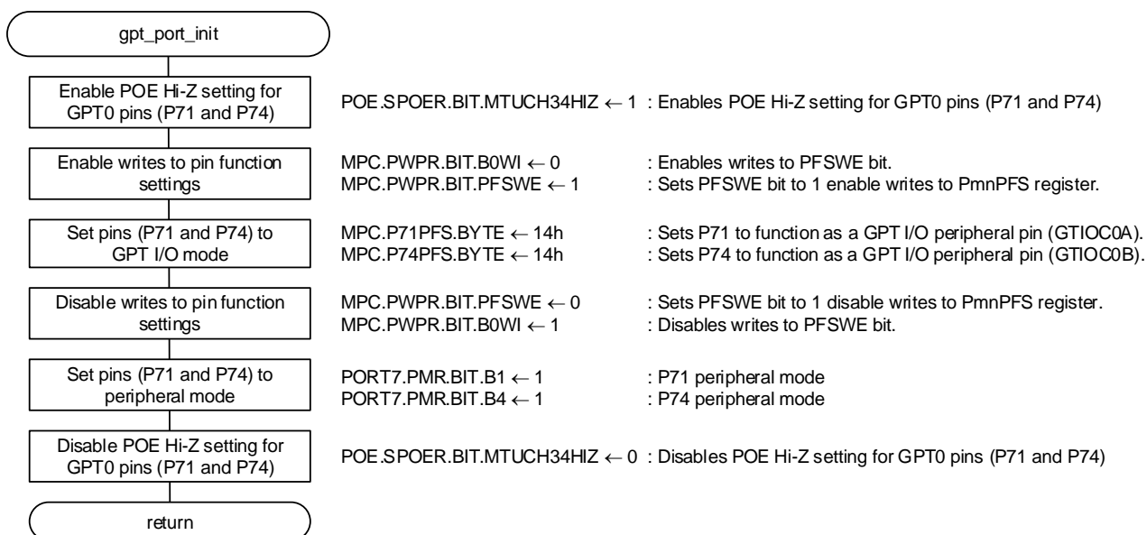
Figure 4.9 GPT I/O Pin Initialization
