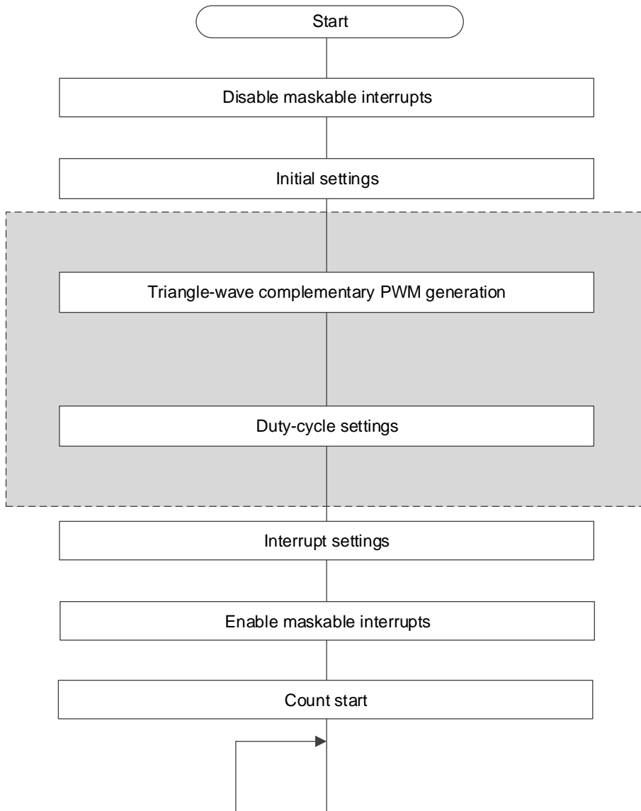
Figure 1.3 Flowchart of Sample Code
