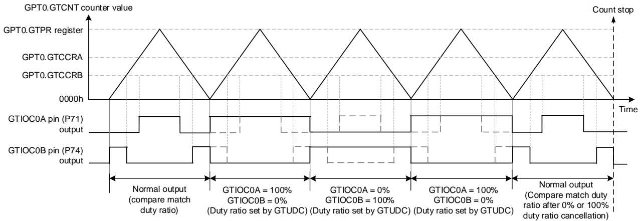
Figure 1.1 PWM Output Produced by rx24u_gpt_sample1
