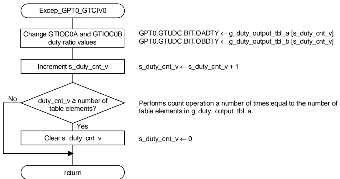
Figure 4.10 GTCIV0 Interrupt Handler
