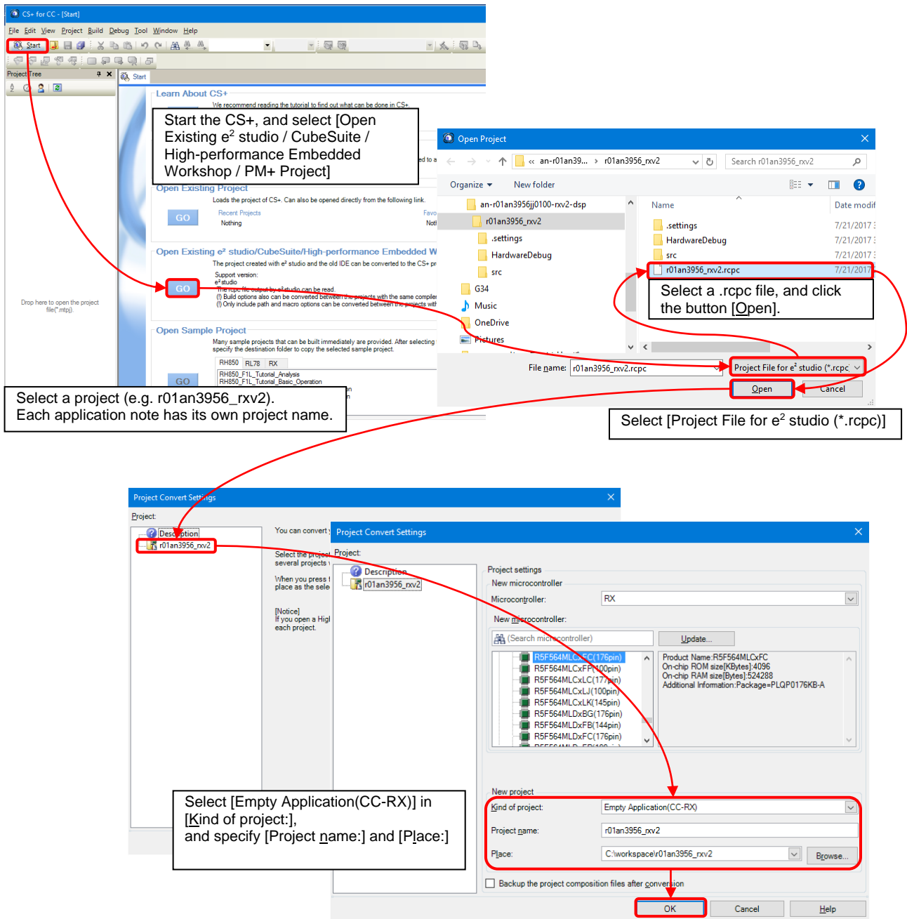
Figure 5.2 Importing a Project into CS+
