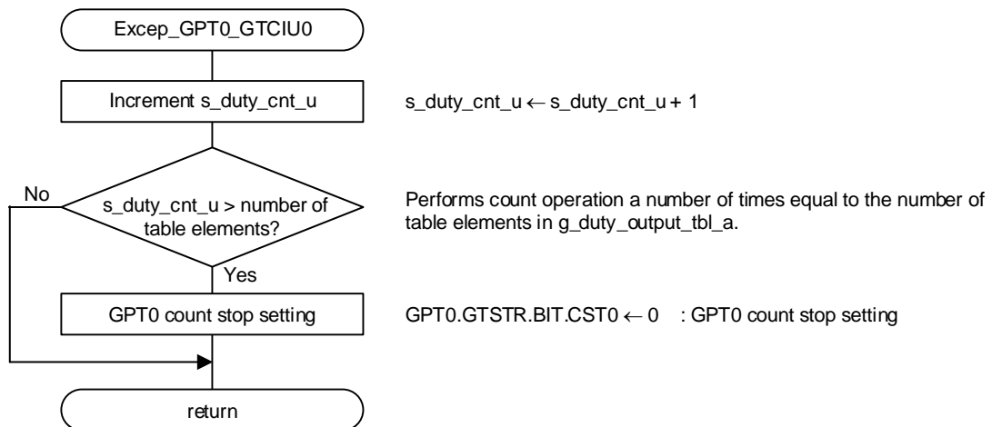
Figure 4.11 GTCIU0 Interrupt Handler
