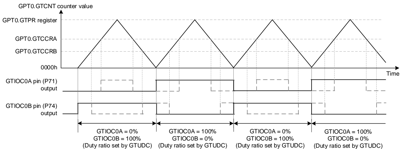
Figure 1.2 PWM Output Produced by rx24u_gpt_sample2
