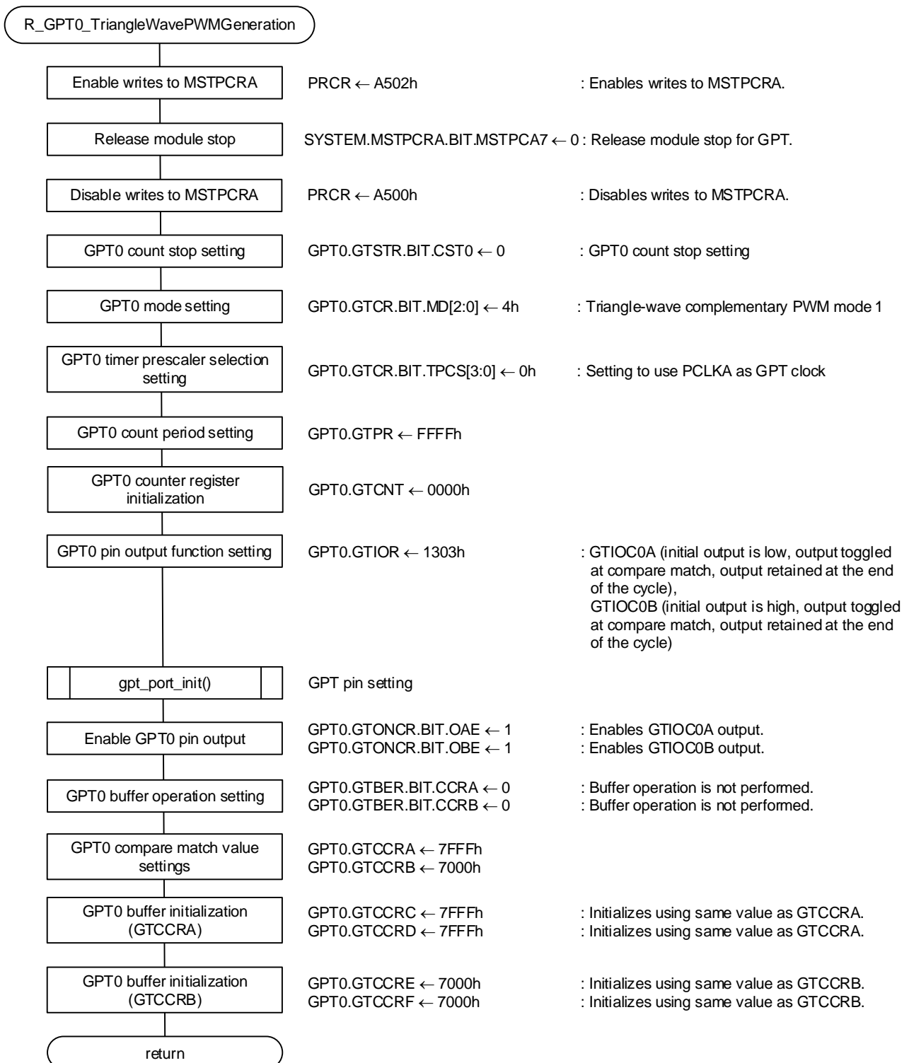
Figure 4.5 Triangle-Wave Complementary PWM Generation
