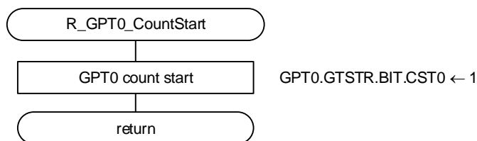
Figure 4.8 Count Start
