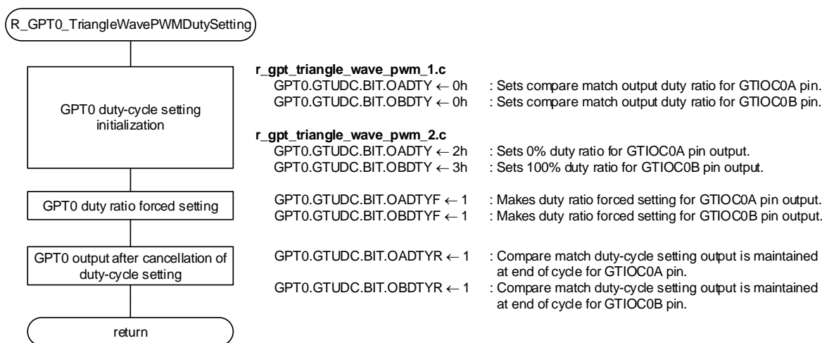
Figure 4.6 Duty-Cycle Settings
