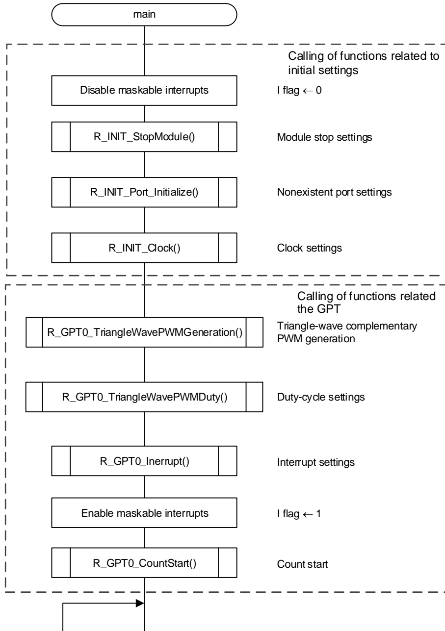
Figure 4.4 Main Processing Routine
