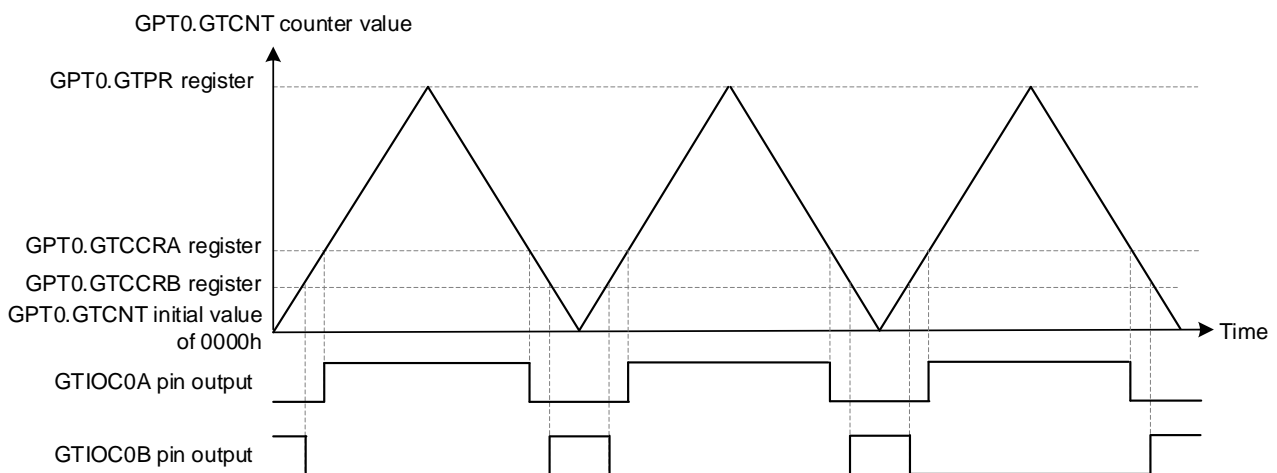
Figure 4.1 Triangle-Wave Complementary PWM Mode 1 Signal Generation Example (GTCCRA > GTCCRB)
