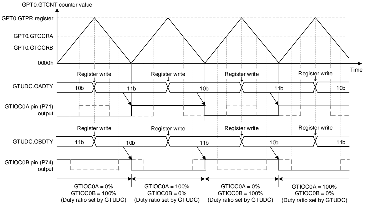
Figure 4.3 Example of Initial Duty Ratio (Count Stop) Setting and Its Reflection in Output after Count Operation Start
