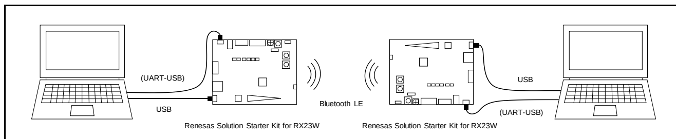
Figure 3-1 Demo Configuration of the Sample Program
