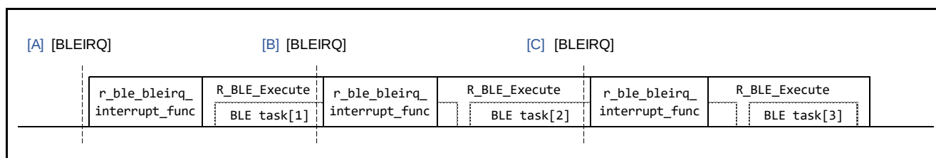
Figure 2-3 Bluetooth LE Communication Events with High Frequency
