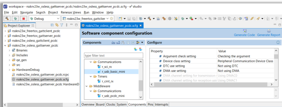
Figure 3-25 Configuration of USB Basic Mini FIT Module (r_usb_basic_mini)
