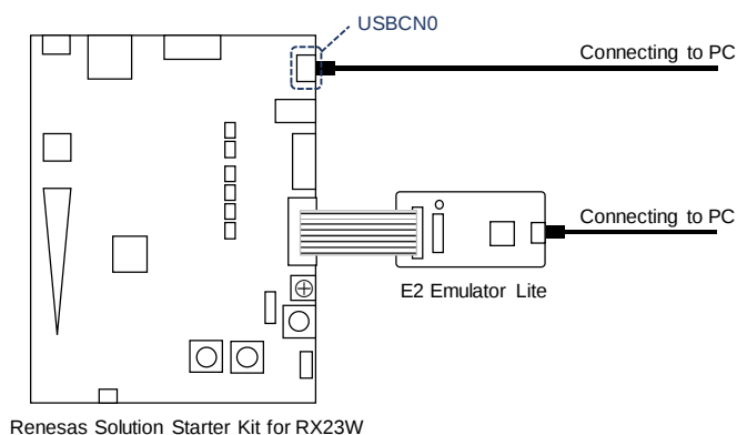
Figure 3-13 Connections of the Evaluation Board for Writing a Program File
