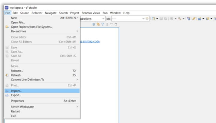
Figure 3-7 [File]→[Import...]
