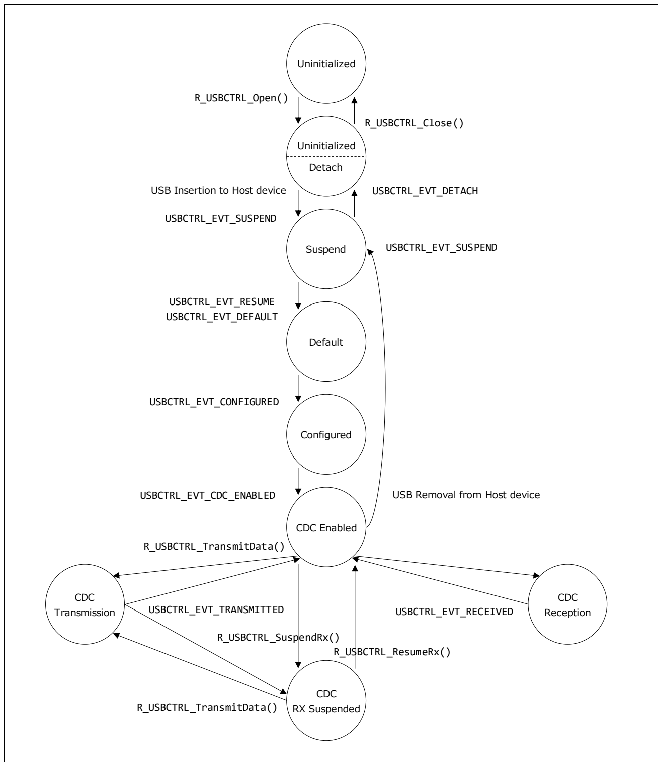
Figure 3-21 State Transition of USB Control Processing
