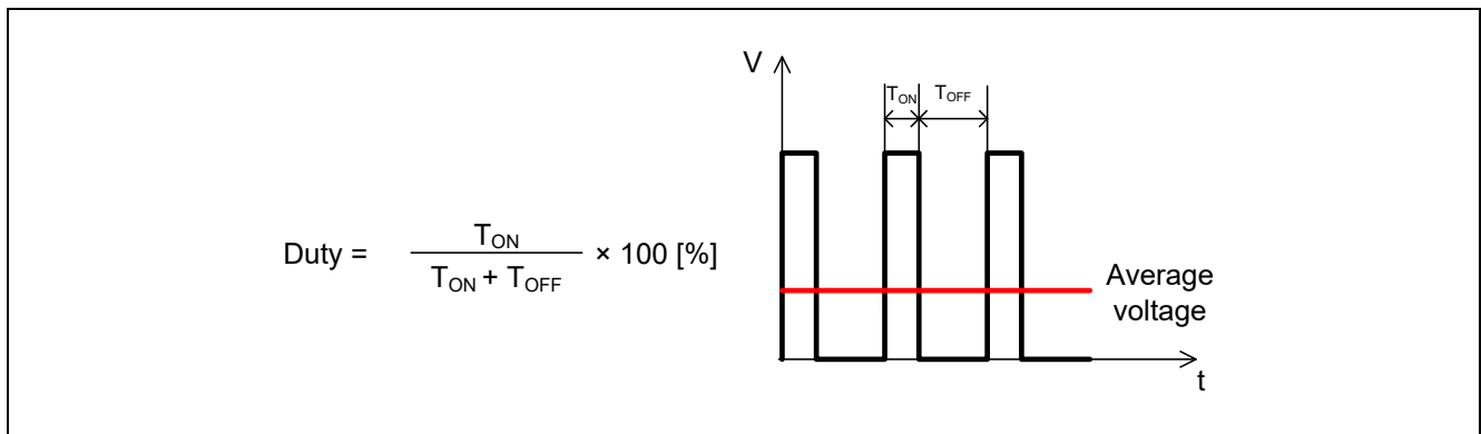
Figure 3-2 PWM Control
