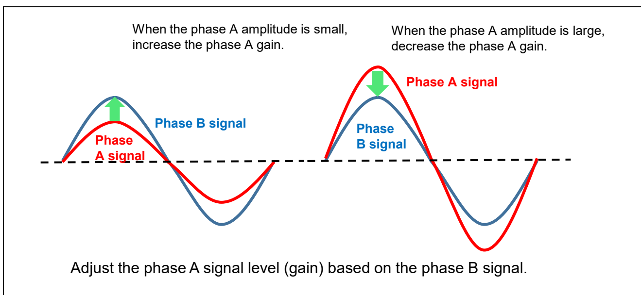
Figure 3.18 Resolver Signal Gain Adjustment
