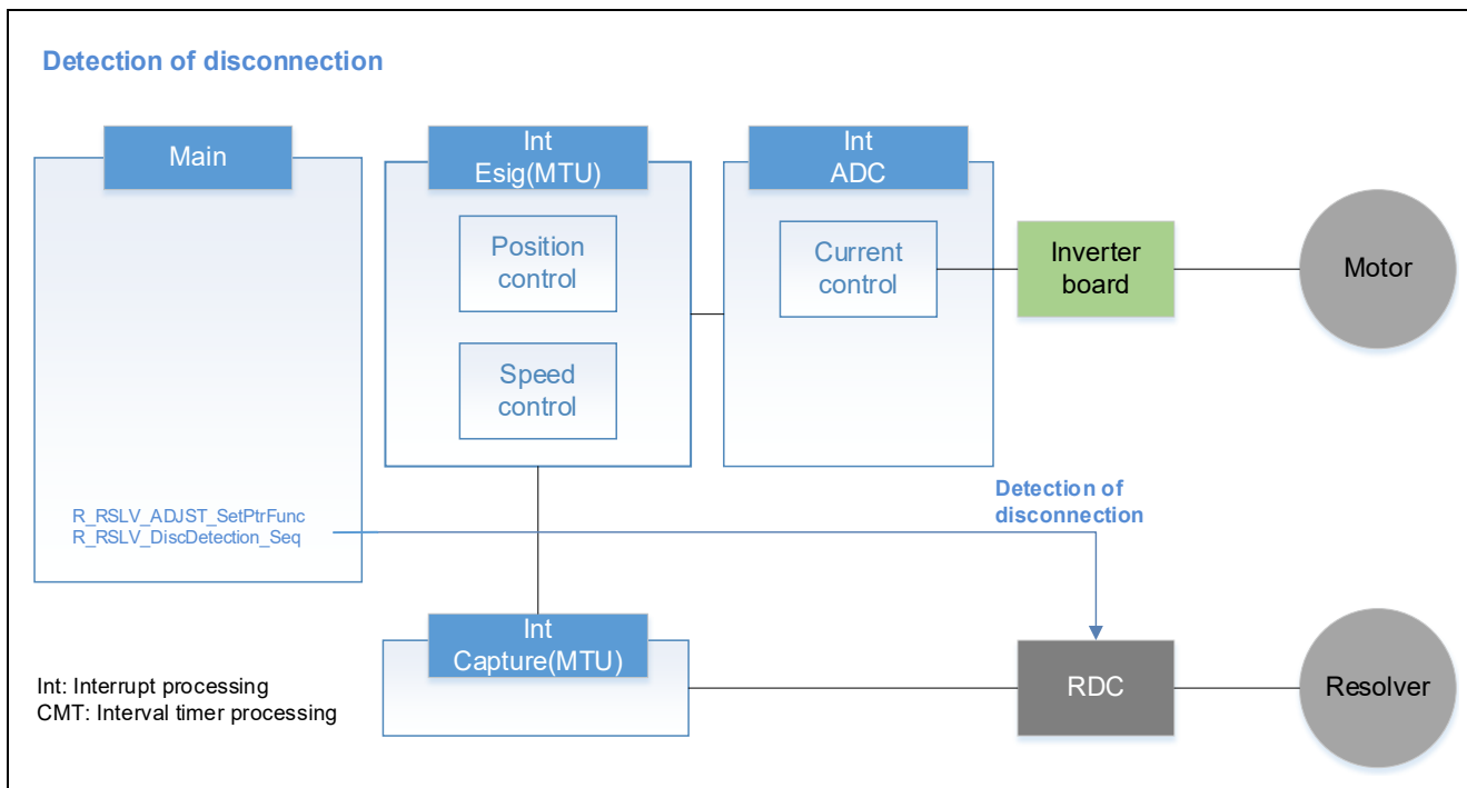
Figure 7.19 Example of Implementing Detection of Disconnection from the Resolver Sensor
