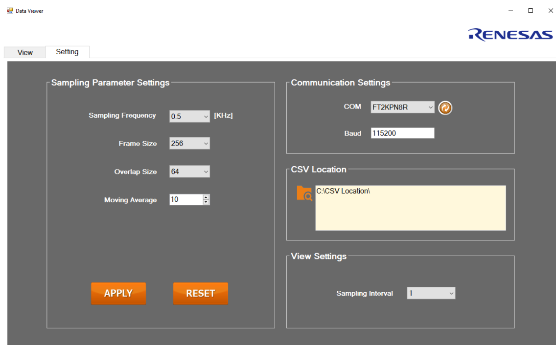
Figure 11 Data Collection Tool parameter settings
