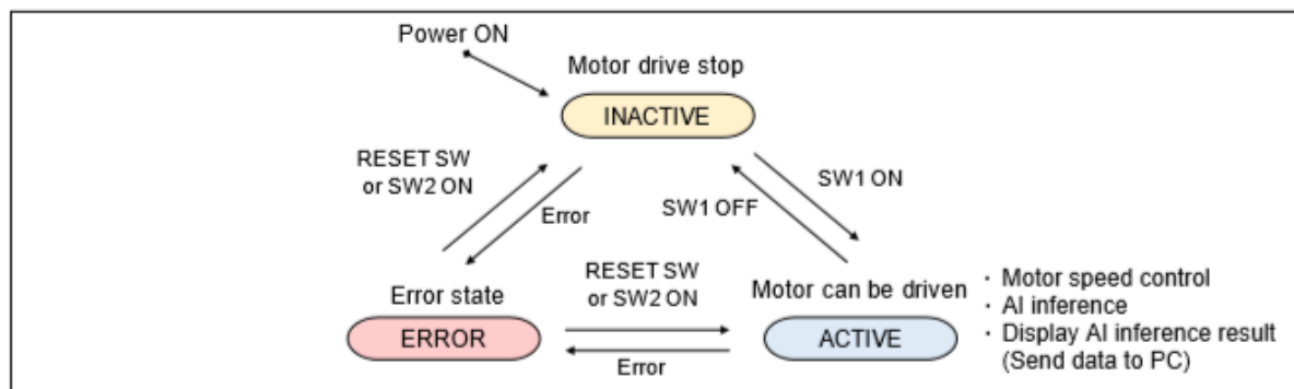
Figure 16. State Transition
