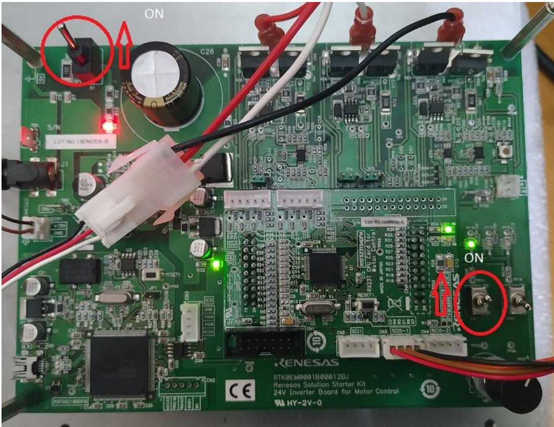
Figure 8 Switch conditions of RX23T
