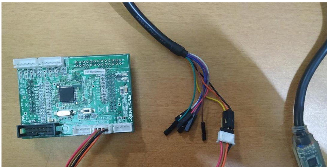
Figure 10 USB-Serial Cable connection to RX23T
