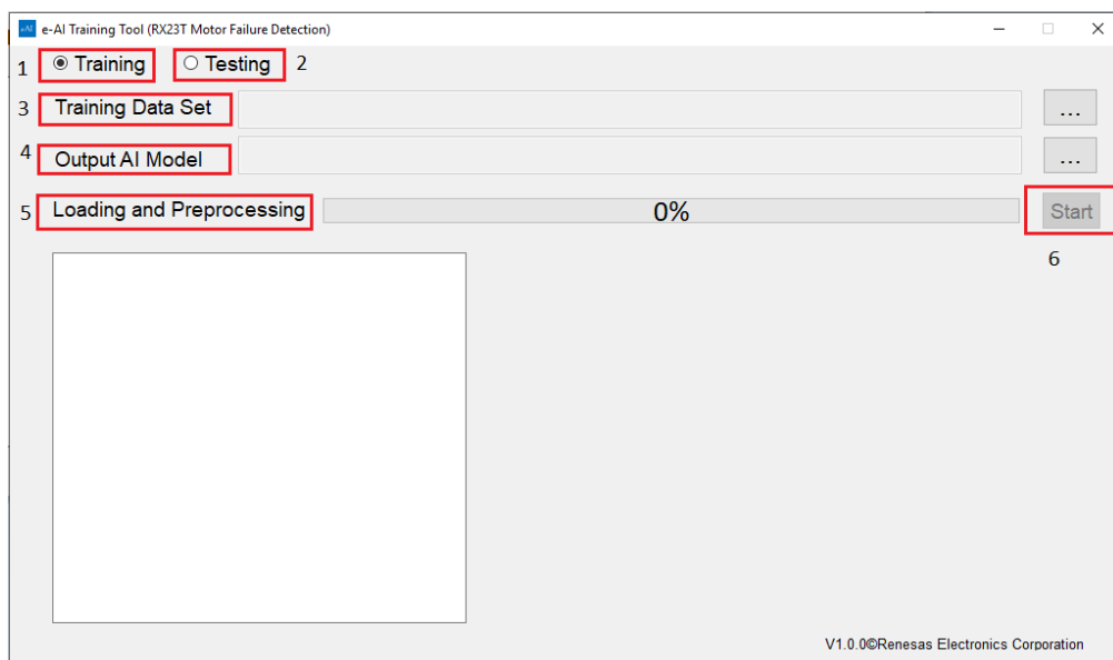
Figure 38 Training tool functionality
