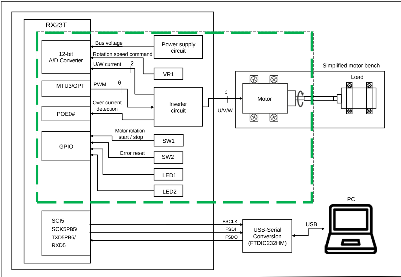
Figure 17 hardware diagram
