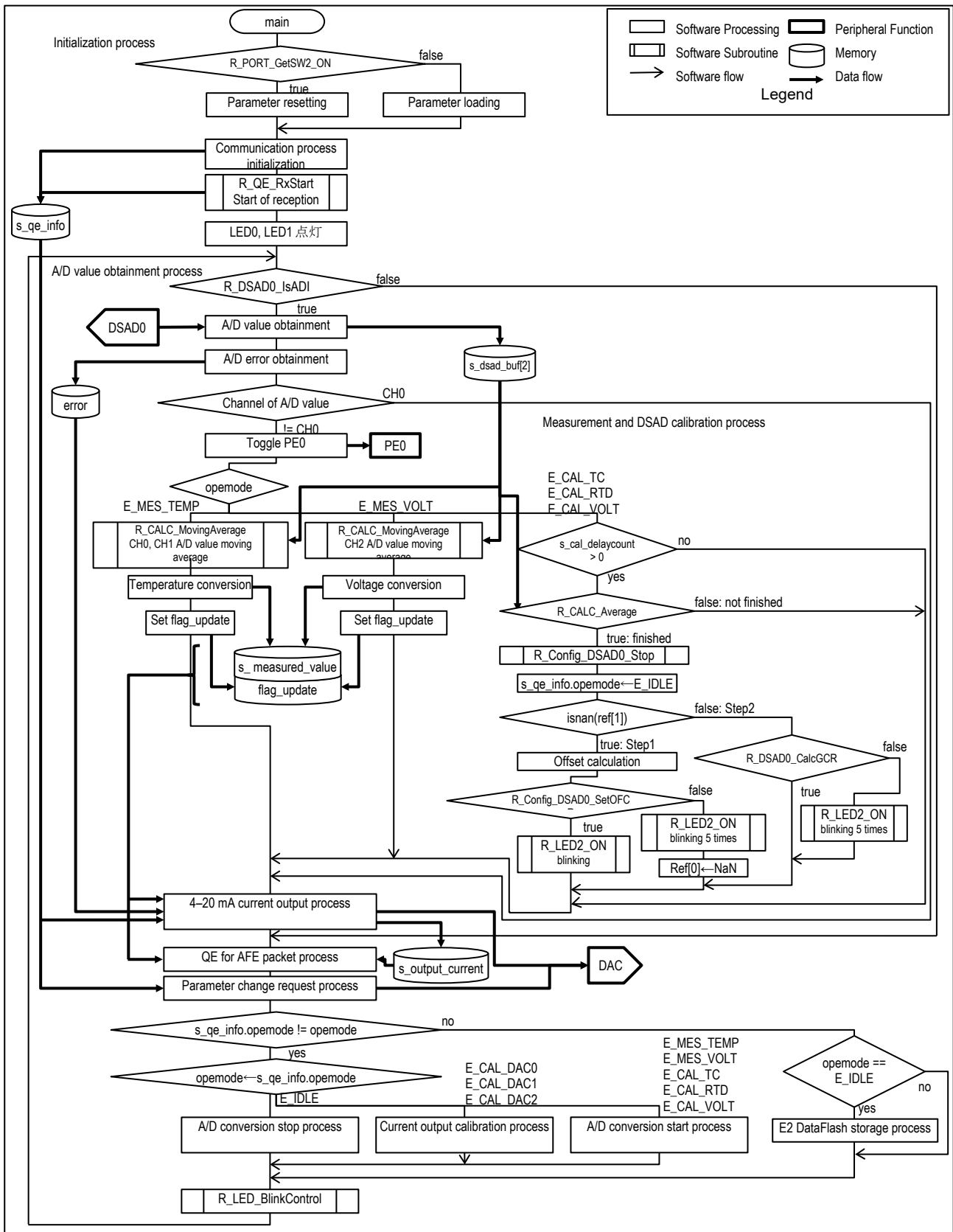
Figure 5-1 General Flow
