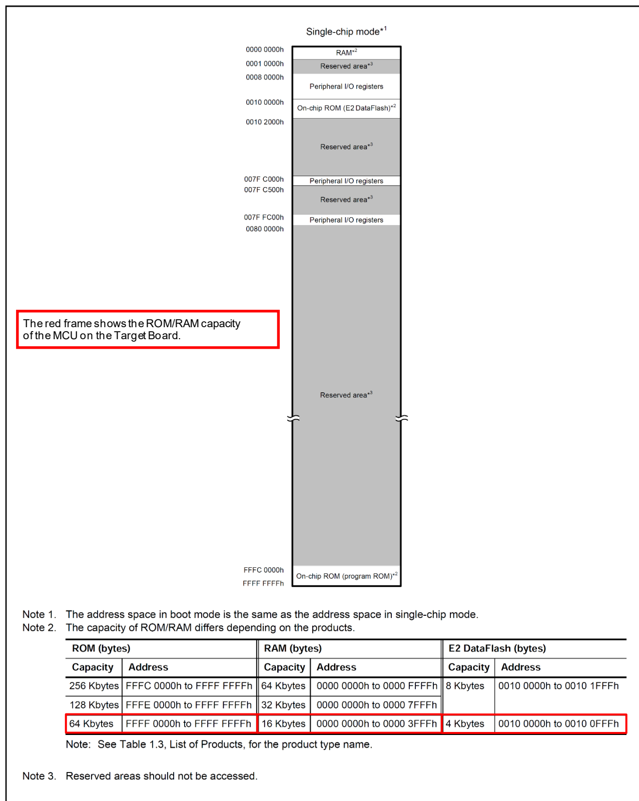
Figure 4-1: RX140 Memory map
