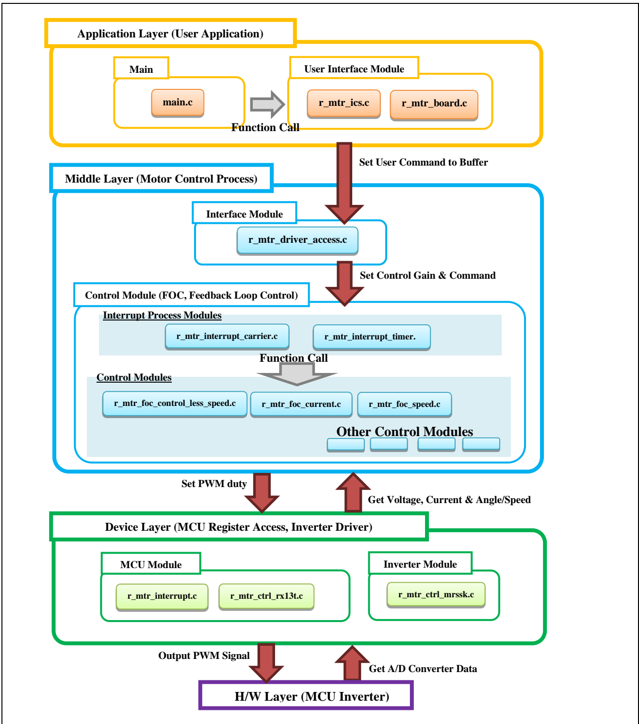
Figure 2-3 Module Configuration
