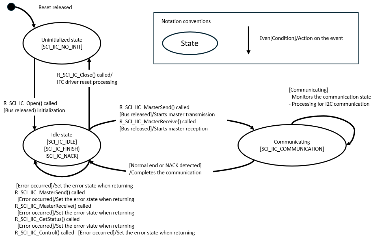
Figure 1.10 State Transition Diagram
