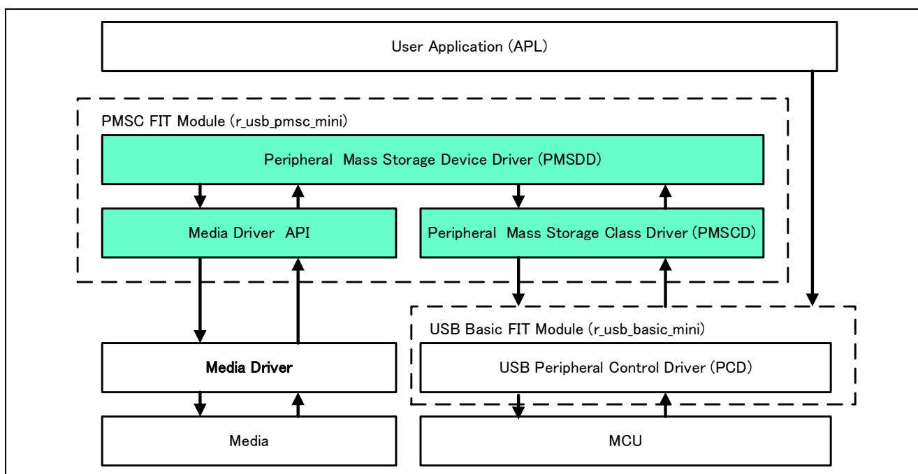
Figure 2-1 Module Configuration
