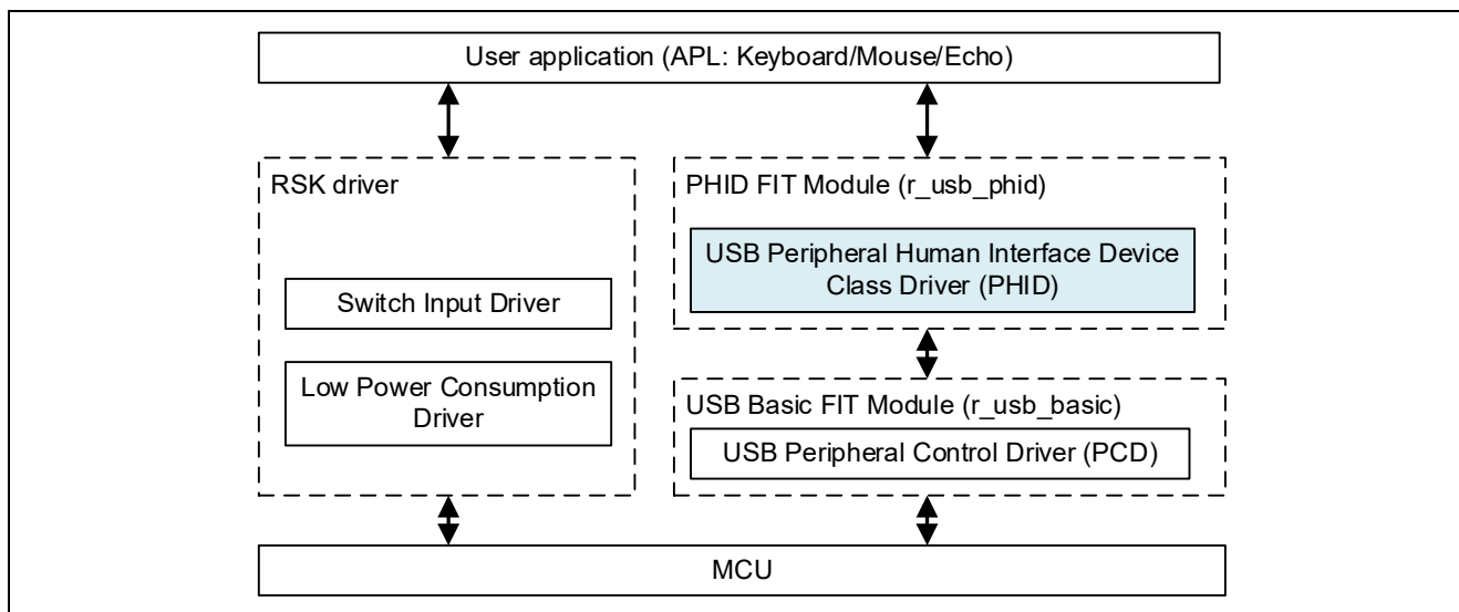
Figure 2-1 Module Configuration
