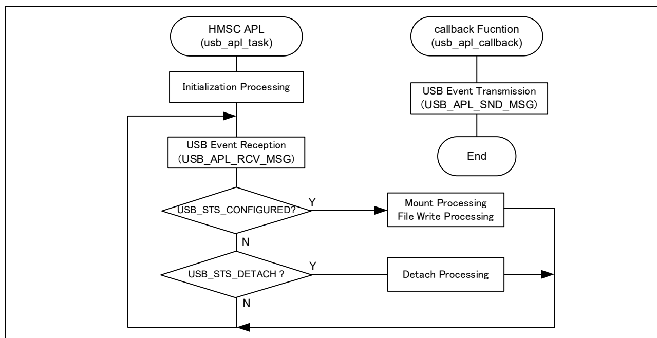
Figure 4-2 usb_apl_task
