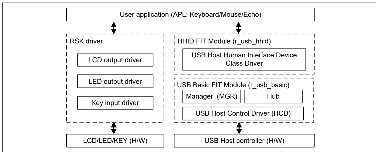
Figure 2-1 Module Configuration
