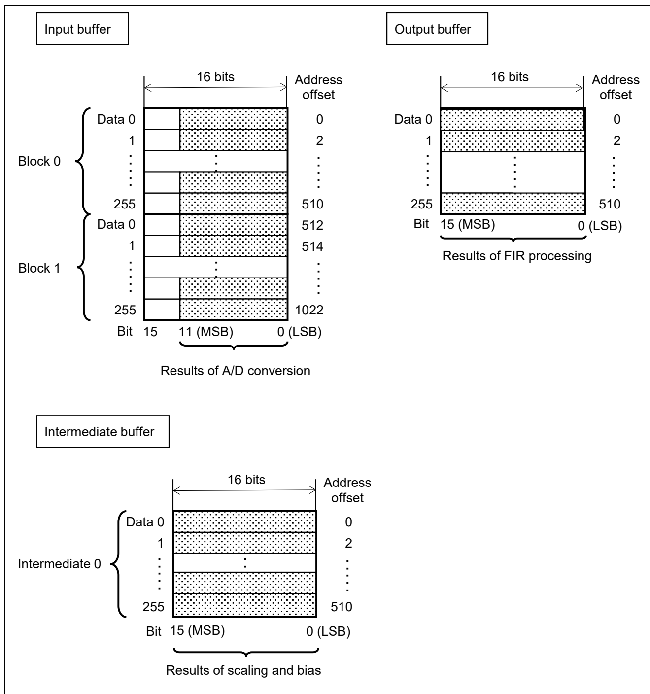
Figure 3.4 Input, Intermediate, and Output Buffers
