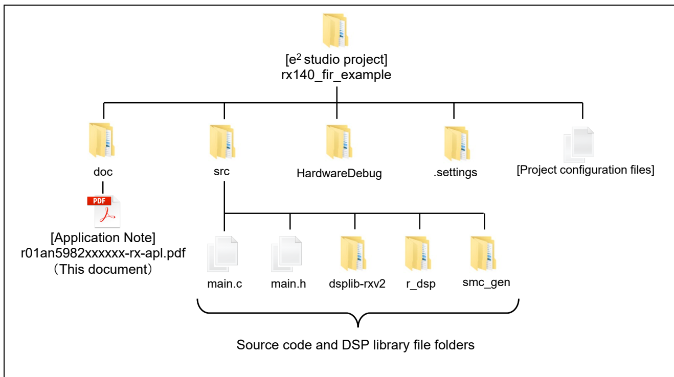
Figure 1.3 Folder Structure of Sample Project
