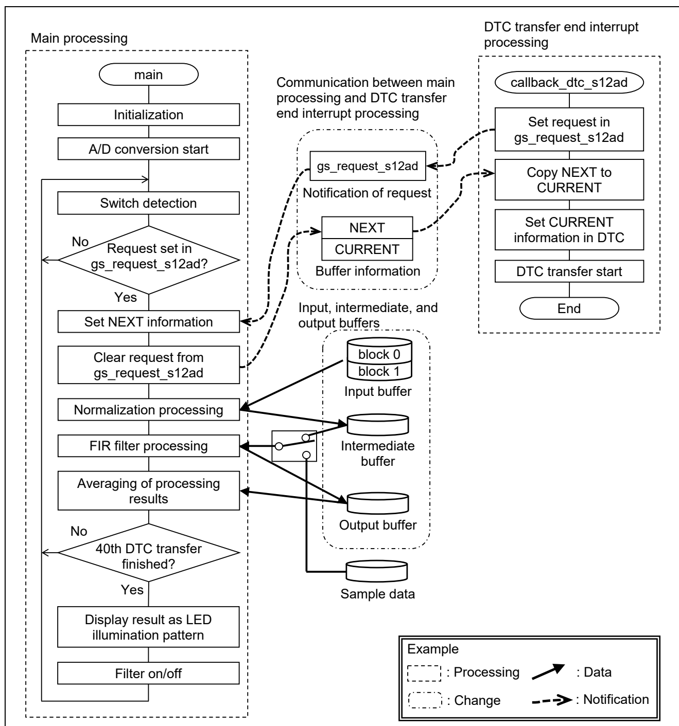
Figure 3.2 Processing Flowchart
