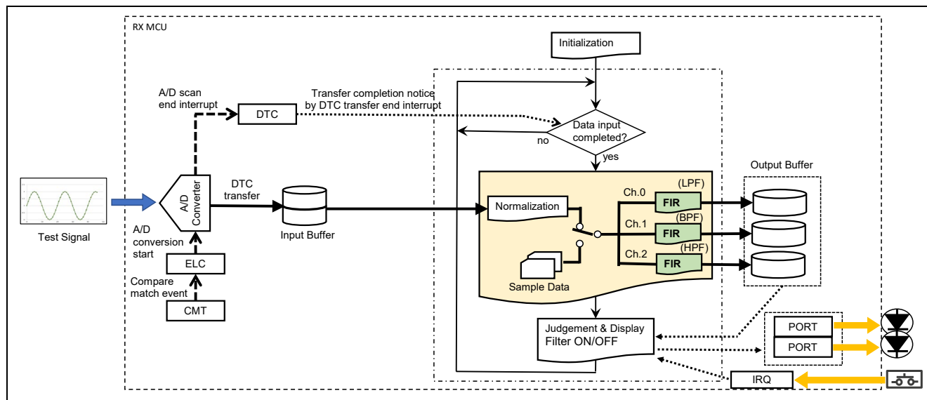
Figure 1.1 System Overview
