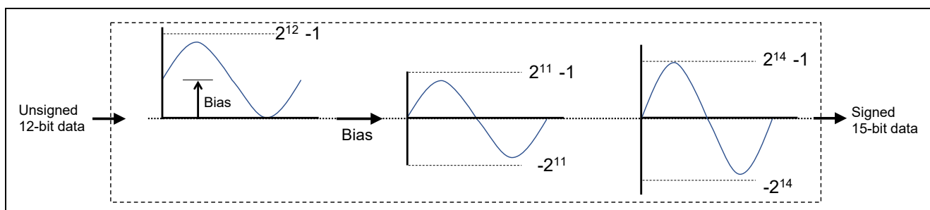
Figure 3.5 Normalization Processing
