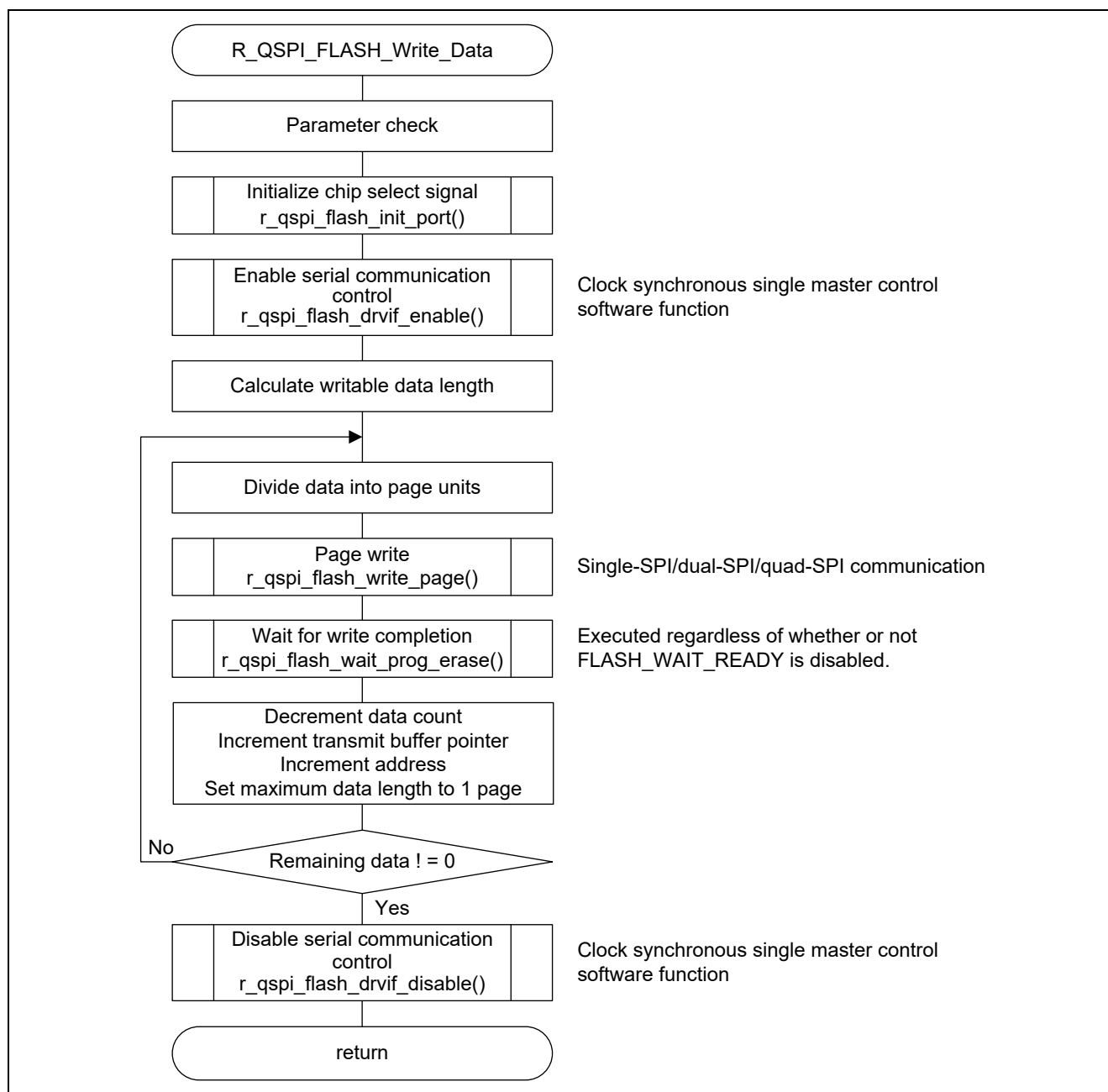
Figure 5.22 Overview of Data Write Processing
