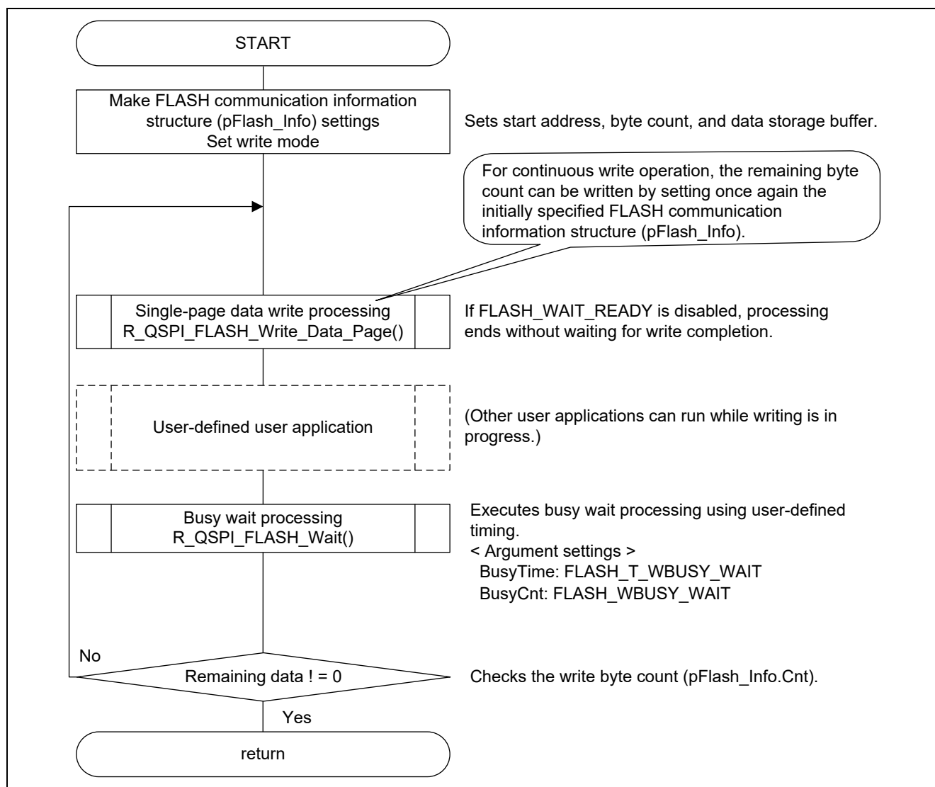
Figure 5.24 Using R_QSPI_FLASH_Wait() to Wait for Data Write Processing (for Single-Page Write) Completion
