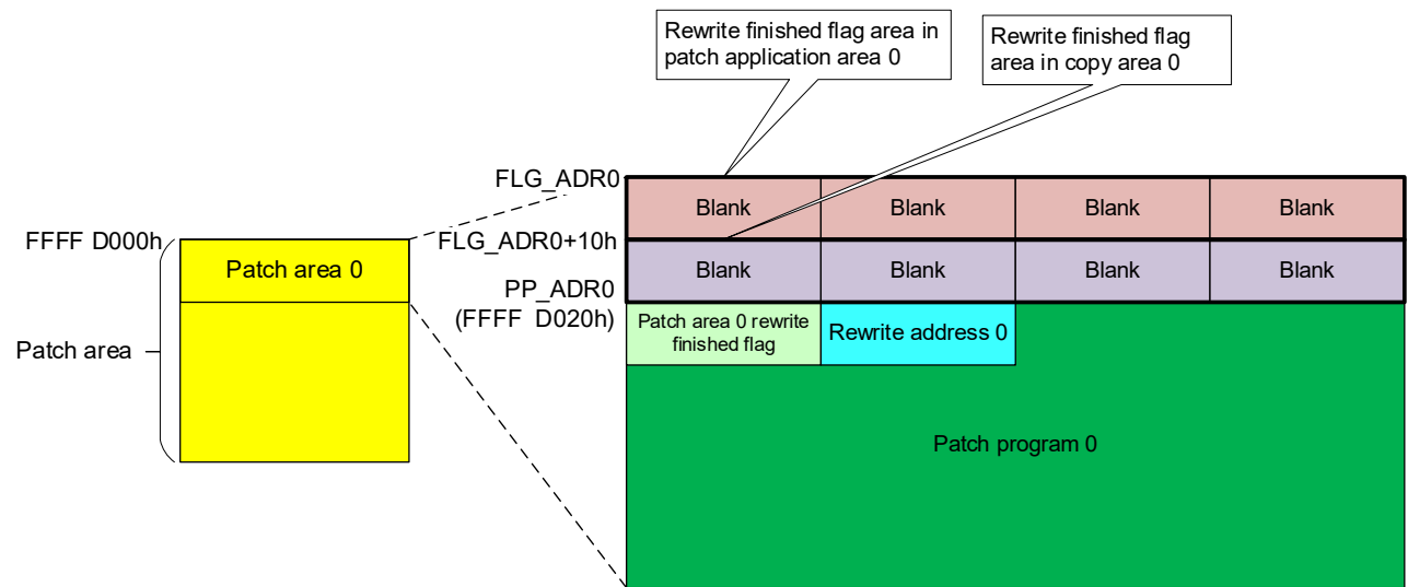
Figure 6.1 Example Patch Area Settings
