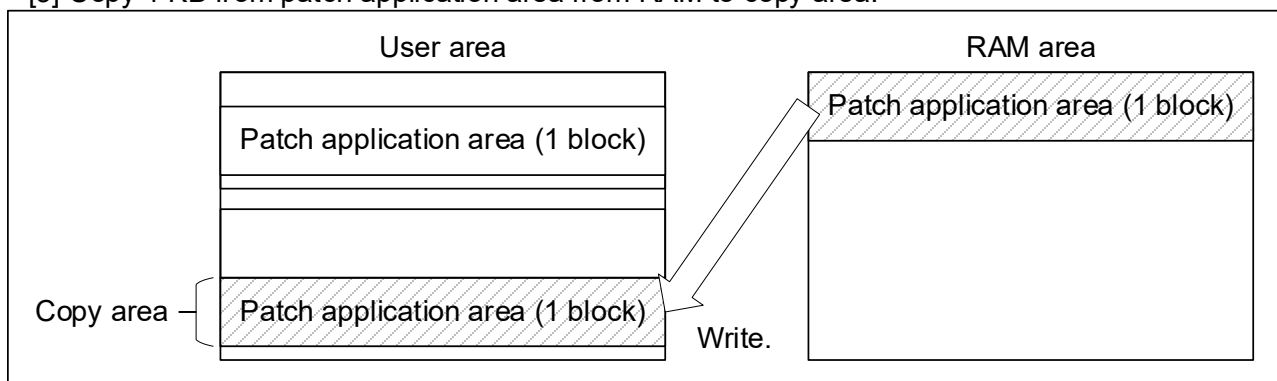
Figure 4.6 Copy Area Rewrite Procedure
