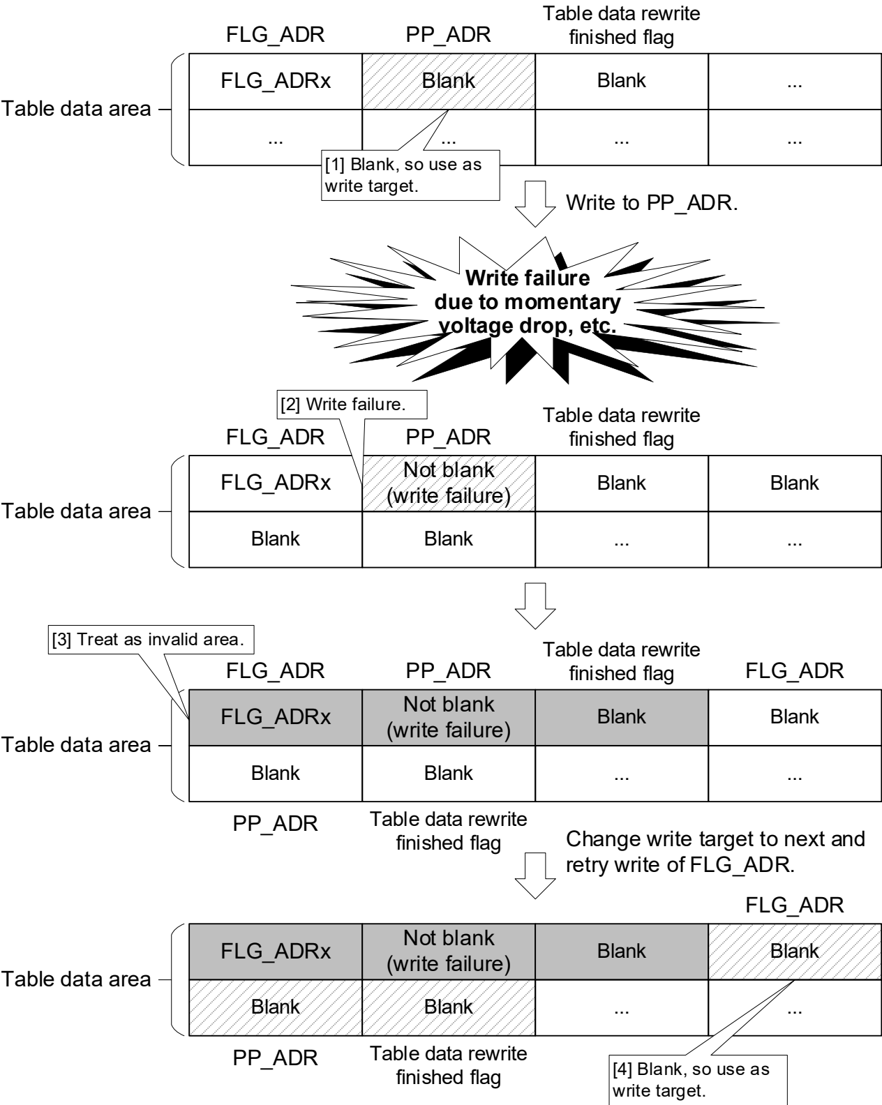
Figure 5.2 Table Data Area Write Procedure Example where Write Failed Due to Momentary Voltage Drop, Etc.
