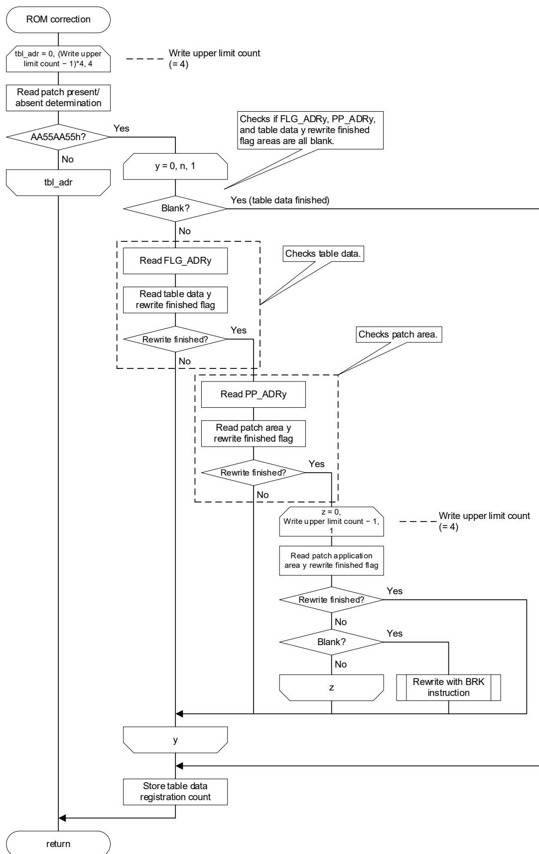
Figure 4.4 ROM Correction Flowchart
