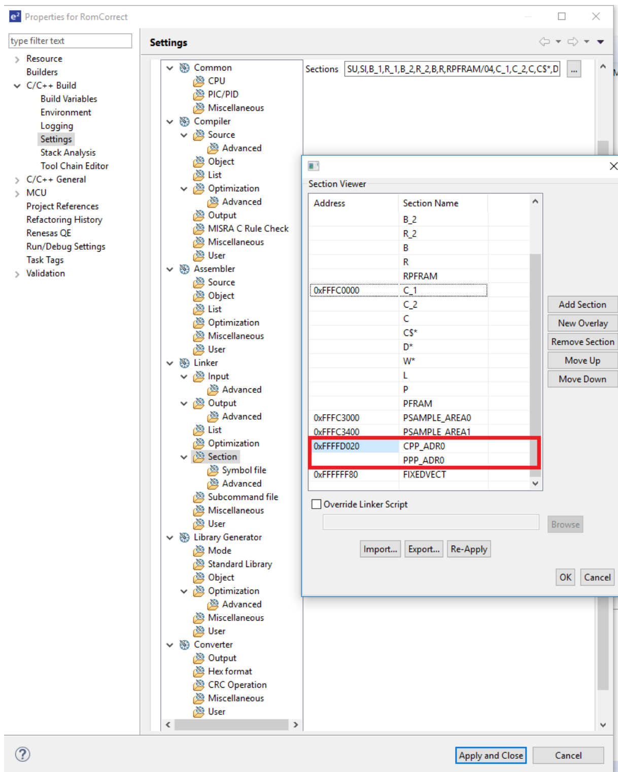
Figure 6.4 Example Section Settings (2/2)
