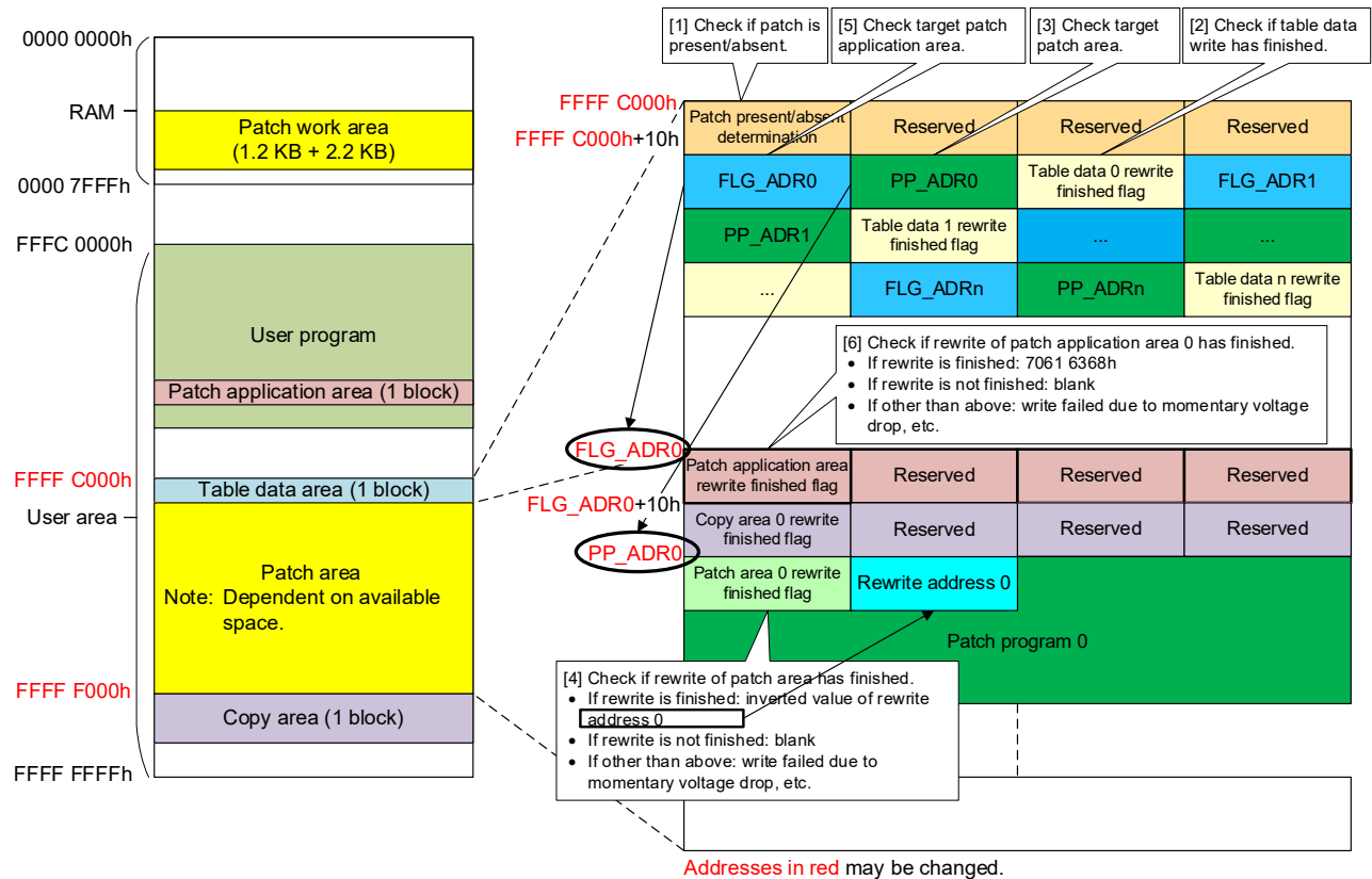
Figure 4.3 Table Data Area and Patch Area Checking
