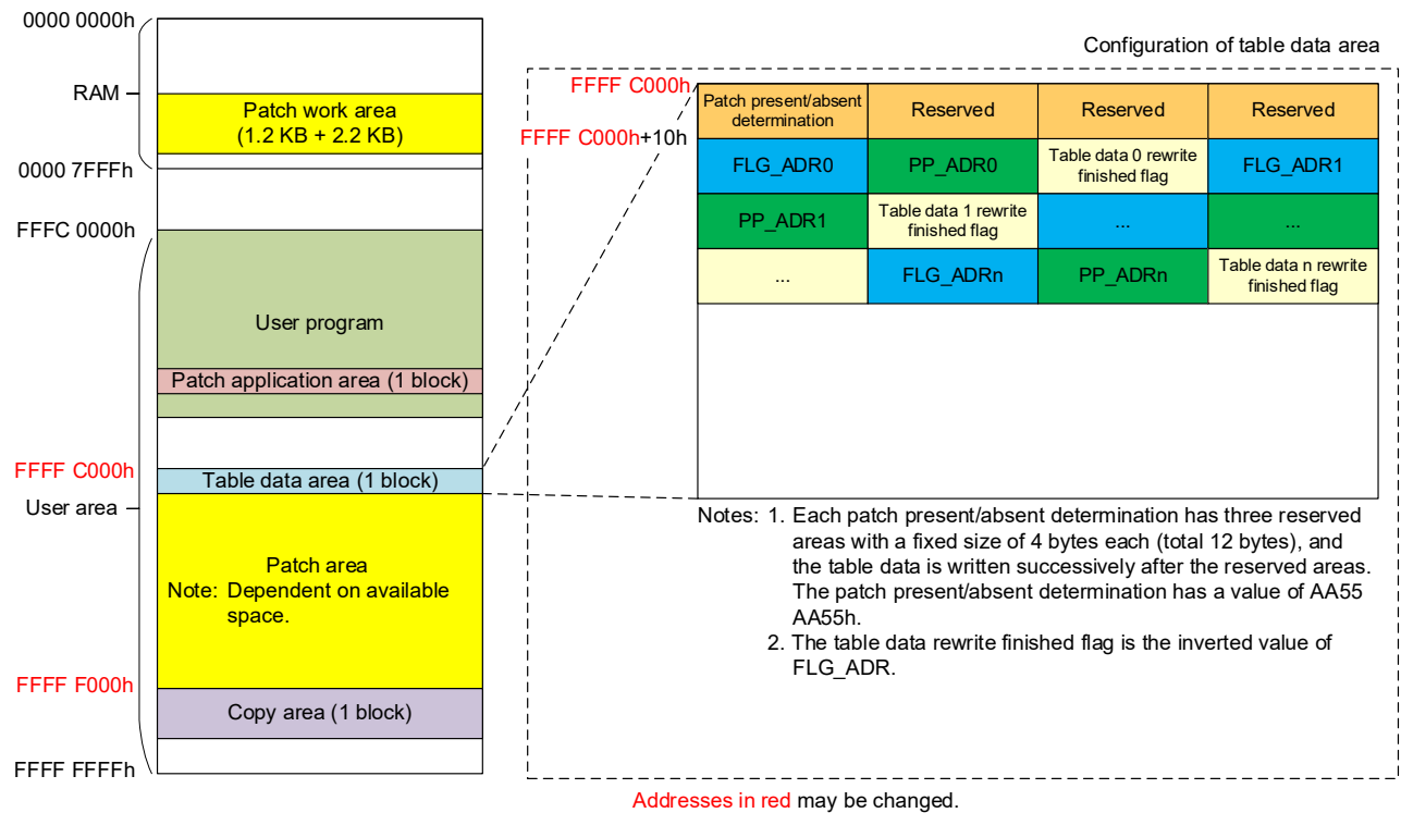
Figure 1.2 Table Data Area
