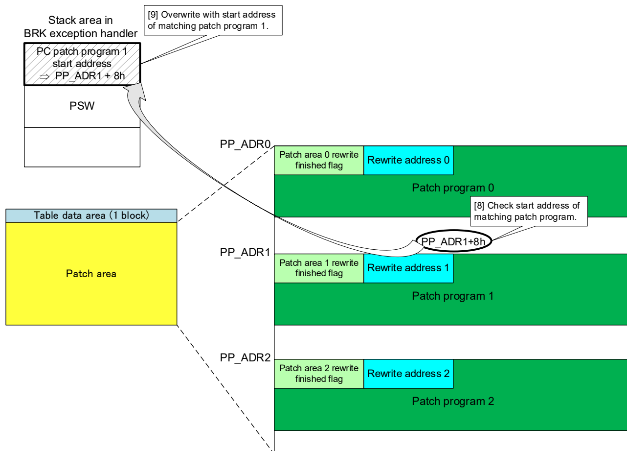
Figure 4.11 Return Setting from BRK Exception Handler
