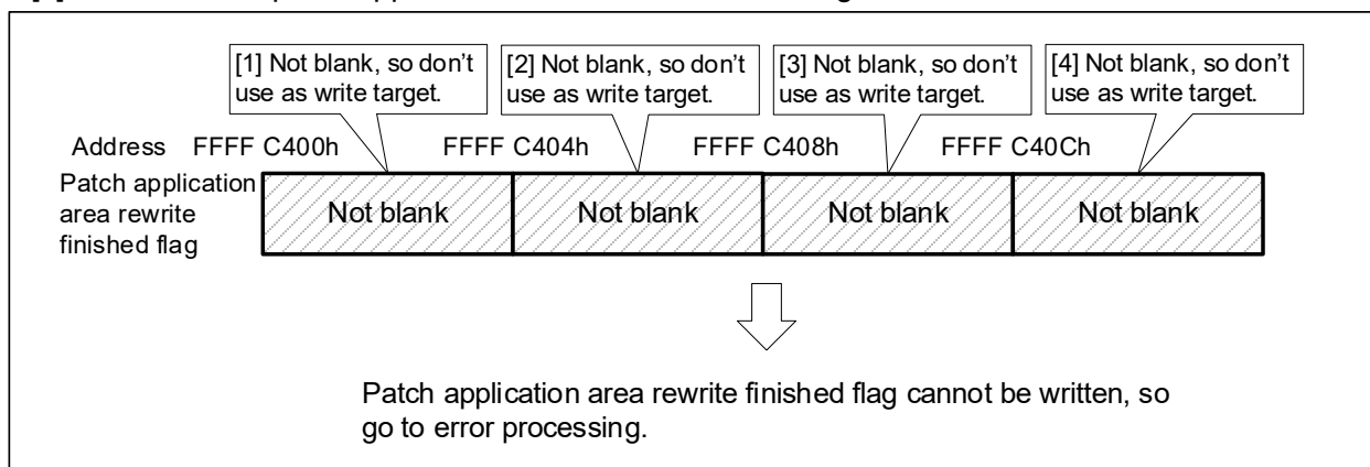
Figure 4.8 Write Procedure with Patch Application Area Rewrite Finished Flag as Example
