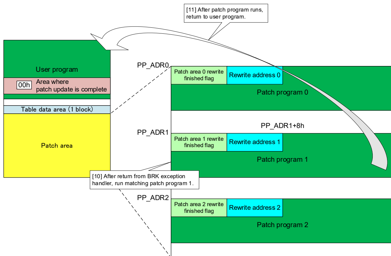
Figure 4.12 Patch Program Execution
