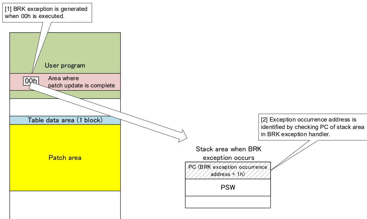
Figure 4.9 Operation when BRK Exception Occurs
