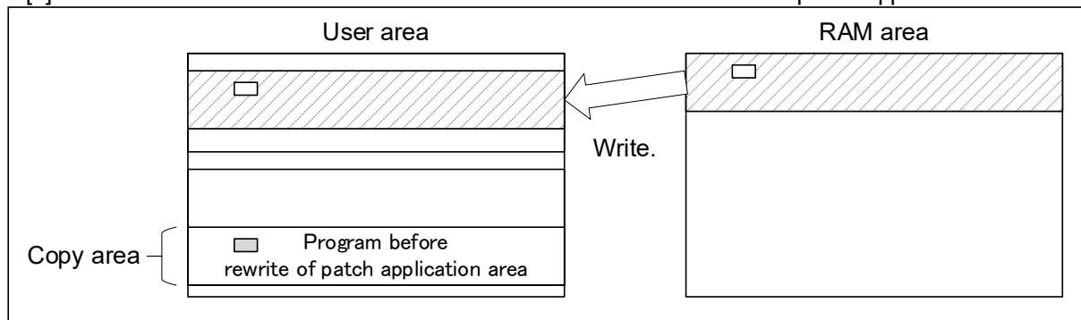
Figure 4.7 Rewrite with BRK Instruction Procedure
