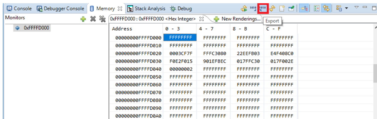
Figure 6.9 Exporting Data from a Memory Area
