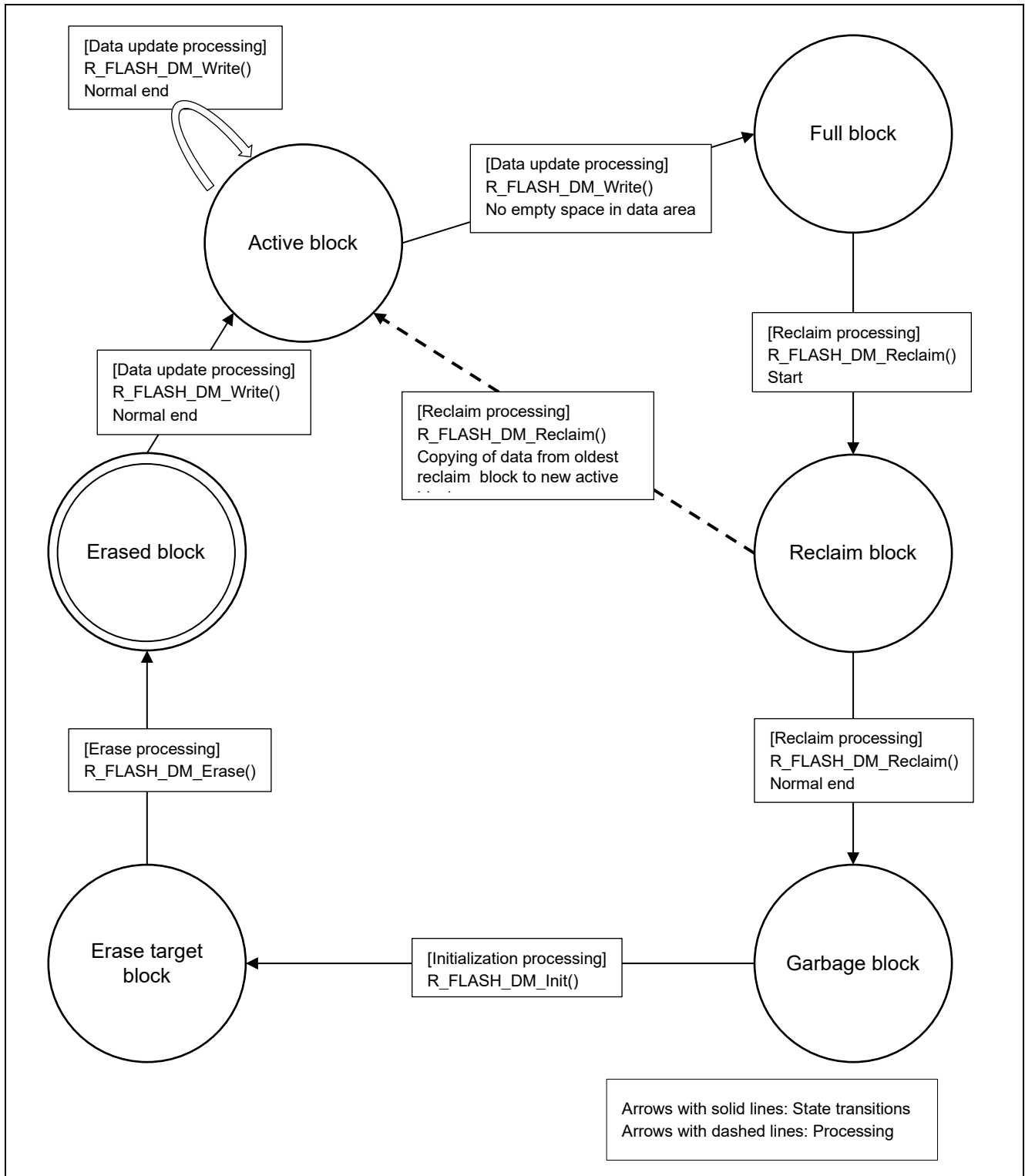
Figure 5.1 Block State Transitions (Flash Type 1)
