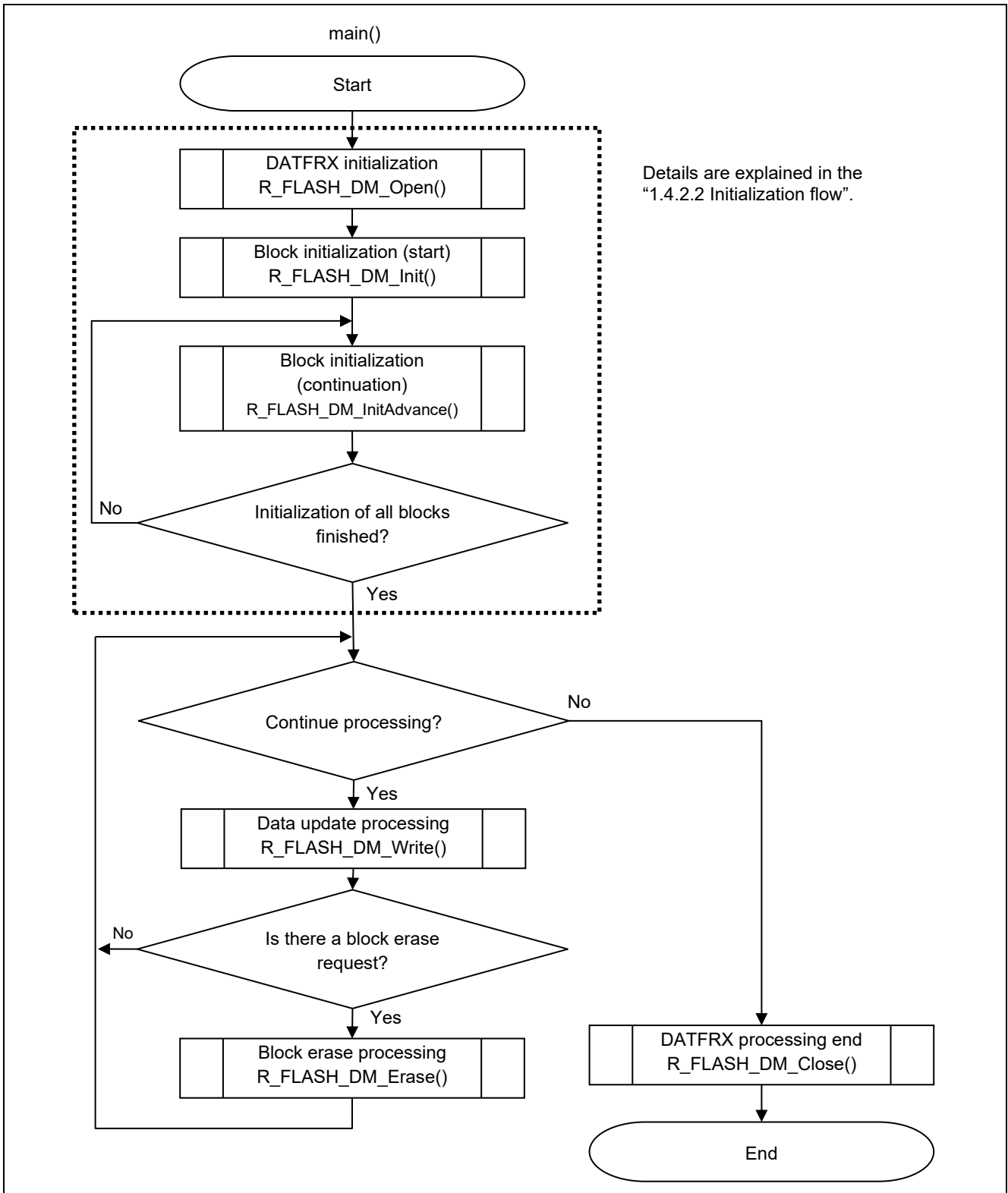
Figure 1.4 Processing Example of Main Function (Flash Type 3, 4 and 5)
