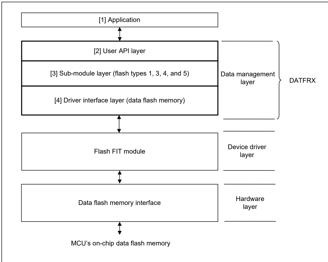
Figure 1.1 Relationship between DATFRX and Flash FIT Module
