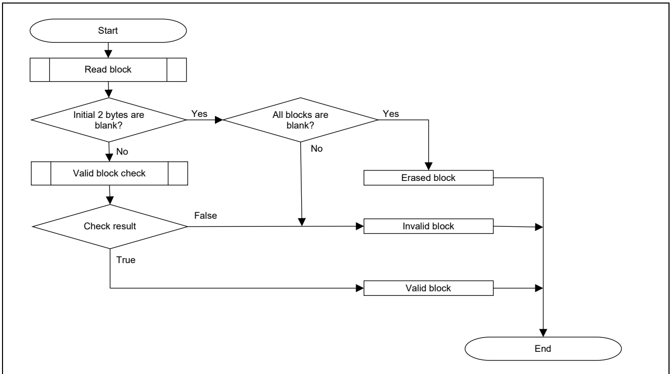
Figure 5.4 Block State Determination Flowchart (Flash Types 3, 4, and 5)
