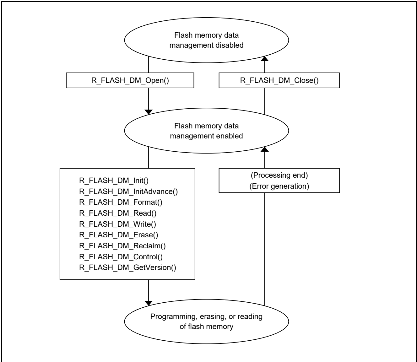
Figure 1.6 State Transition Diagram
