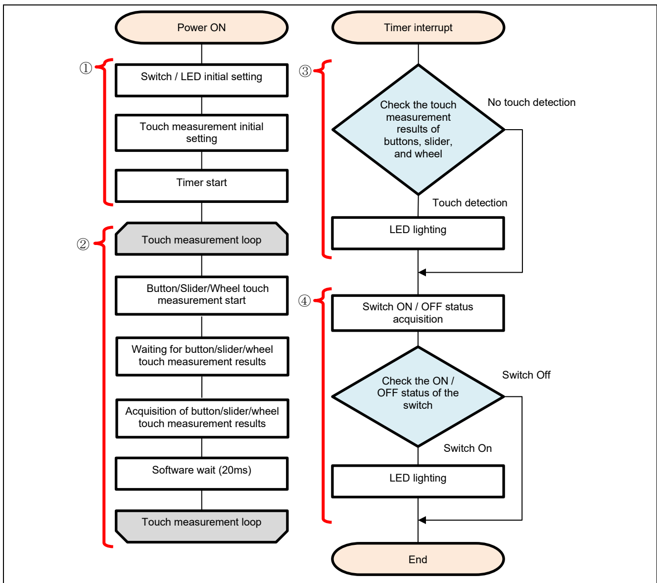
Figure 3-3 Processing Flowchart
