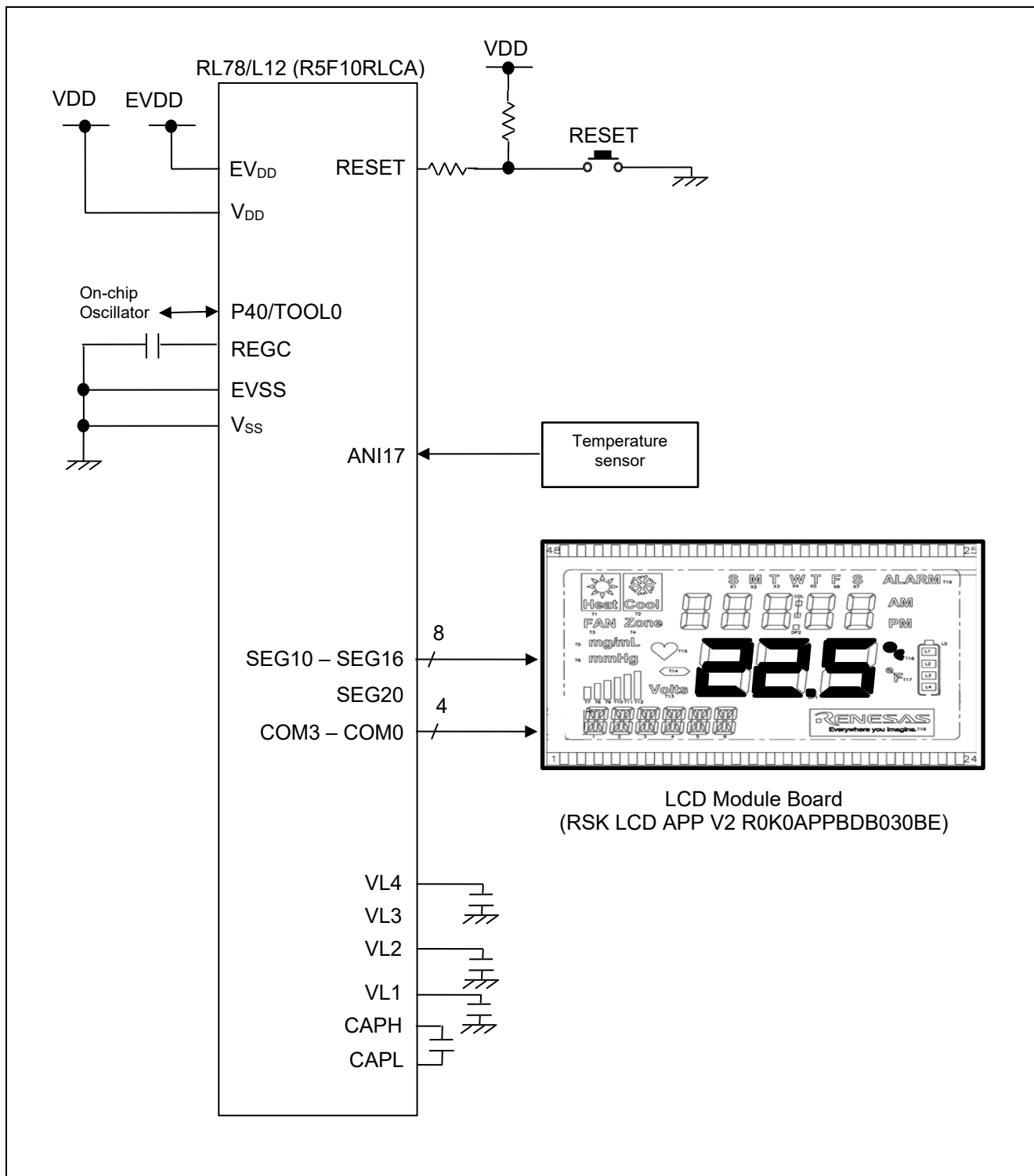
Figure 3.1 Hardware Configuration
