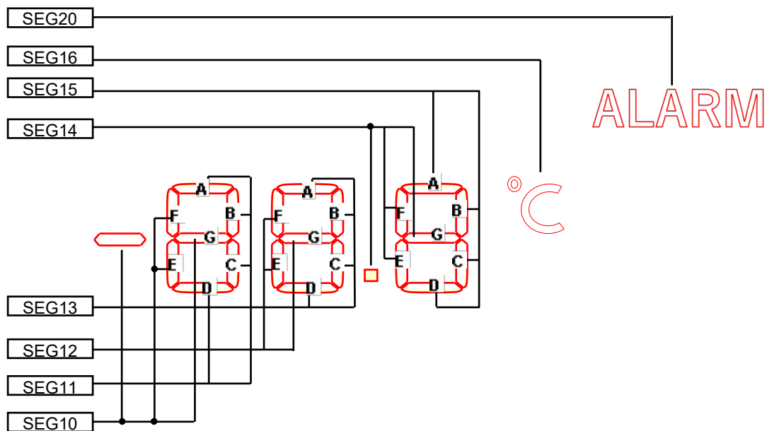
Figure 3.3 shows the connection diagram for symbols and segment (SEG) pins.
