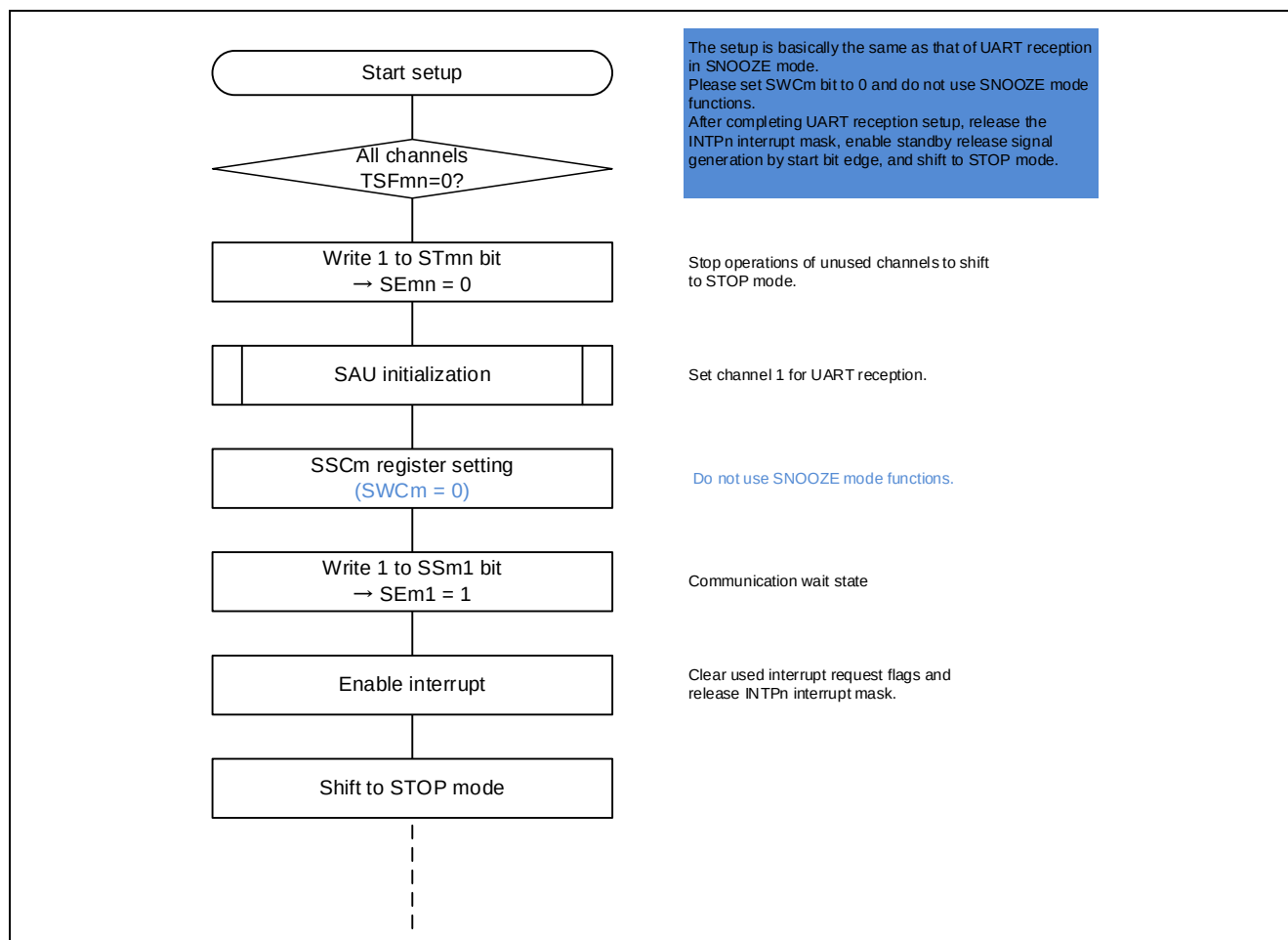
Figure 5.6 How to Receive UART Data in STOP Mode
