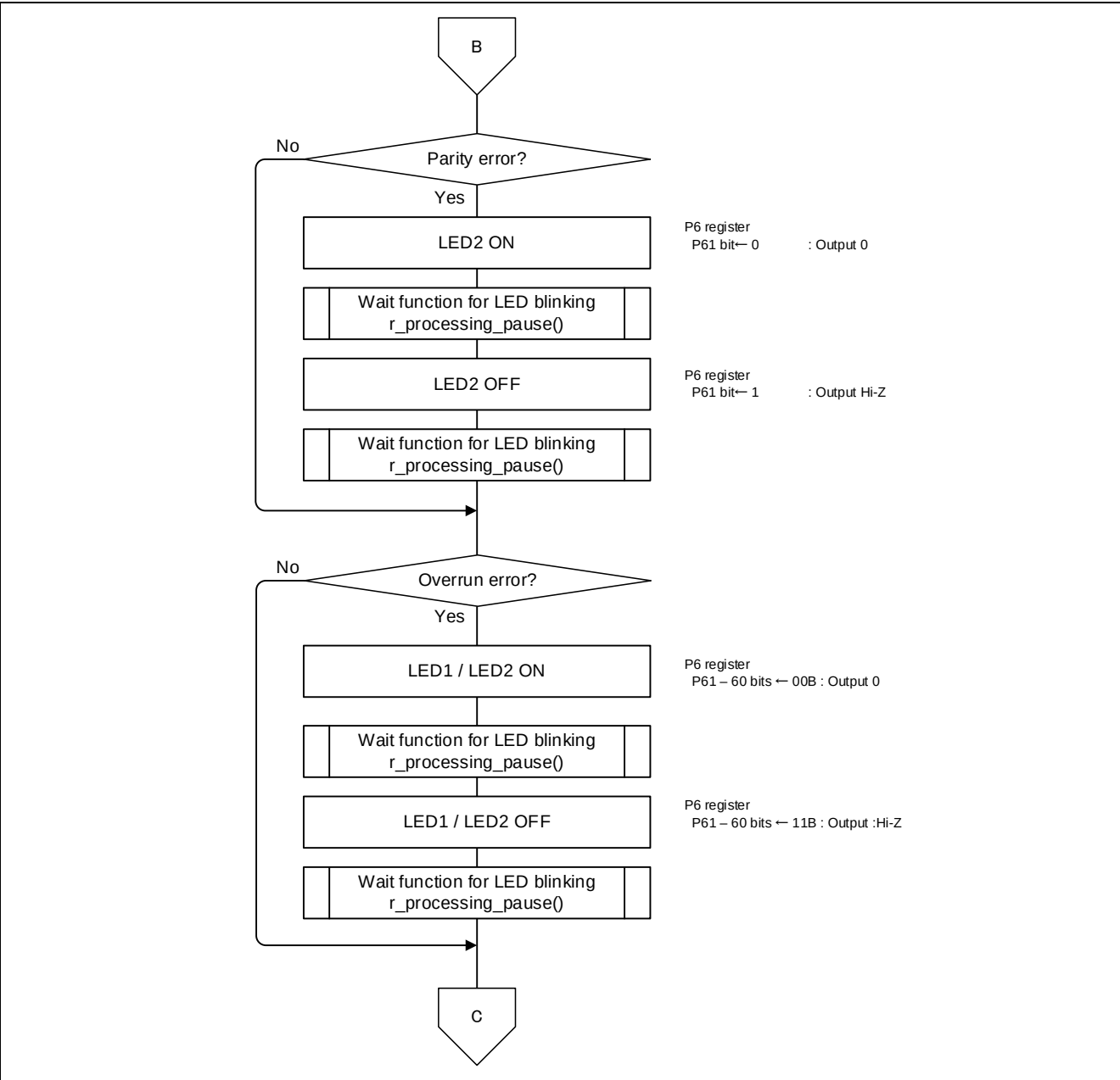
Figure 5.18 Main Processing (2/2)
