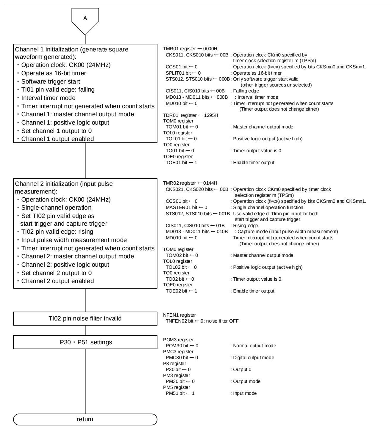
Figure 5.13 TAU0 Initialization (2/2)
