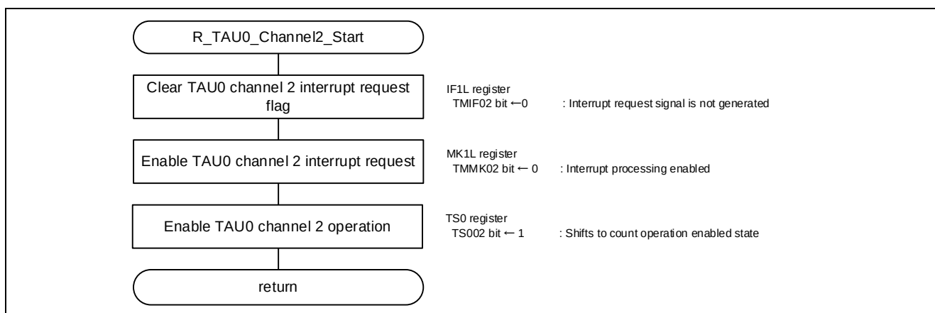
Figure 5.25 TAU0 Channel 2 Operation Start Function
