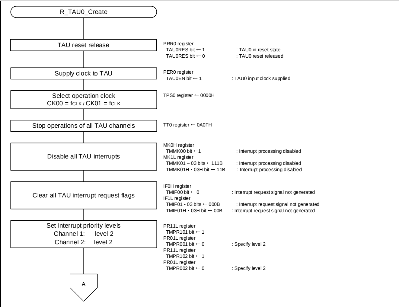
Figure 5.12 TAU0 Initialization (1/2)
