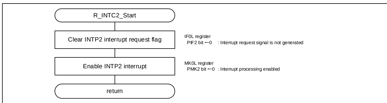
Figure 5.24 INTP2 Operation Start Function
