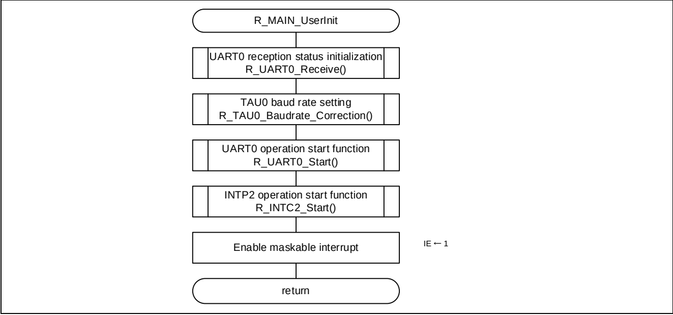
Figure 5.19 Main Initialization
