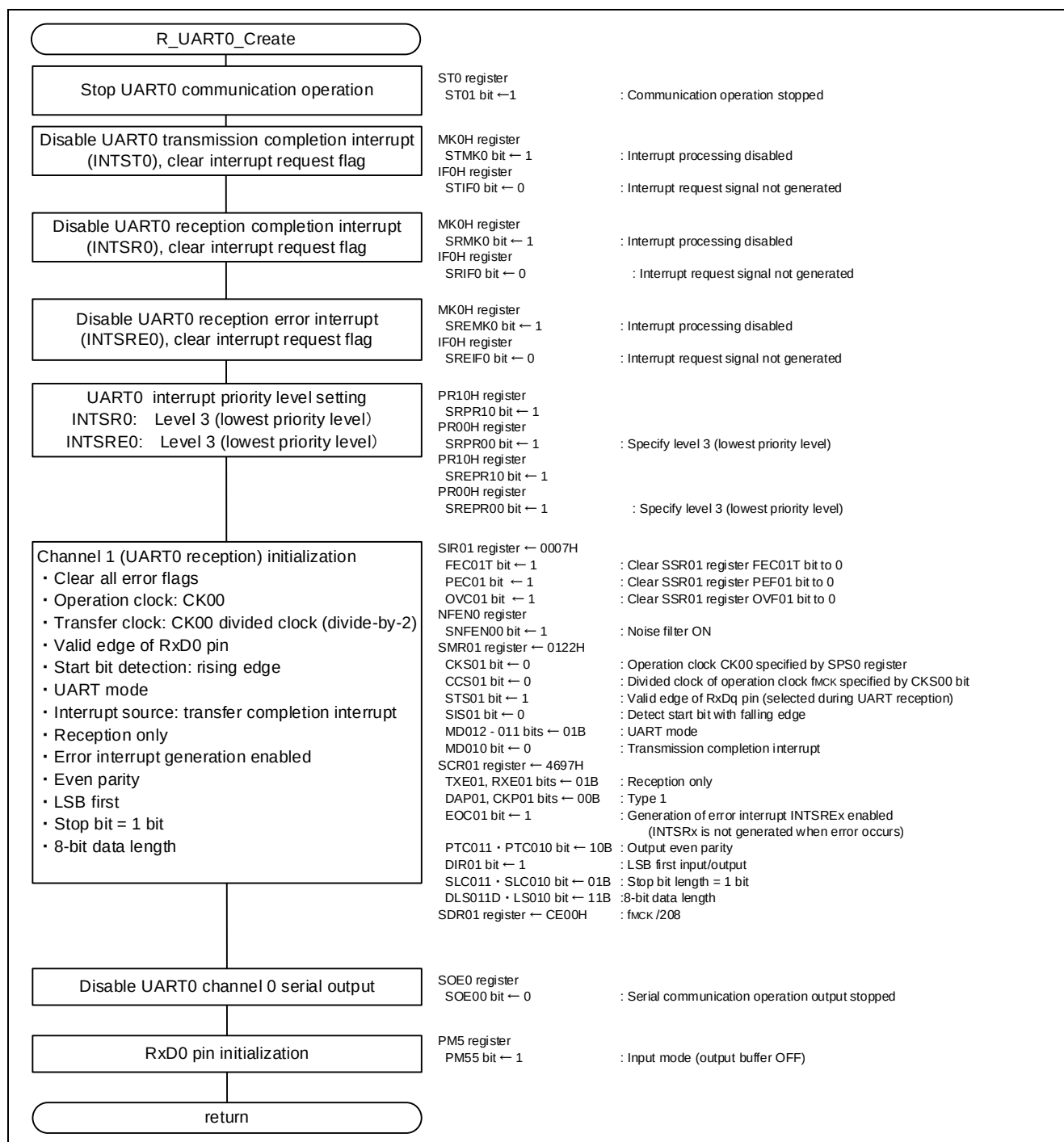
Figure 5.15 UART0 Initialization
