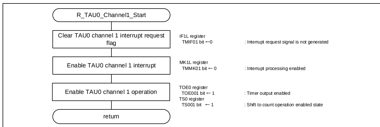
Figure 5.26 TAU0 Channel 1 Operation Start Function
