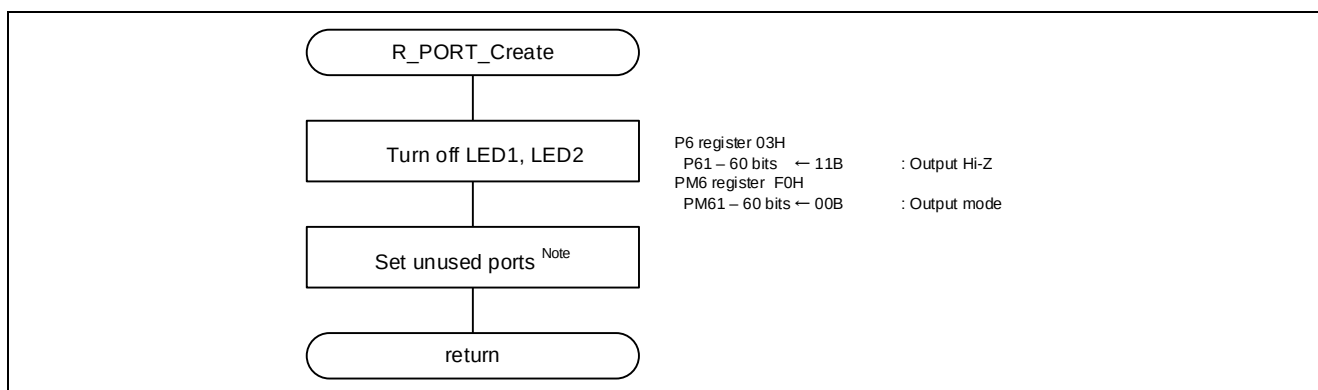
Figure 5.10 Port Initialization
