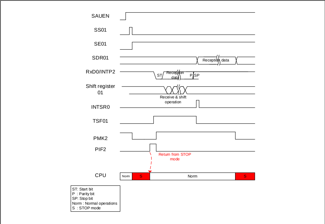
Figure 5.3 Timing Chart
