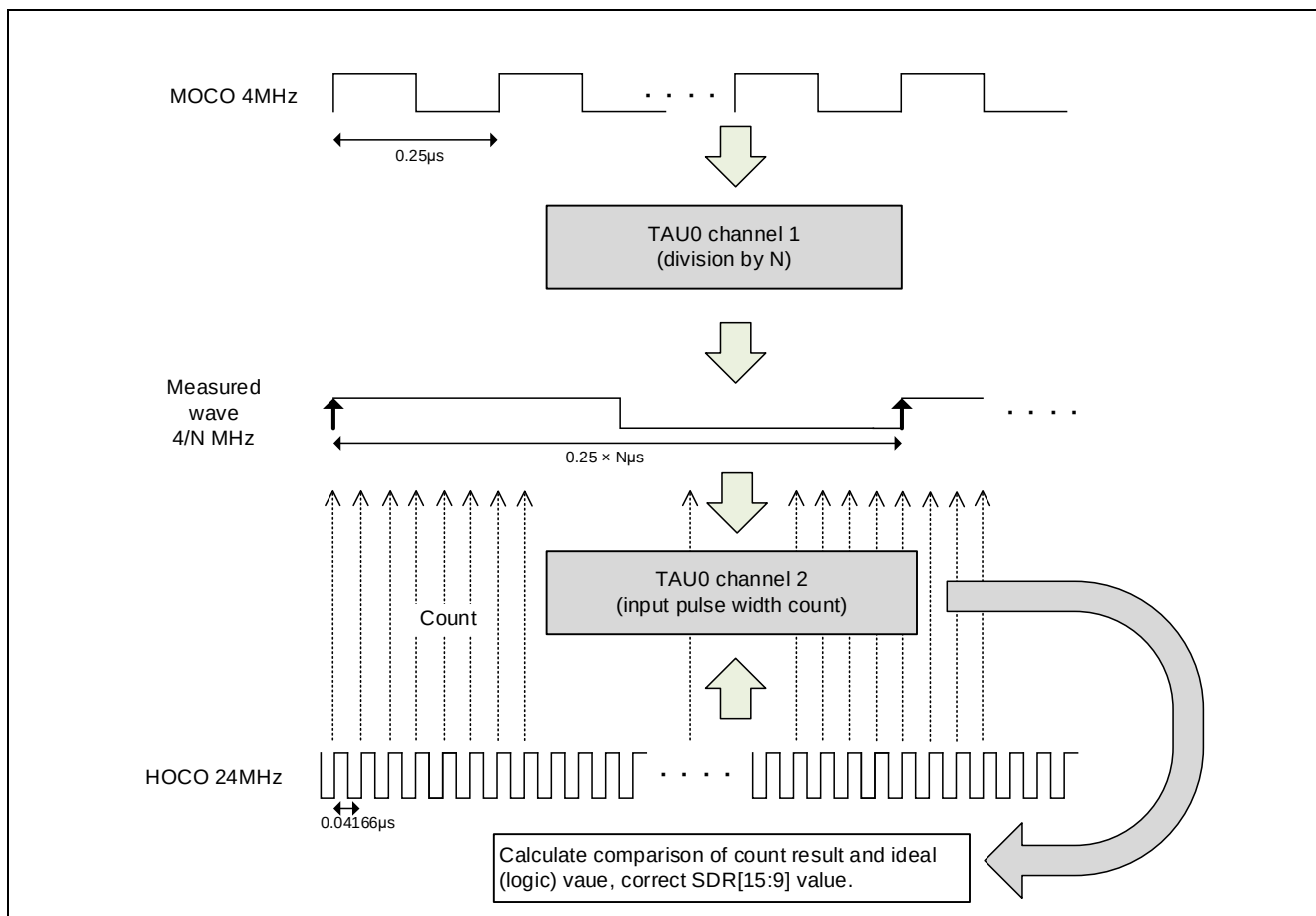
Figure 5.4 Correction Processing
