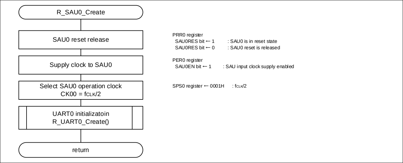
Figure 5.14 SAU0 Initialization
