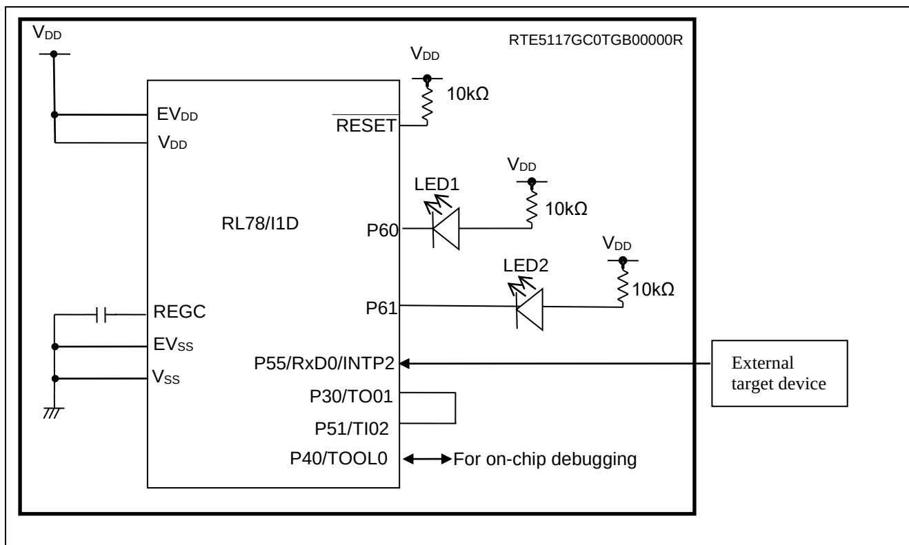
Figure 4.1 Hardware Configuration
