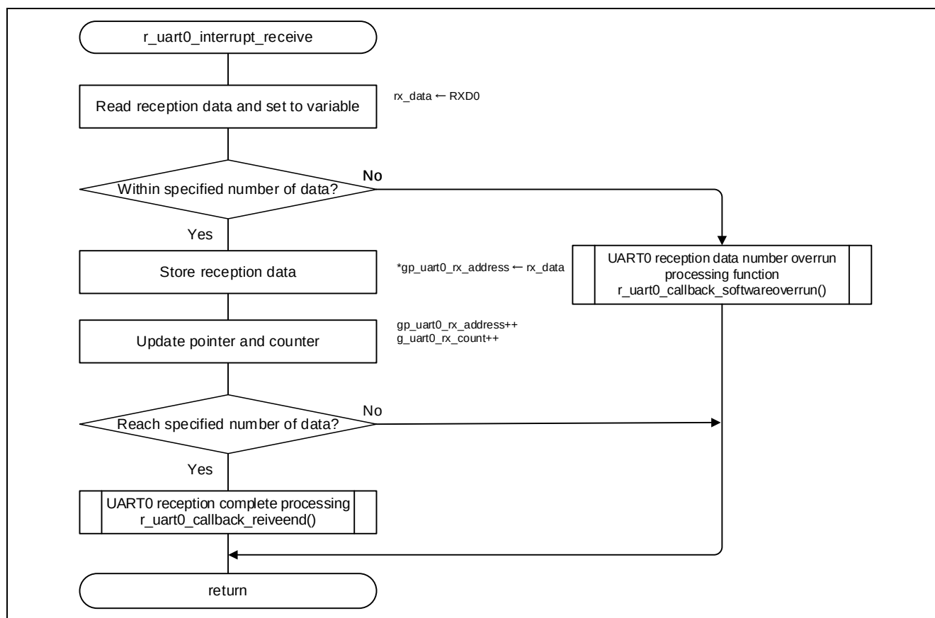
Figure 5.32 UART0 Reception Complete Interrupt Processing
