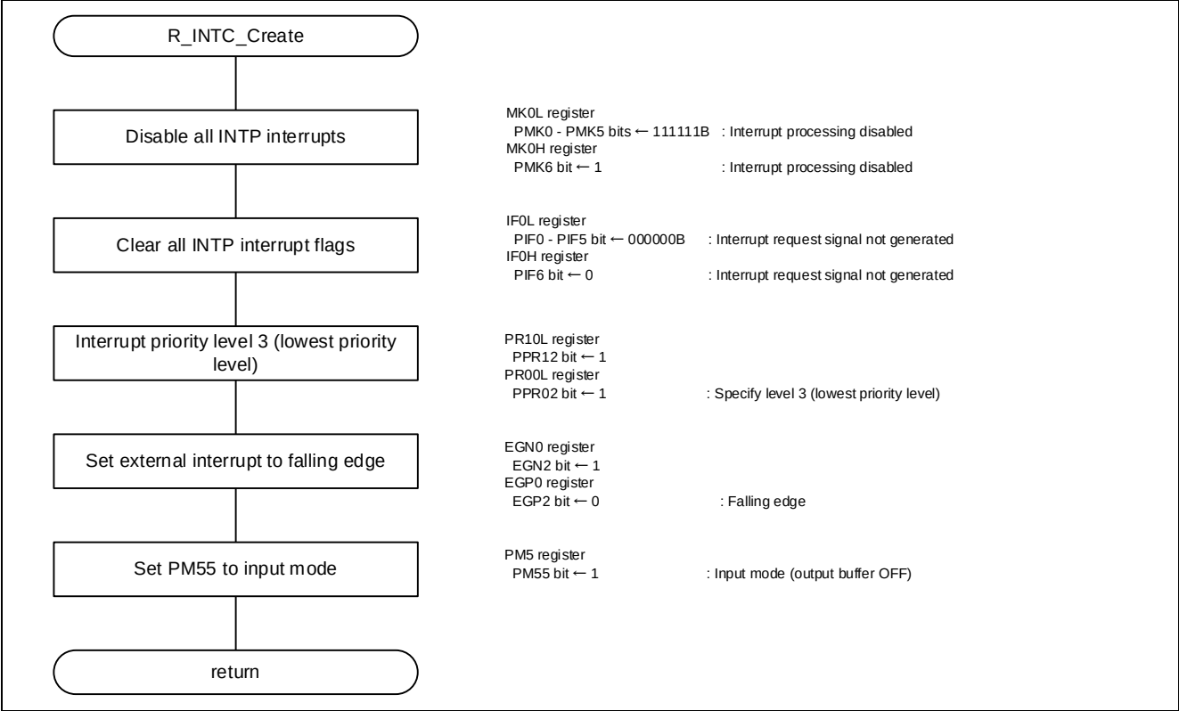
Figure 5.16 INTP Initialization
