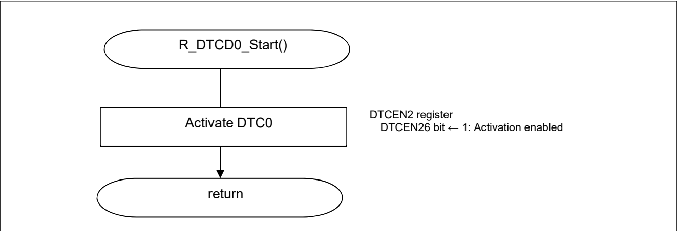
Figure 5.17 DTC0 Activation
