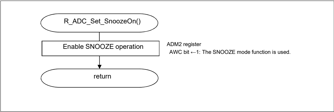
Figure 5.20 A/D Converter’s SNOOZE Function Start
