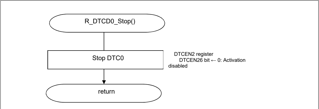
Figure 5.28 DTC0 Stop
