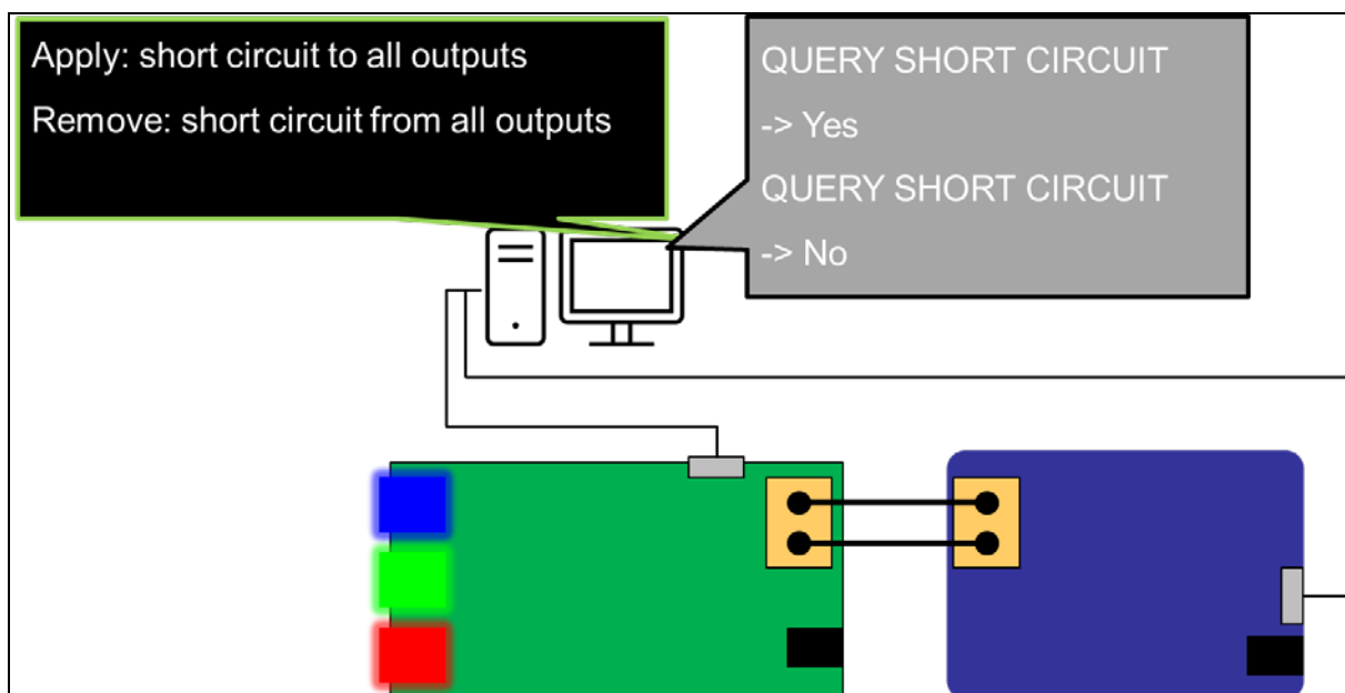
Figure 1-1 102ed.2.0+207ed.1.0 Sample Application Operation Schematic
