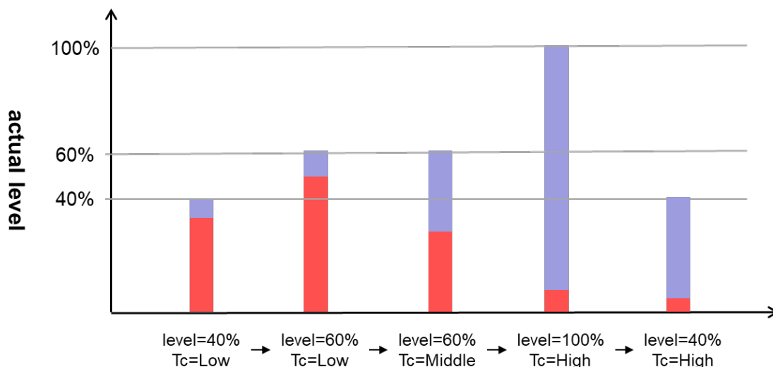
Figure 4-10 Ratio of the total dimming ratio (actual level) to the dimming ratio of each temperature range LED
