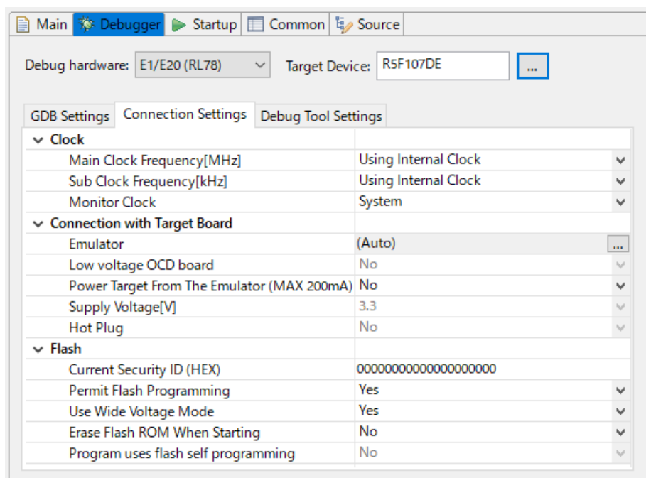
Figure 4-5 Debug screen setting contents
