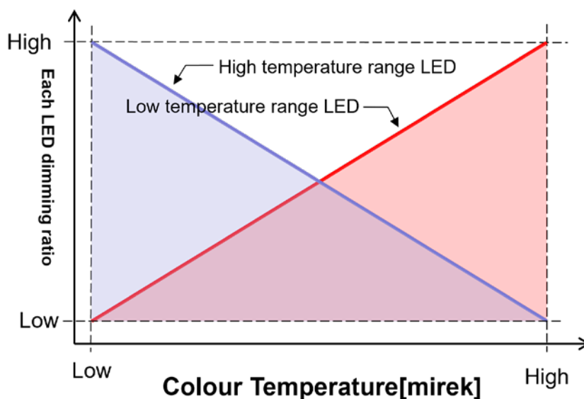
Figure 4-8 Relationship between color temperature and each temperature range LED
