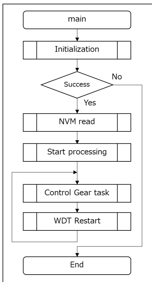
Figure 4-13 Main flow diagram
