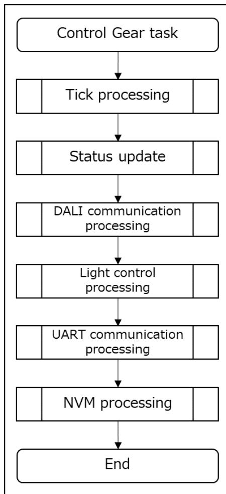
Figure 4-17 Control Gear task processing flow diagram
