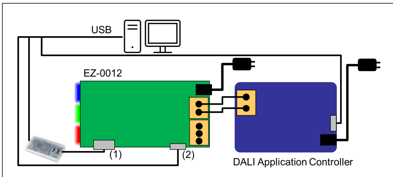
Figure 4-4 Connection diagram when using EZ-0012 only
