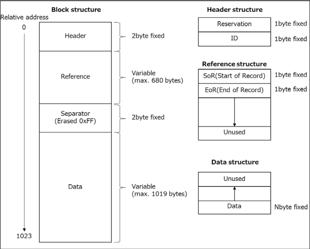
Figure 4-7 Block structure diagram
