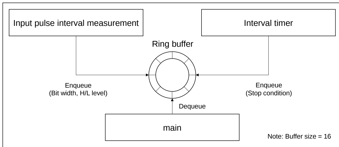
Figure 5-1 Receiver (Rx) overview
