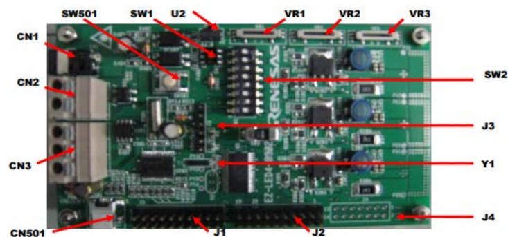
Figure 4-1 RL78 / I1A DC / DC LED Control Evaluation Board(EZ-0012) Components
