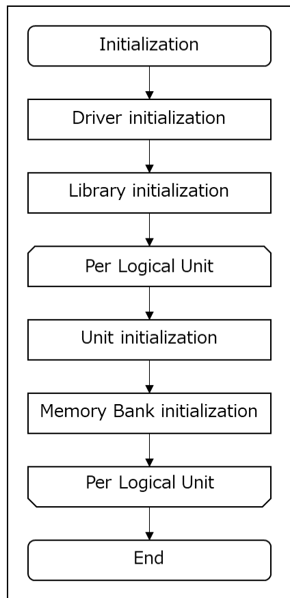
Figure 4-14 Initialization flow diagram
