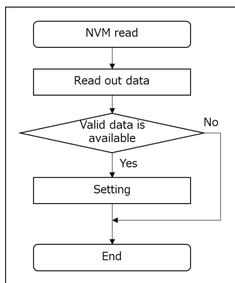
Figure 4-15 NVM reading process flow diagram
