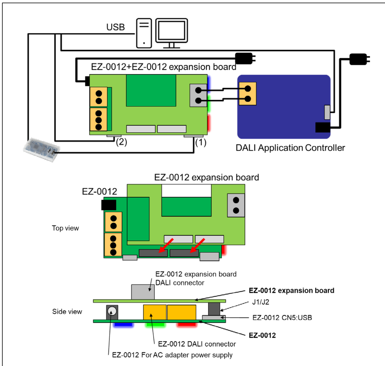
Figure 4-3 Connection diagram when using EZ-0012 expansion board
