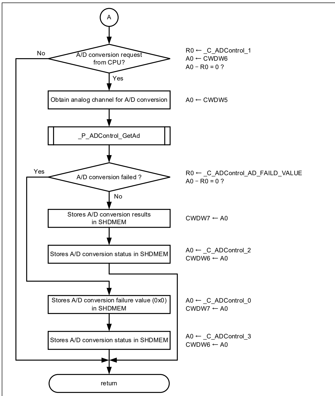
Figure 5-17 _P_ADControl_TAU0_Interrupt (2/2)
