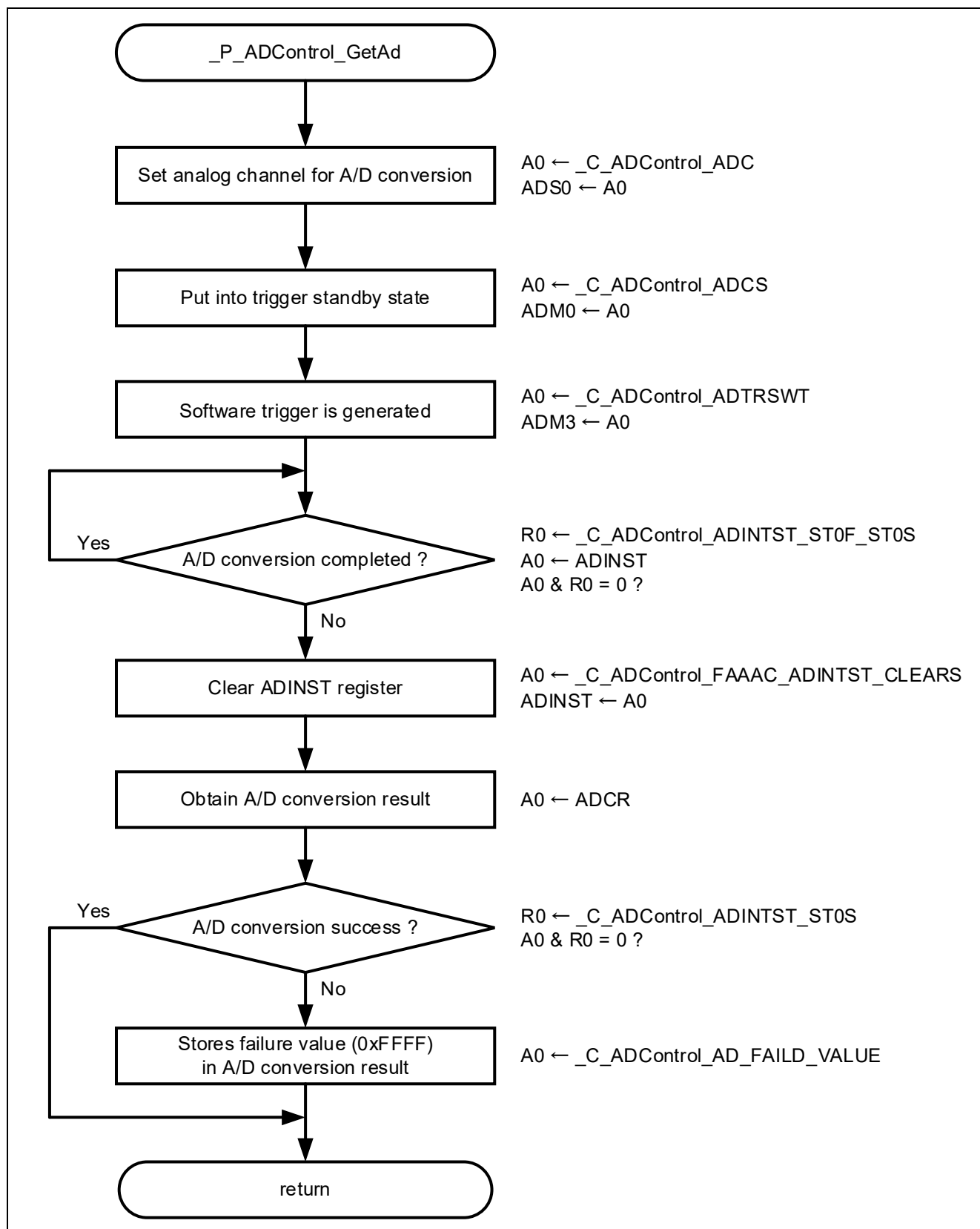
Figure 5-18 _P_ADControl_GetAd
