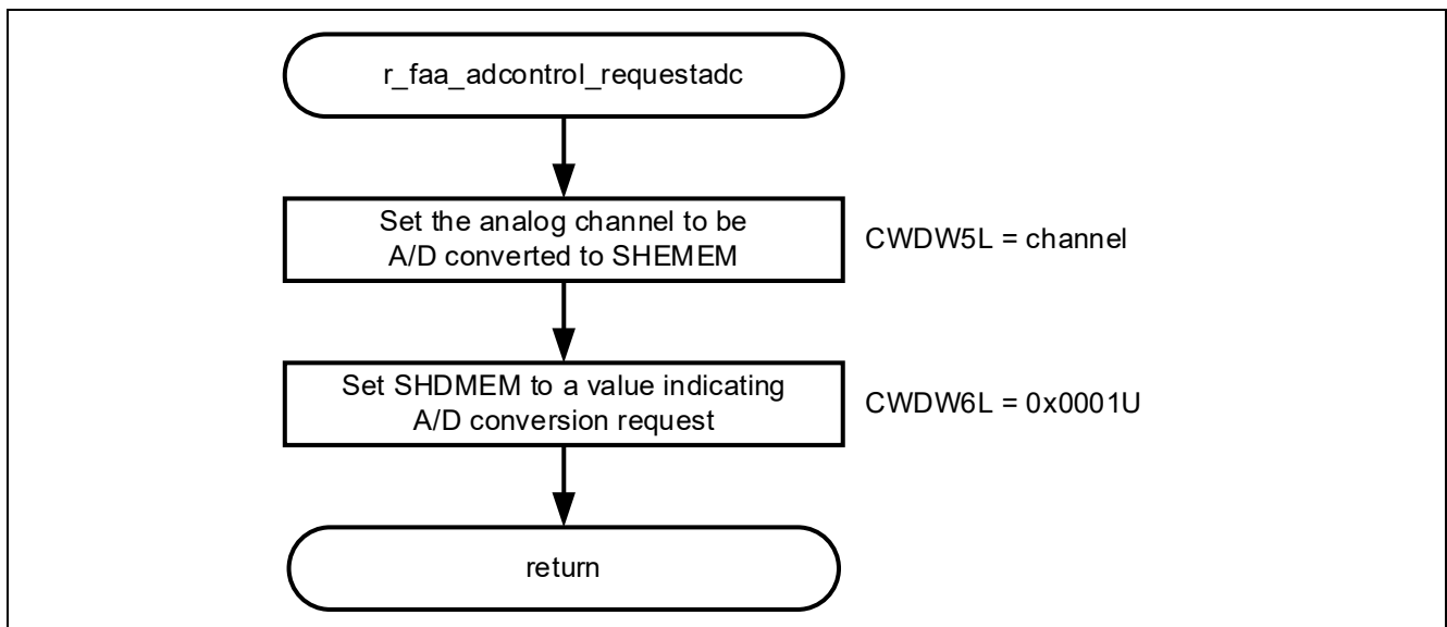
Figure 5-13 r_faa_adcontrol_requestadc function
