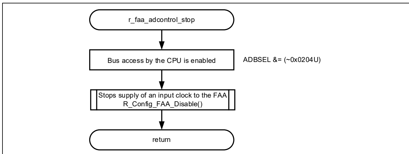
Figure 5-12 r_faa_adcontrol_stop function
