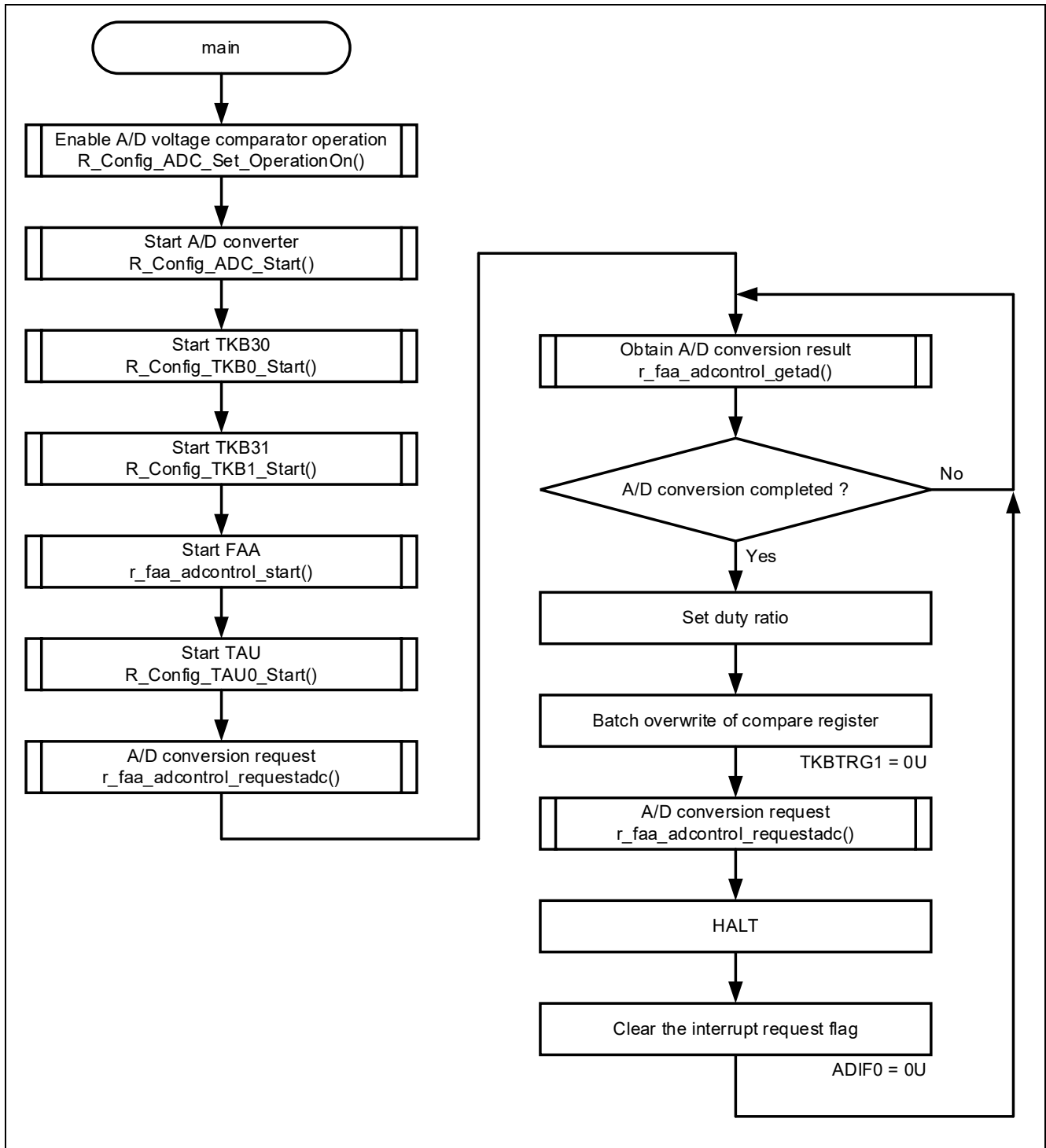
Figure 5-10 Main Process
