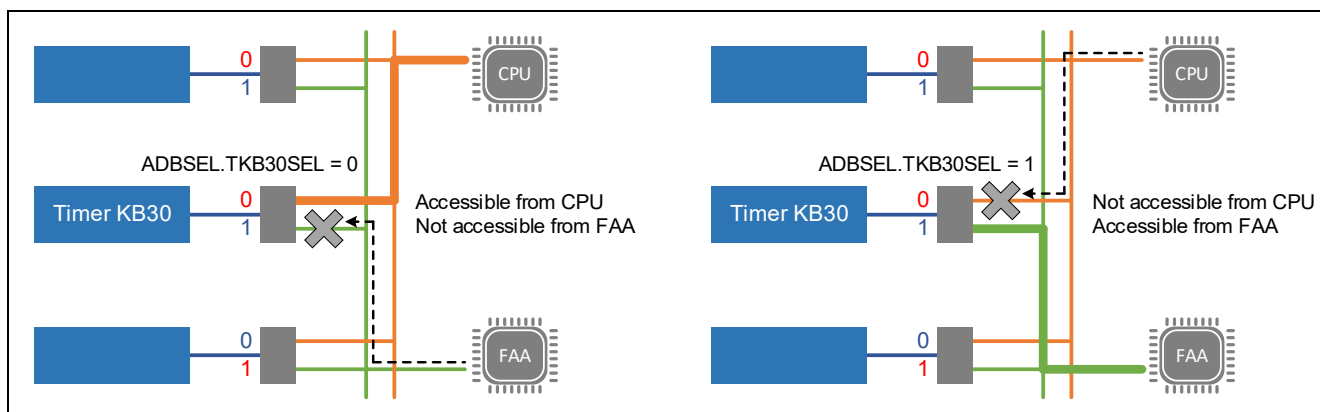
Figure 1-2 Overview of Address Bus Select Function
