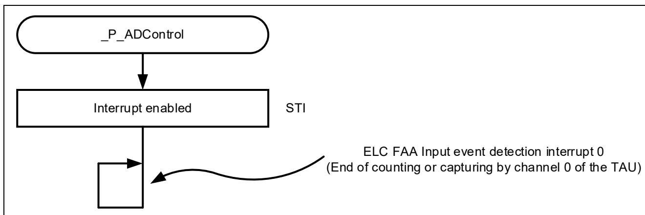
Figure 5-15 _P_ADControl
