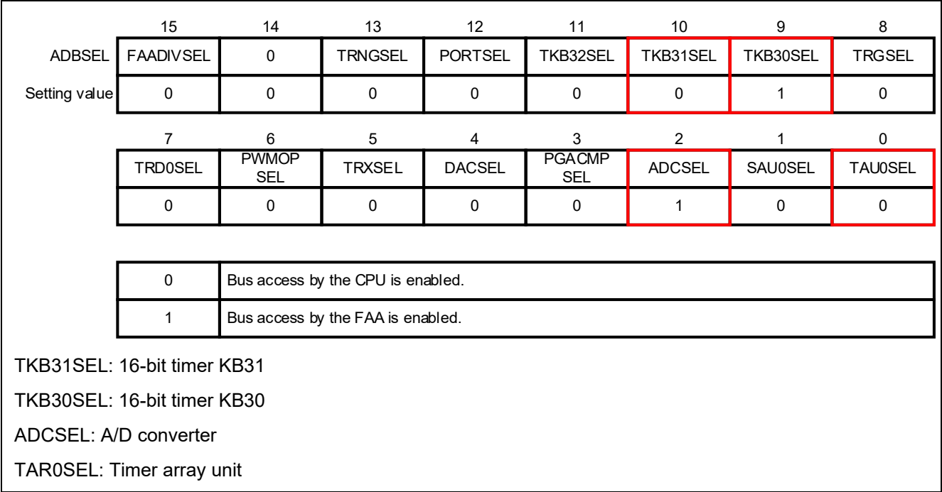
Figure 2-1 Allocation in Address Bus Select Register (ADBSEL)
