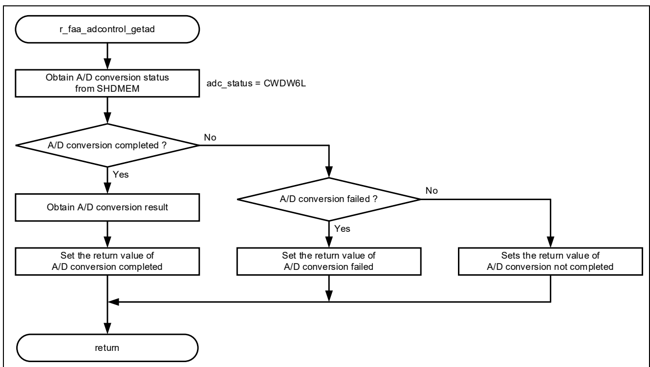
Figure 5-14 r_faa_adcontrol_getad function
