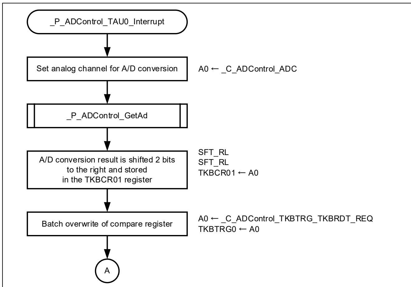
Figure 5-16 _P_ADControl_TAU0_Interrupt (1/2)
