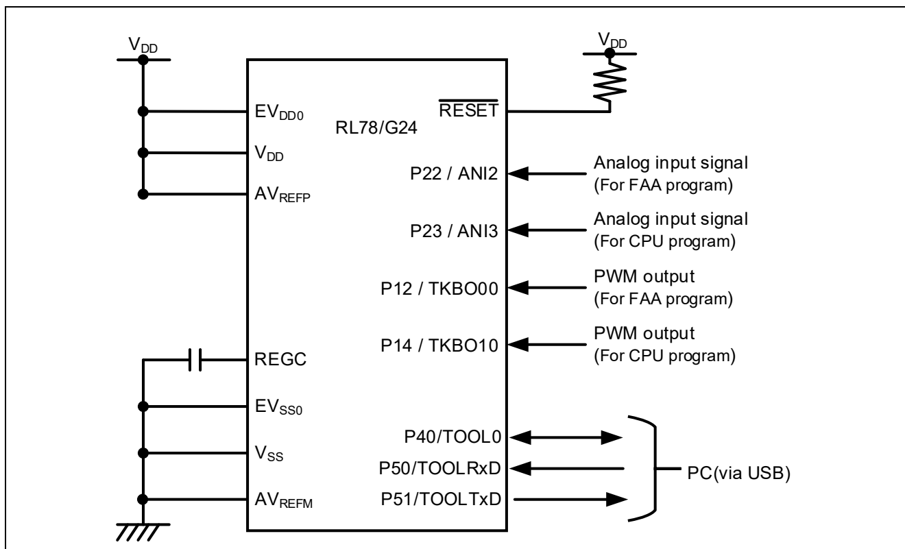
Figure 4-1 Example of Hardware Configuration
