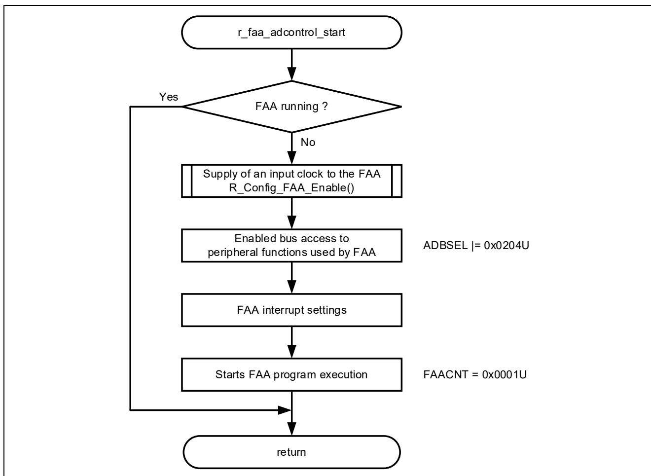
Figure 5-11 r_faa_adcontrol_start function
