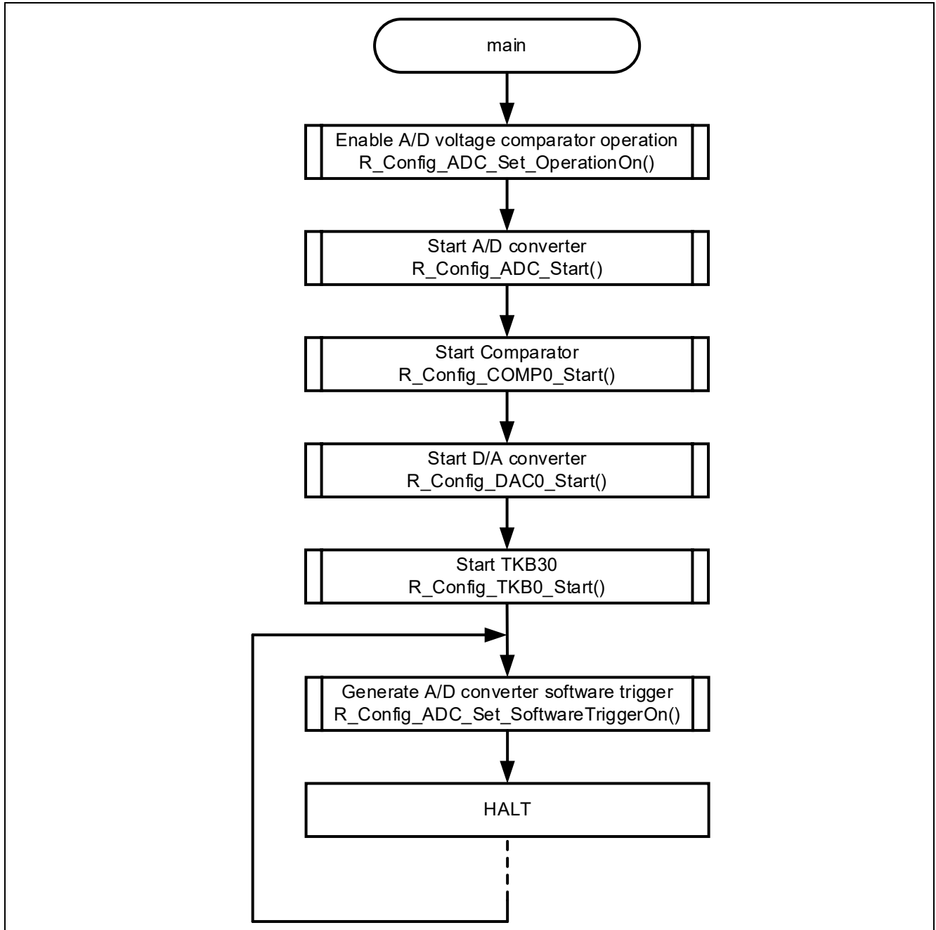
Figure 4-8 Main Process
