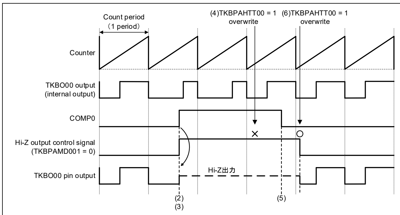
Figure 1-2 Example of Over-Current Protection Output Using Forced Output Stop Function 1
