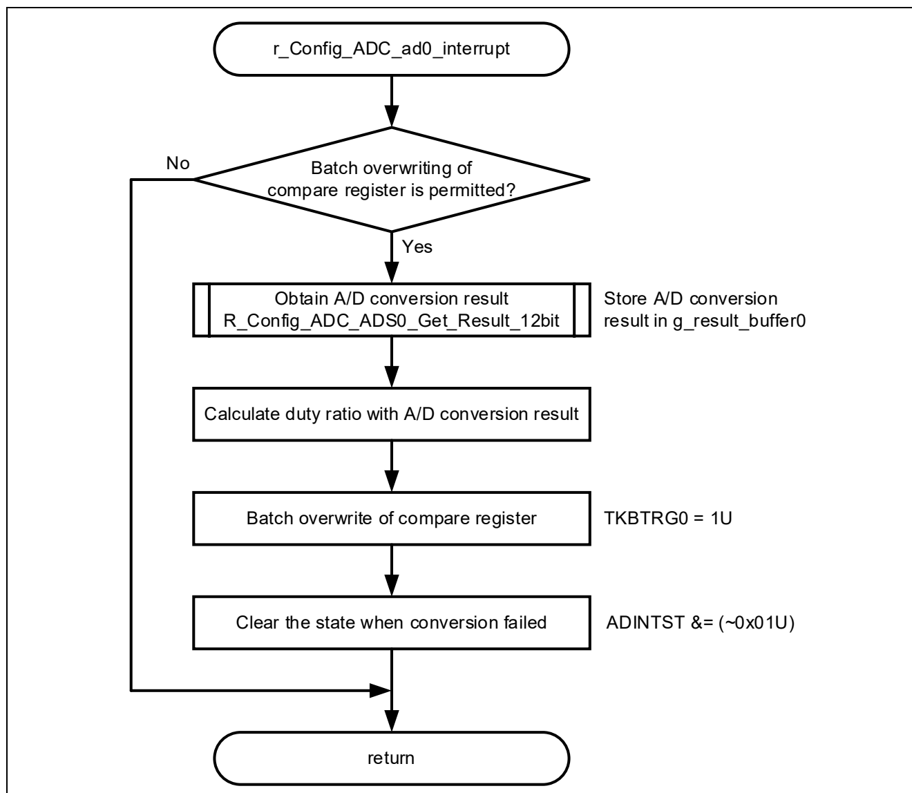
Figure 4-9 r_Config_ADC_ad0_interrupt function
