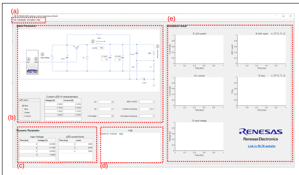
Figure 4.1. execution window
