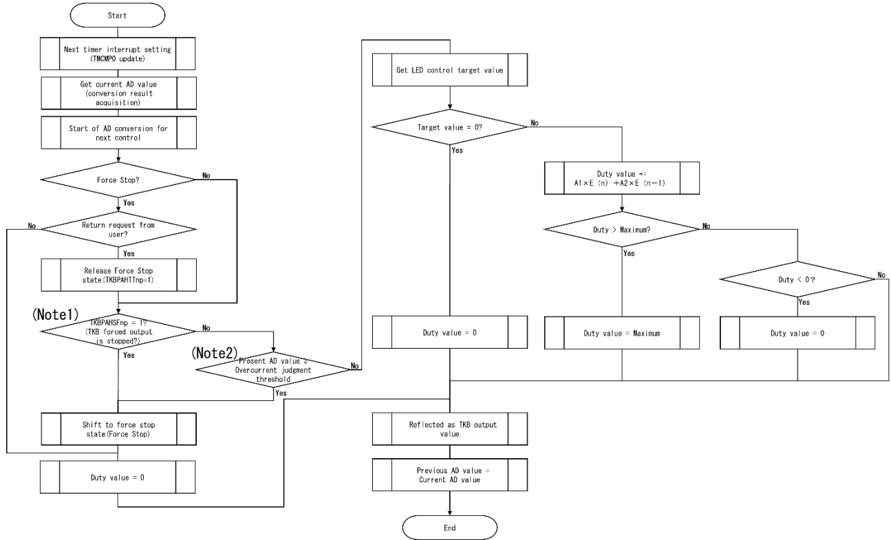
Figure 6-5 LED Control Feedback Processing (High-speed Operation)
