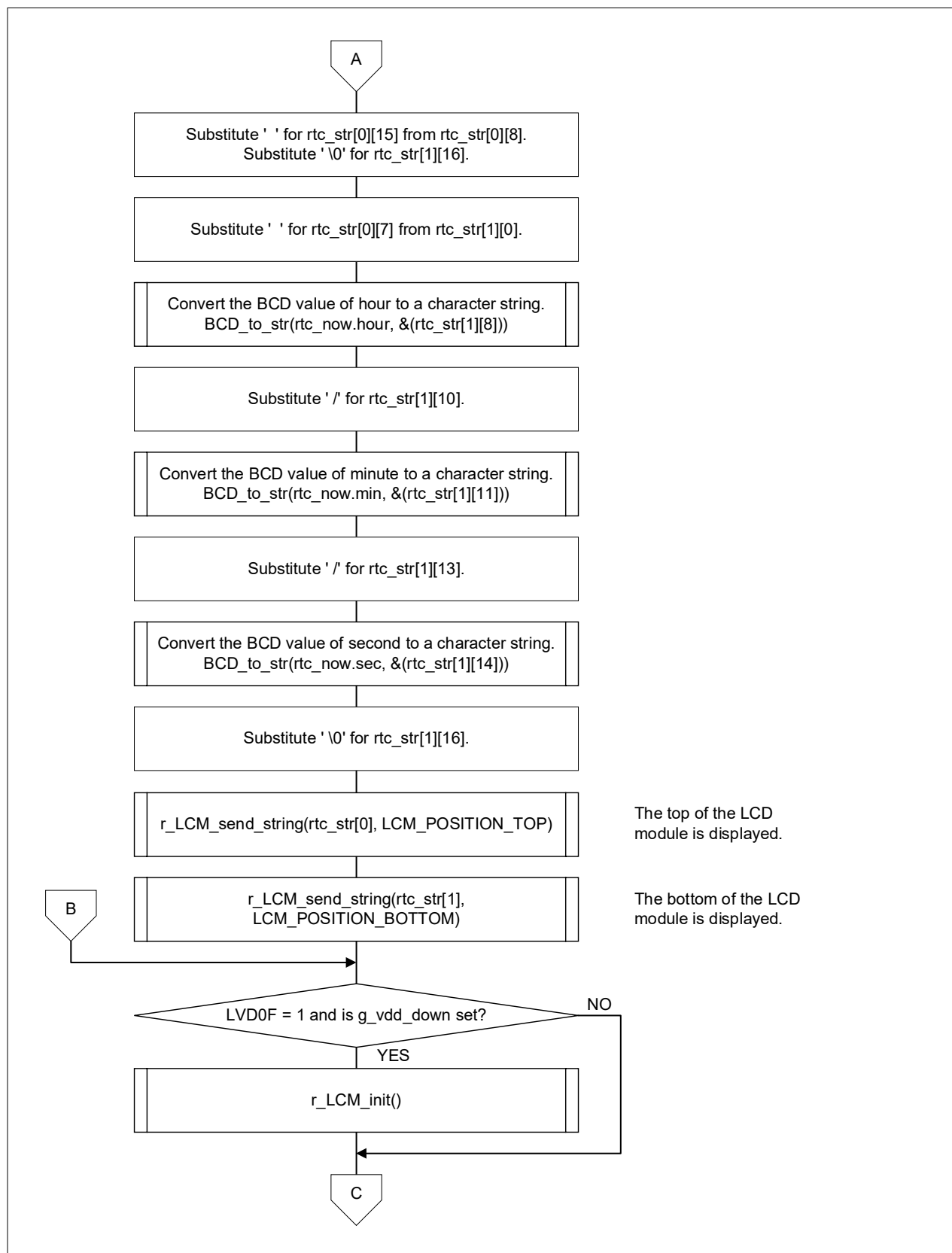
Figure 4-2 Main Processing (2/2)
