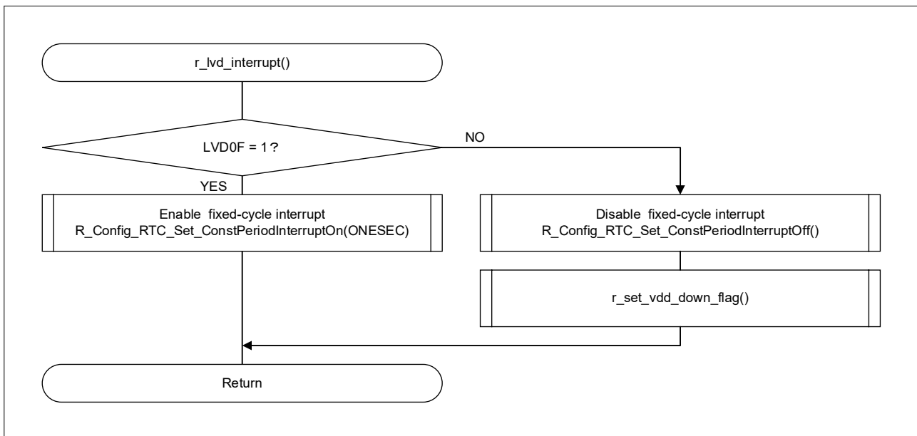
Figure 4-16 LVD0 Interrupt Processing
