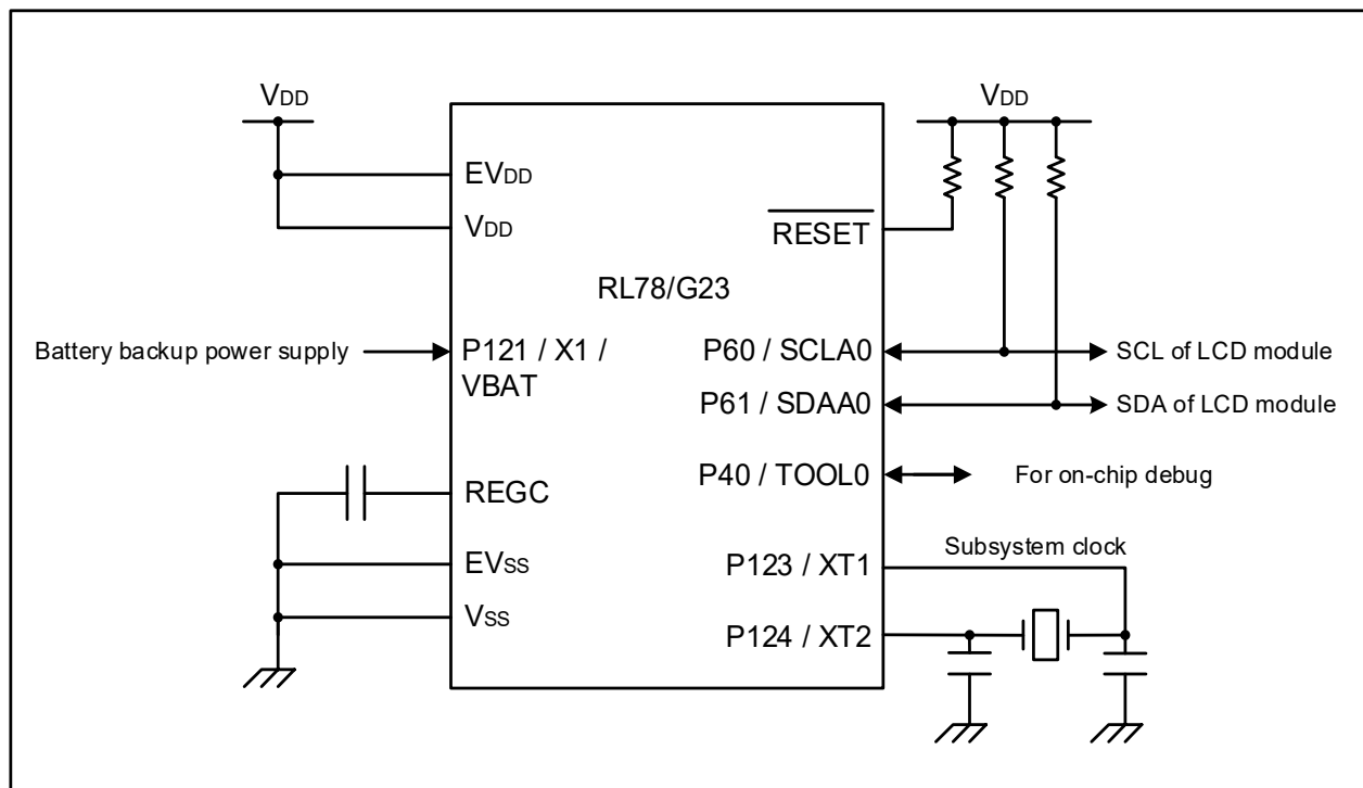
Figure 3-1 Hardware Configuration
