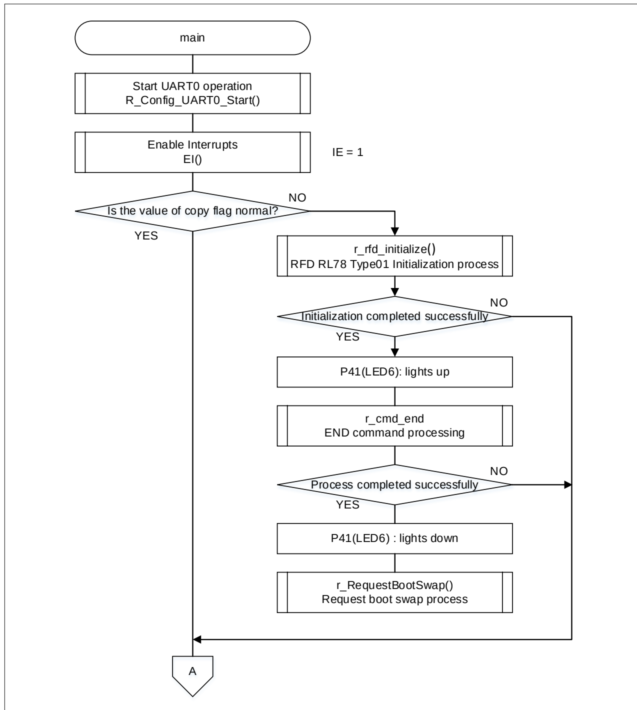
Figure 4-1 Main Processing (1/2)
