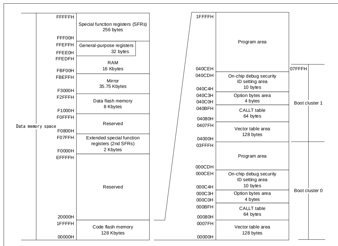
Figure 1-1 Memory Map
