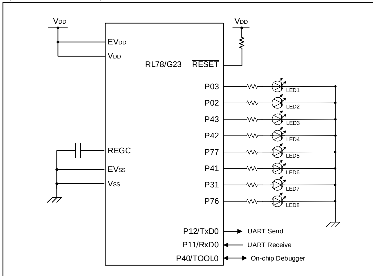
Figure 3-1 Hardware Configuration
