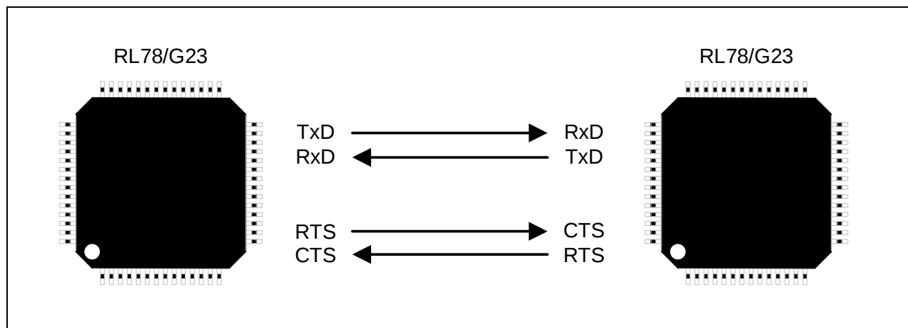
Figure 1-1 Flow Control Block Diagram
