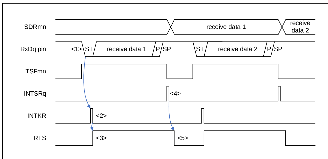
Figure 1-2 Timing Chart for Data Reception
