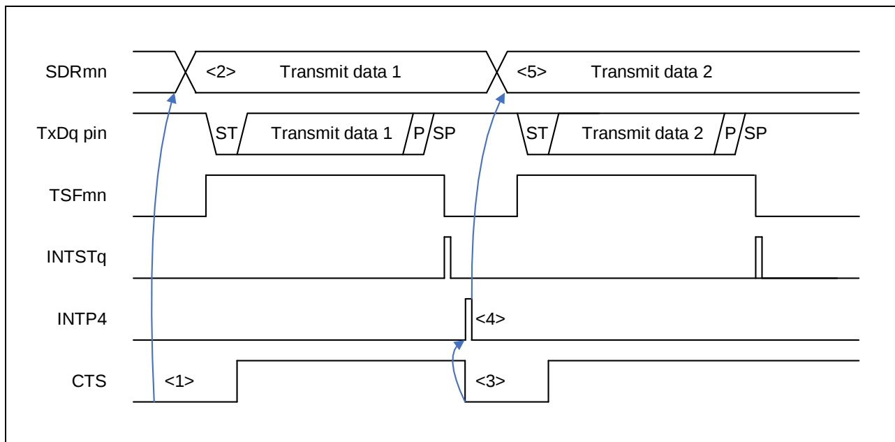
Figure 1-3 Timing Chart for UART Transmission
