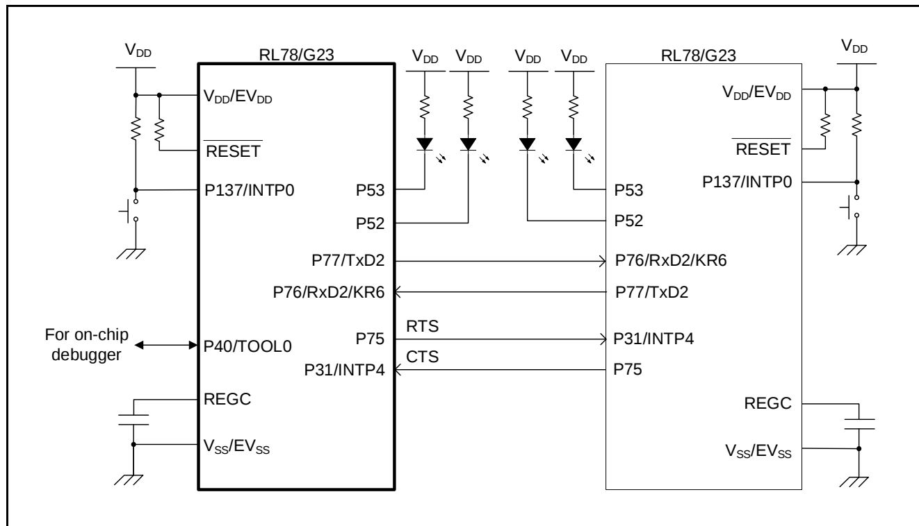
Figure 3-1 Hardware Configuration
