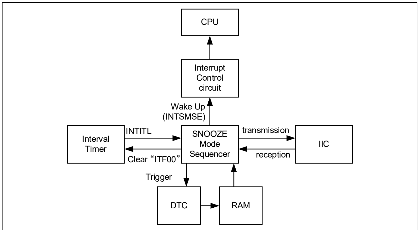
Figure 1-2 System Configuration
