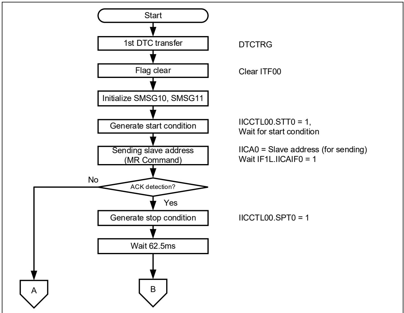
Figure 5-8 SMS process
