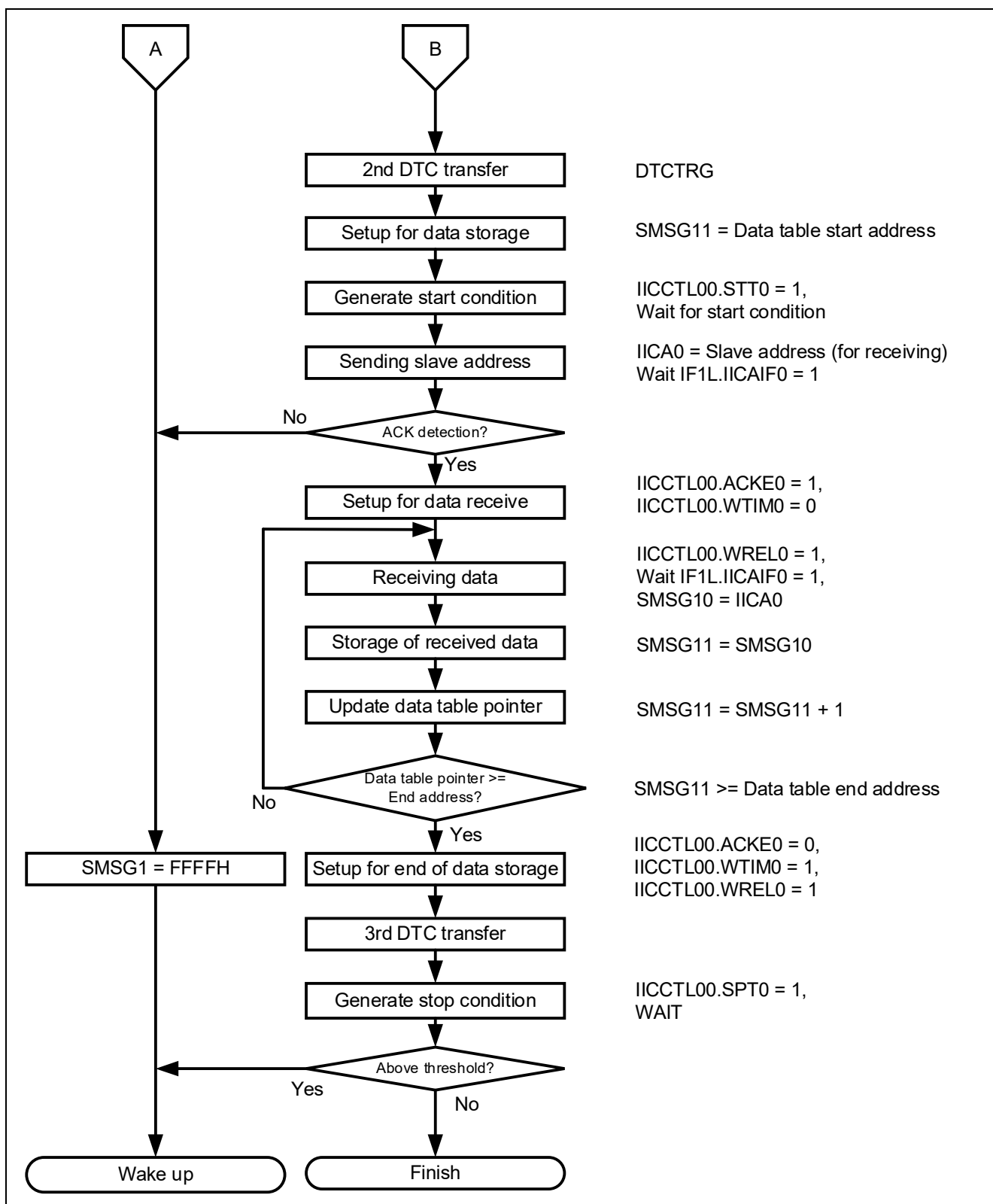
Figure 5-9 SMS process
