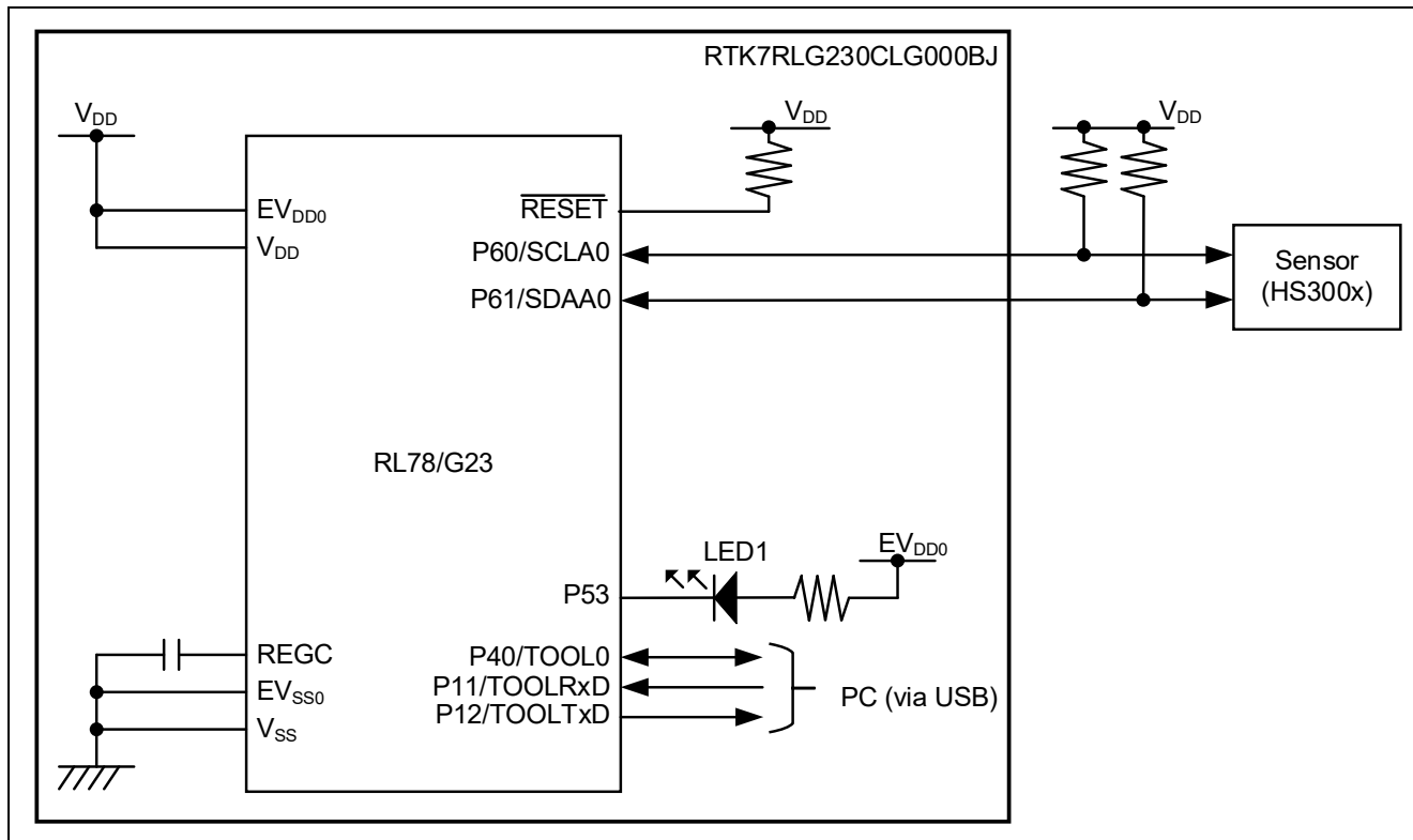
Figure 4-1 Hardware Configuration
