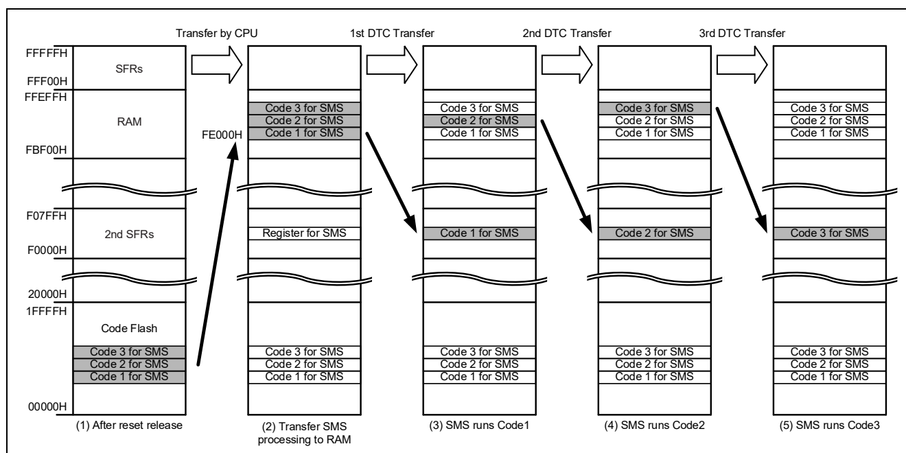
Figure 1-1 Memory map
