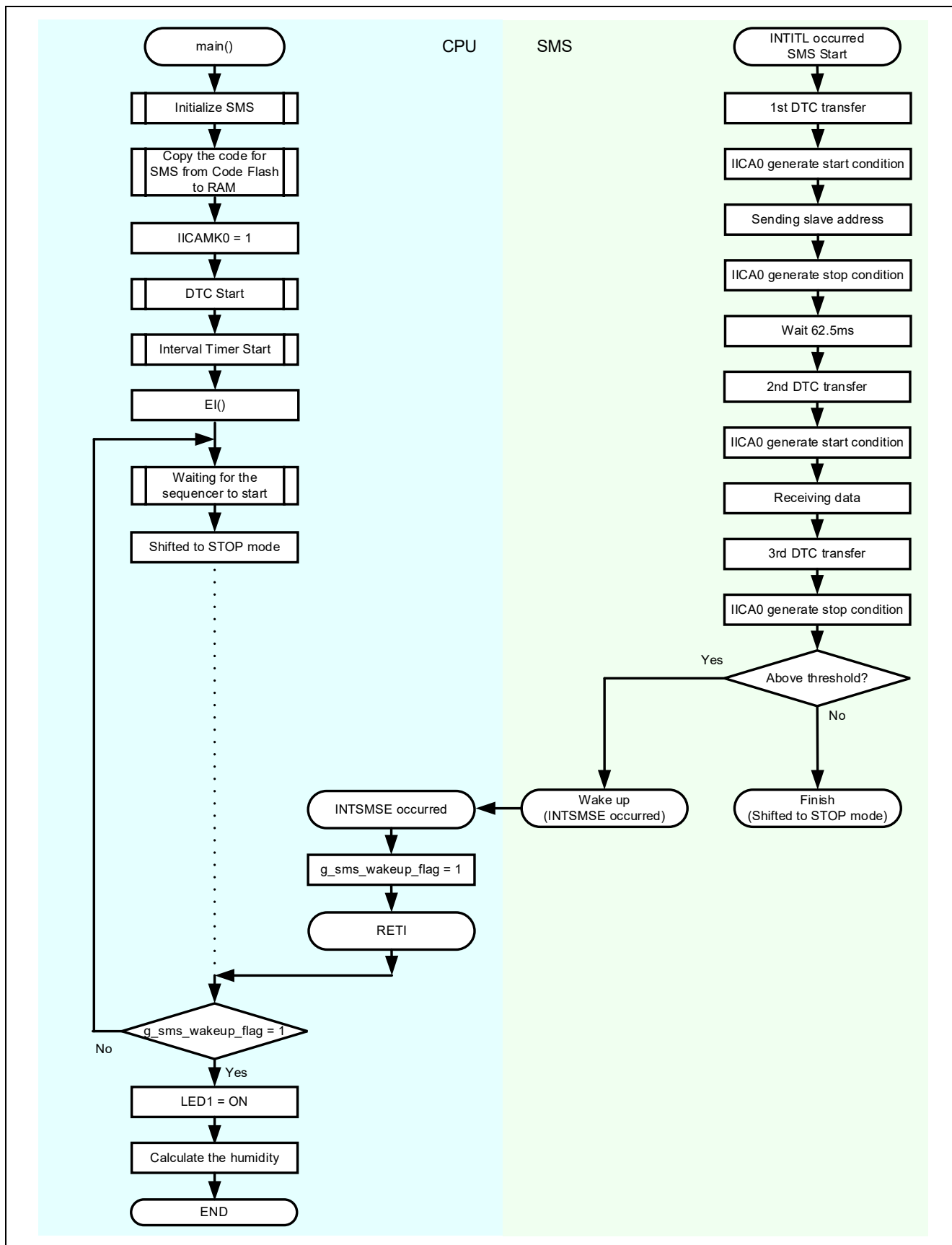
Figure 1-3 Entire Flowchart
