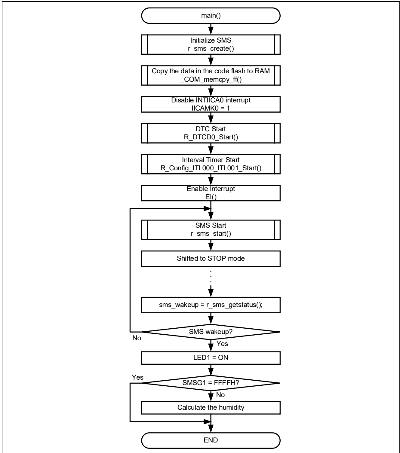
Figure 5-1 Main process
