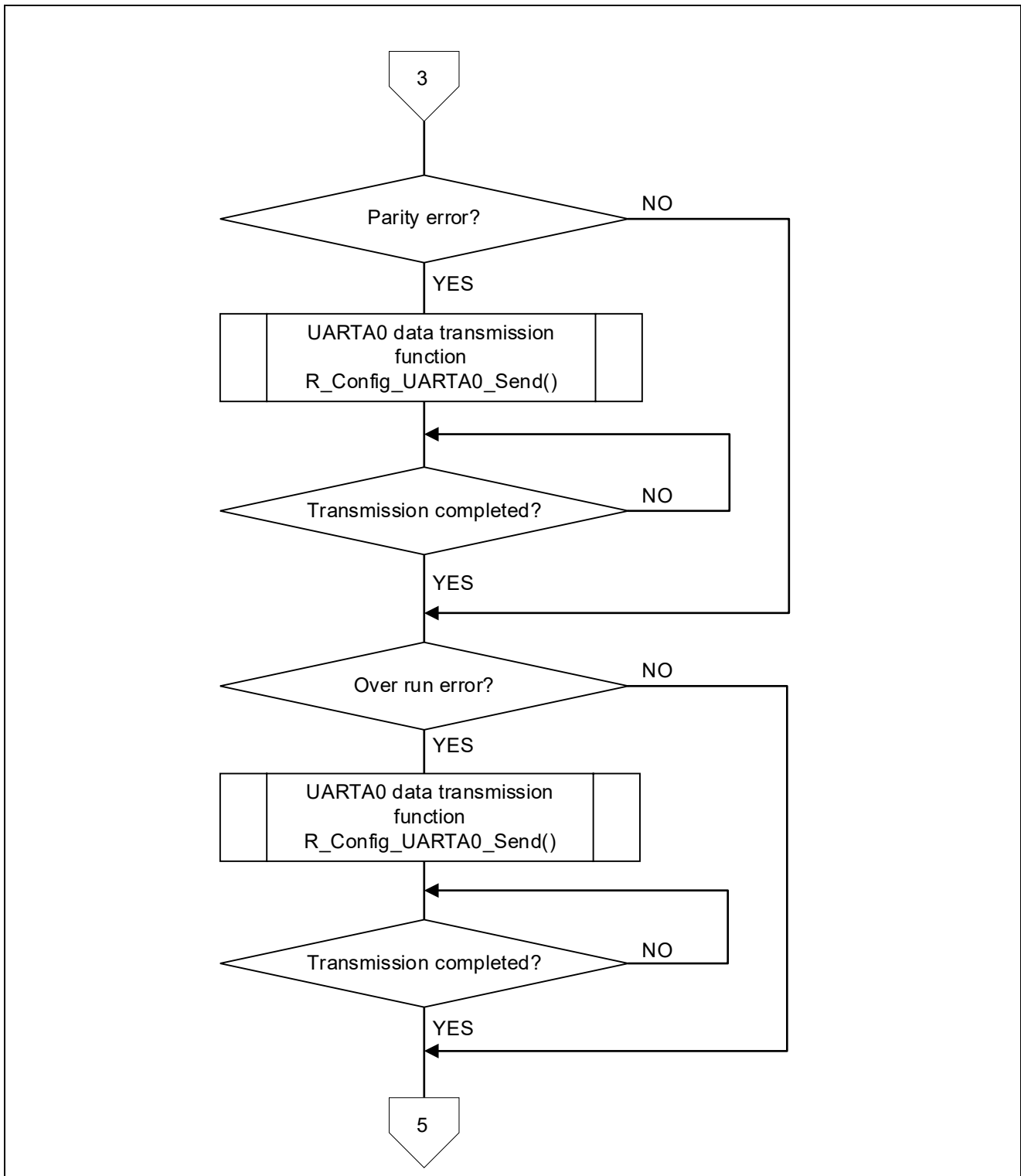
Figure 4.2 Main Function (2/3)
