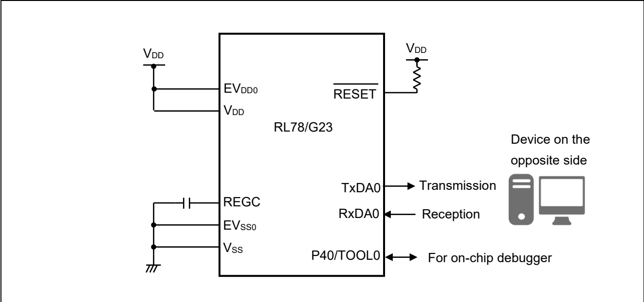
Figure 3.1 Hardware Configuration
