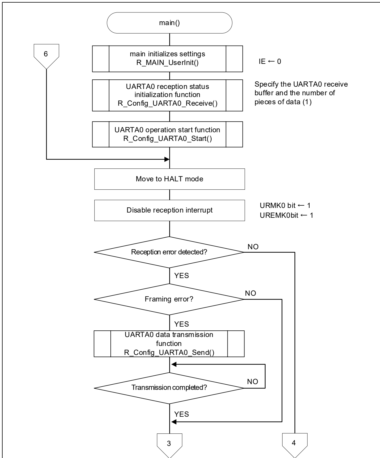
Figure 4.1 Main Function (1/3)
