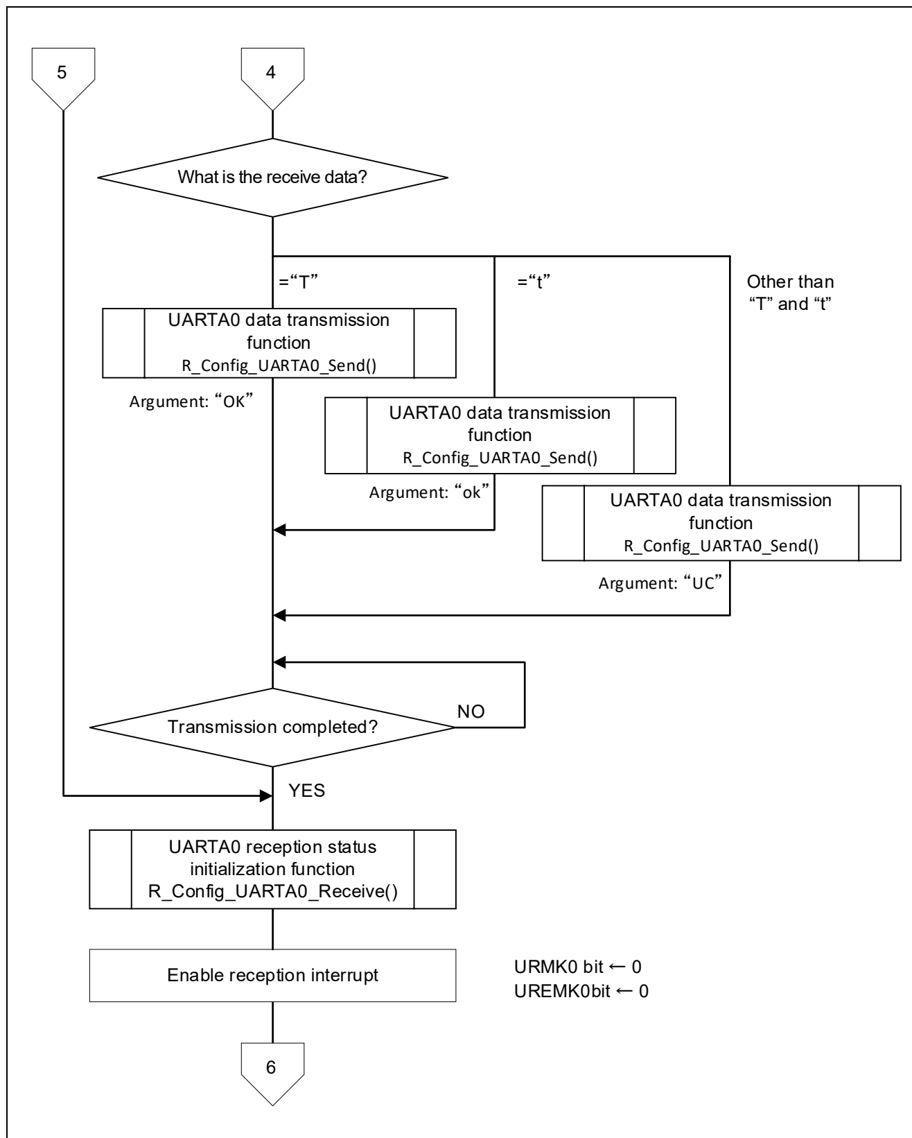
Figure 4.3 Main Function (3/3)
