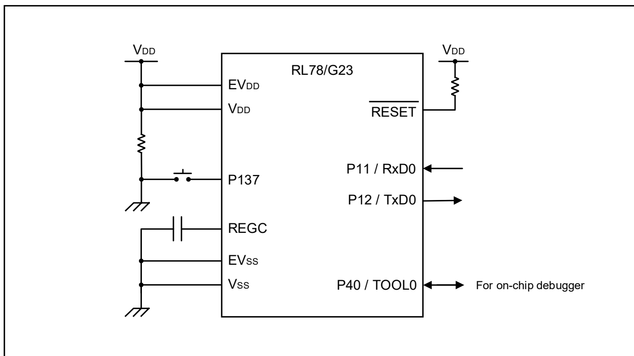
Figure 3-1 Hardware Configuration
