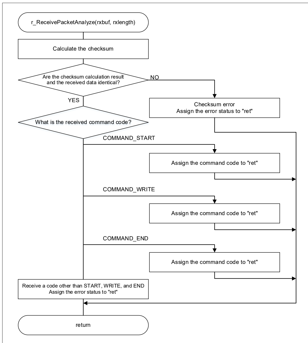
Figure 4-21 Command Analysis Processing by UART0
