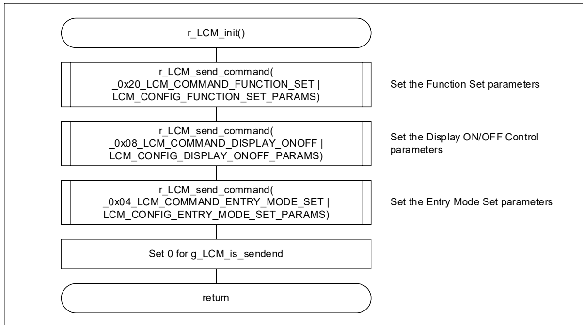
Figure 4-27 Processing to Initialize the LCD Module
