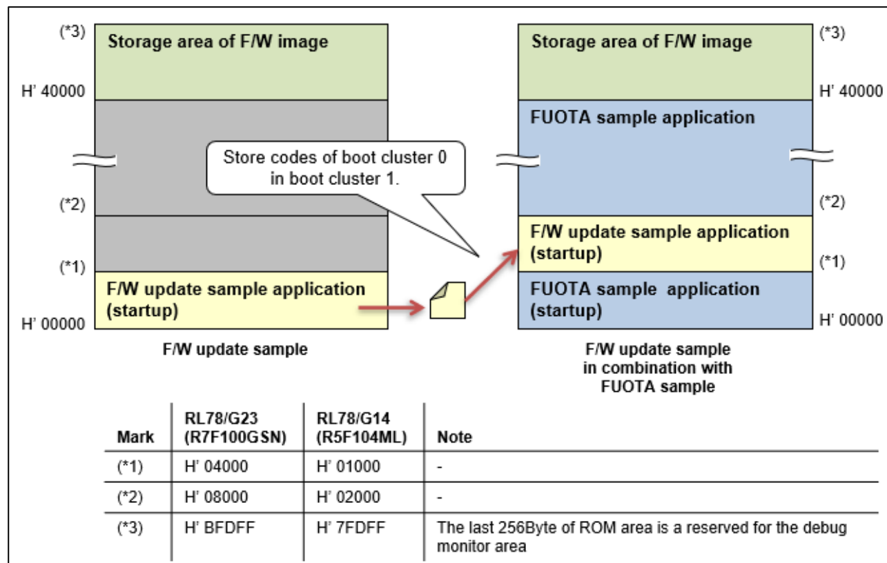
Figure 16 ROM Mapping
