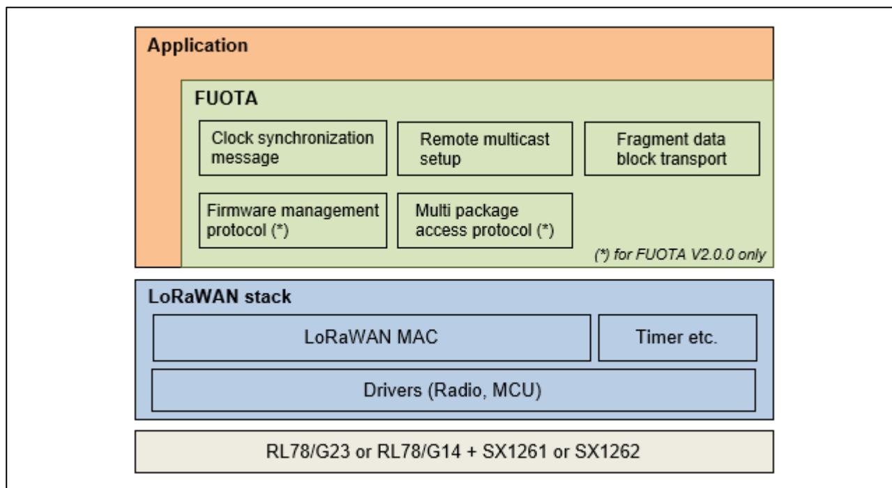
Figure 22 FUOTA V2.0.0 Sample Application Block Diagram
