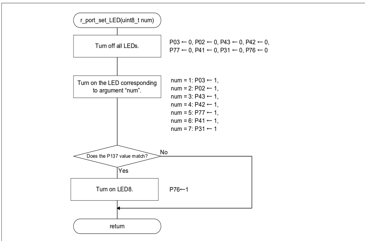
Figure 4-7 LED Lighting Control
