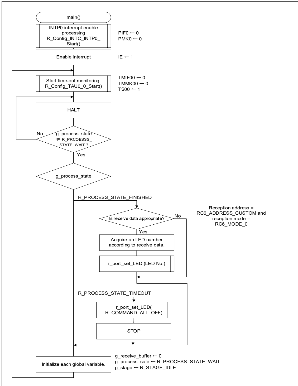
Figure 4-1 Main Processing
