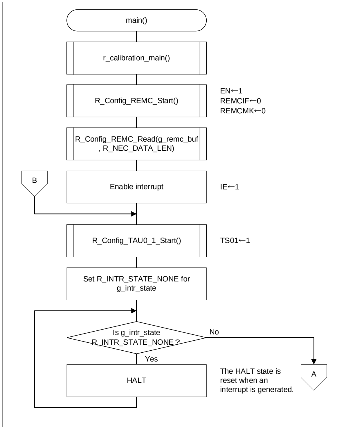
Figure 4-1 Main Processing (1/2)
