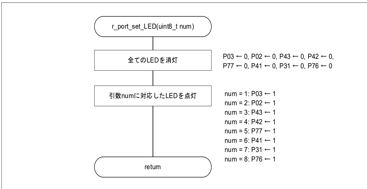
図 4-4 LED 点灯制御
