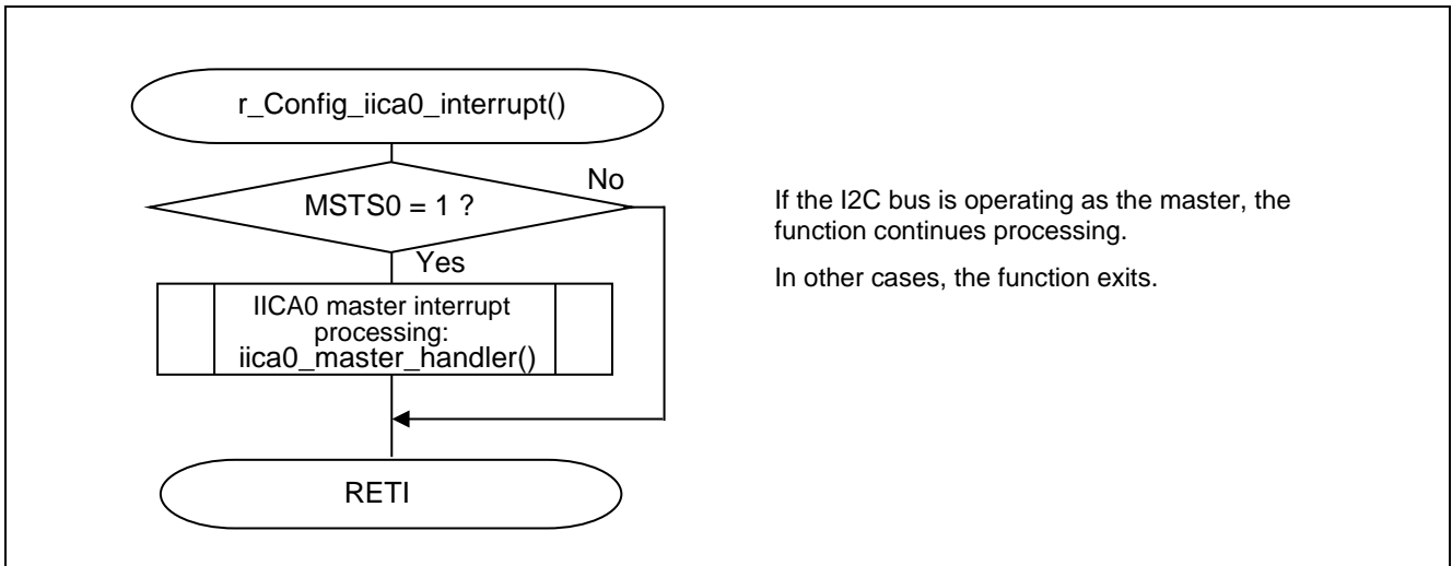
Figure 4-5 IICA0 Interrupt Processing Function
