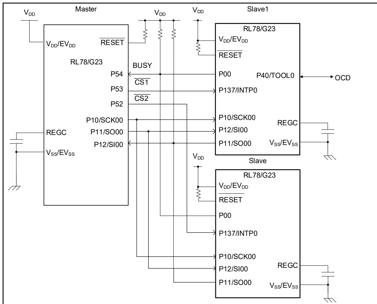
Figure 4-1 Hardware Configuration
