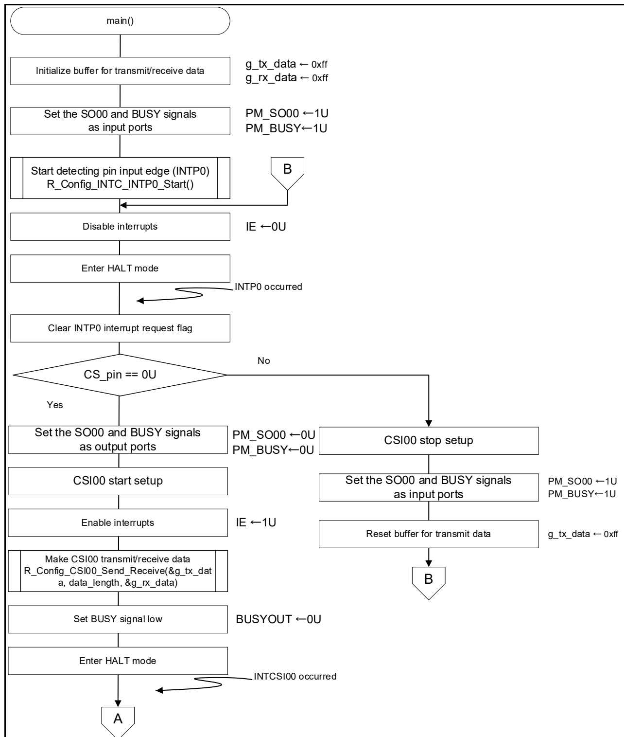
Figure 5-1 Main Processing 1/2
