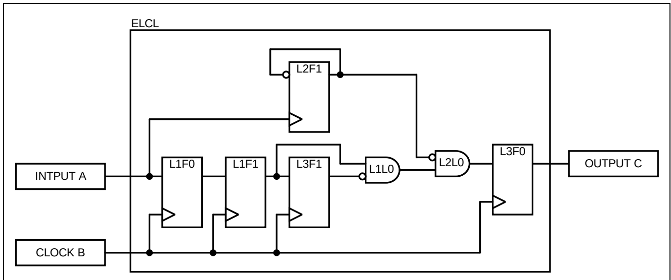
Figure 1-1 System Configuration
