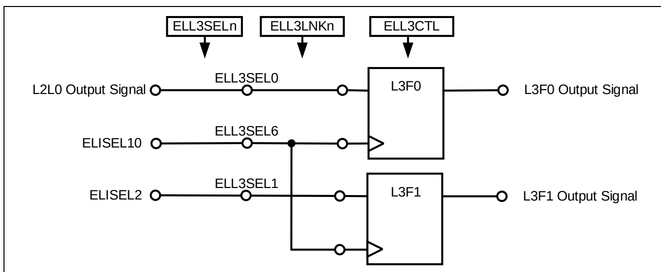
Figure 5-8 Setting of logic cells L3
