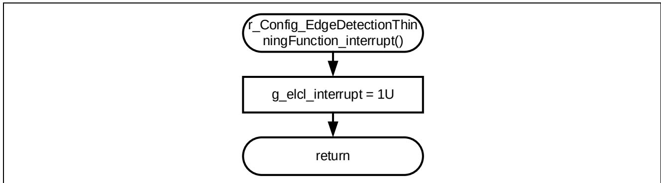
Figure 4-4 ELCL interrupt process
