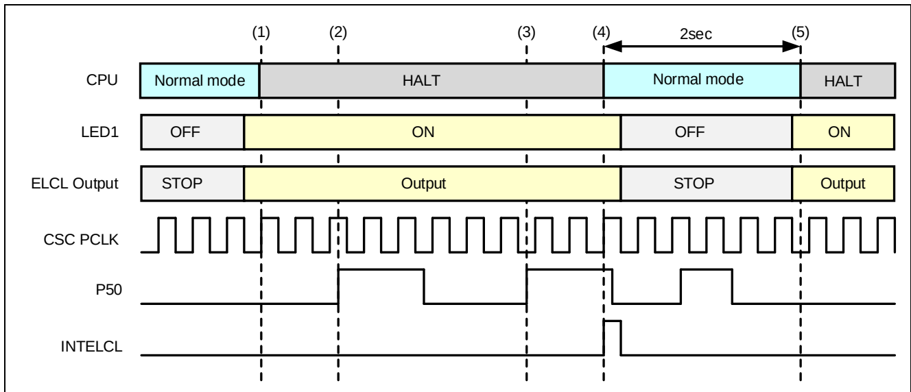
Figure 4-2 Timing chart of the sample code
