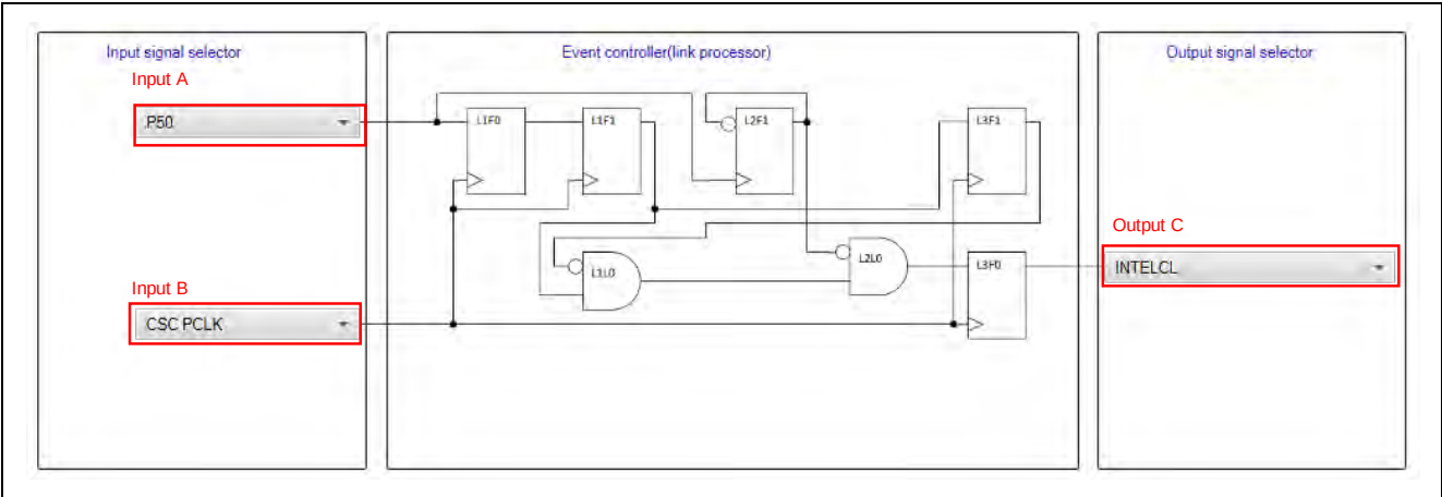
Figure 5-4 Component "ELCL edge detection thinning function"
