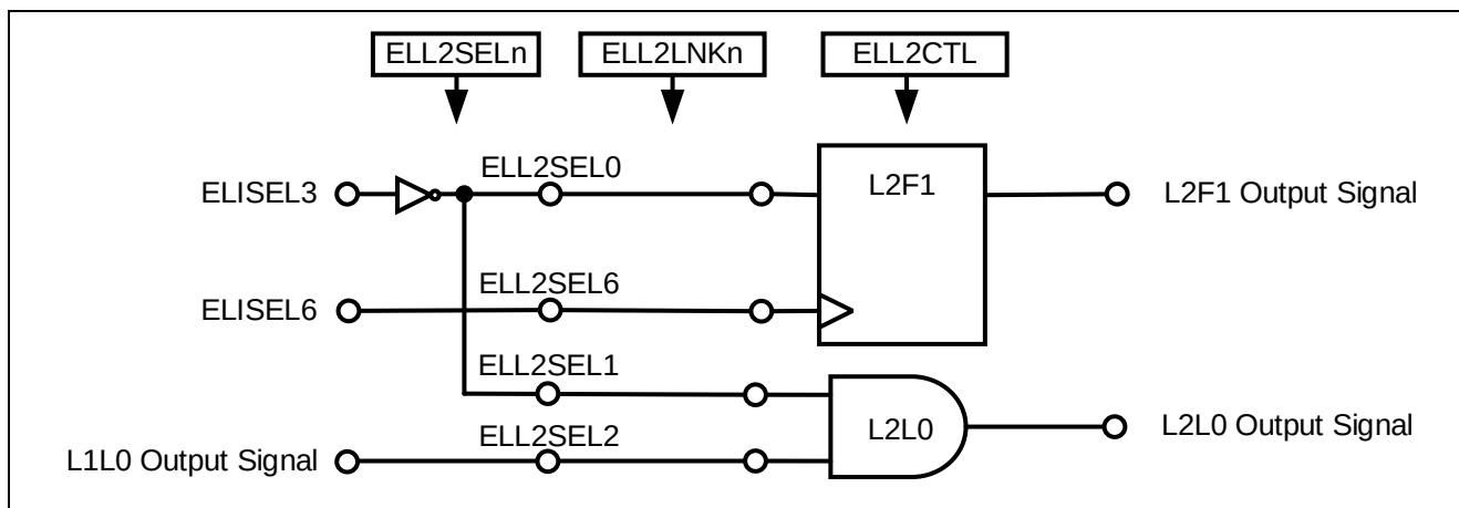
Figure 5-7 Setting of logic cells L2
