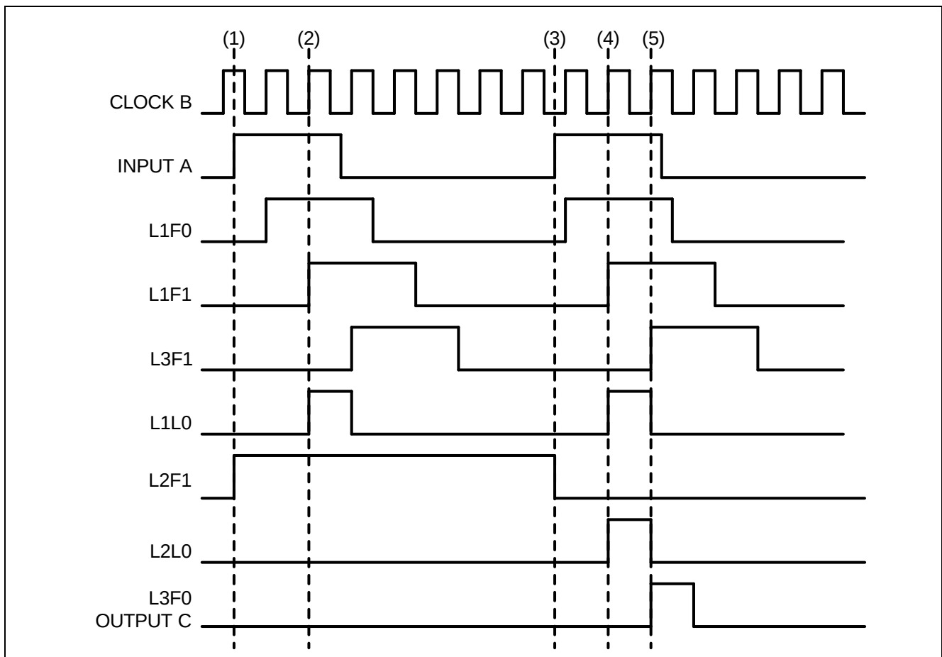
Figure 1-2 Timing chart of Edge detection thinning
