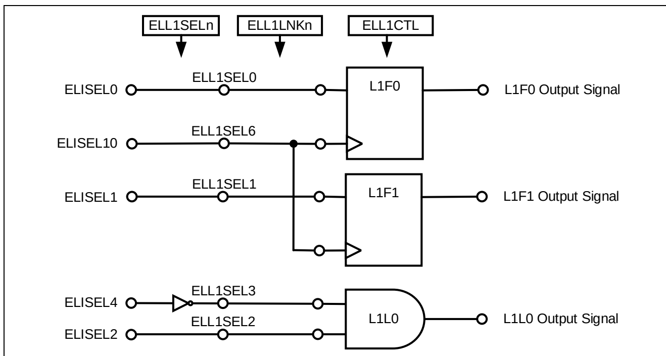
Figure 5-6 Setting of logic cells L1
