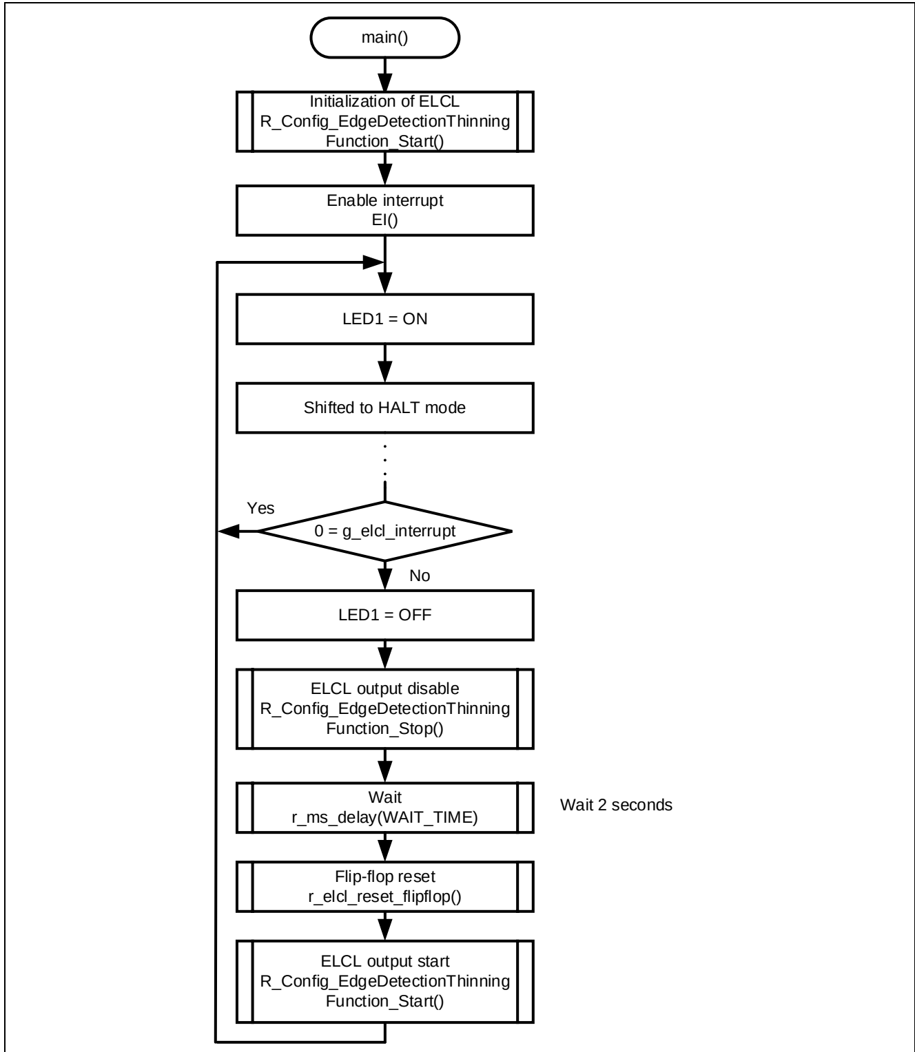
Figure 4-3 Main process
