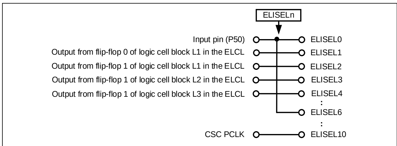
Figure 5-5 Setting of ELCL input
