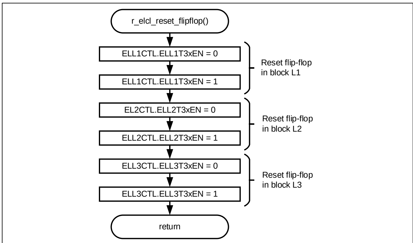
Figure 4-5 ELCL flip-flop reset process
