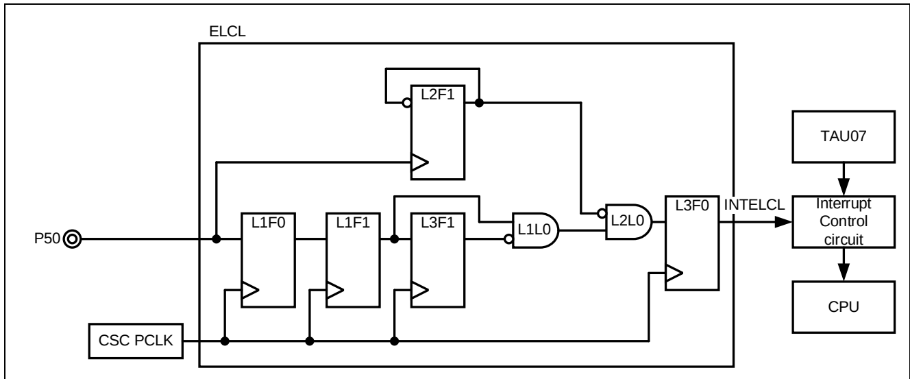
Figure 4-1 System configuration of the sample code
