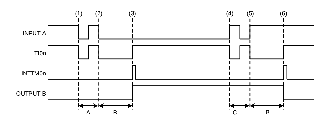
Figure 1-3 Timing chart of chattering prevention control
