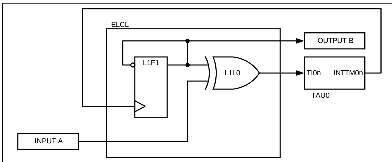
Figure 1-2 System Configuration
