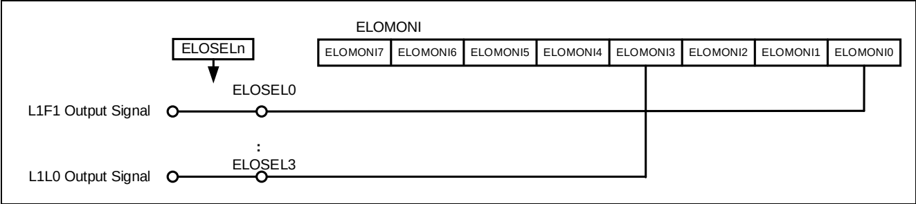
Figure 5-7 Settings of ELCL output
