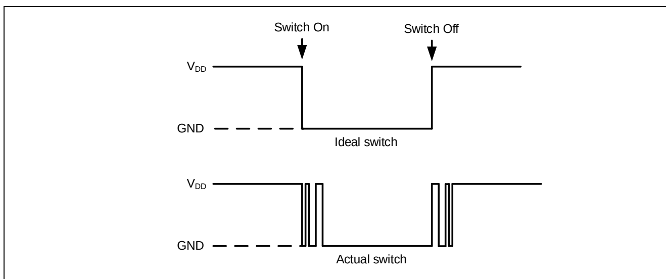
Figure 1-1 Switch waveform
