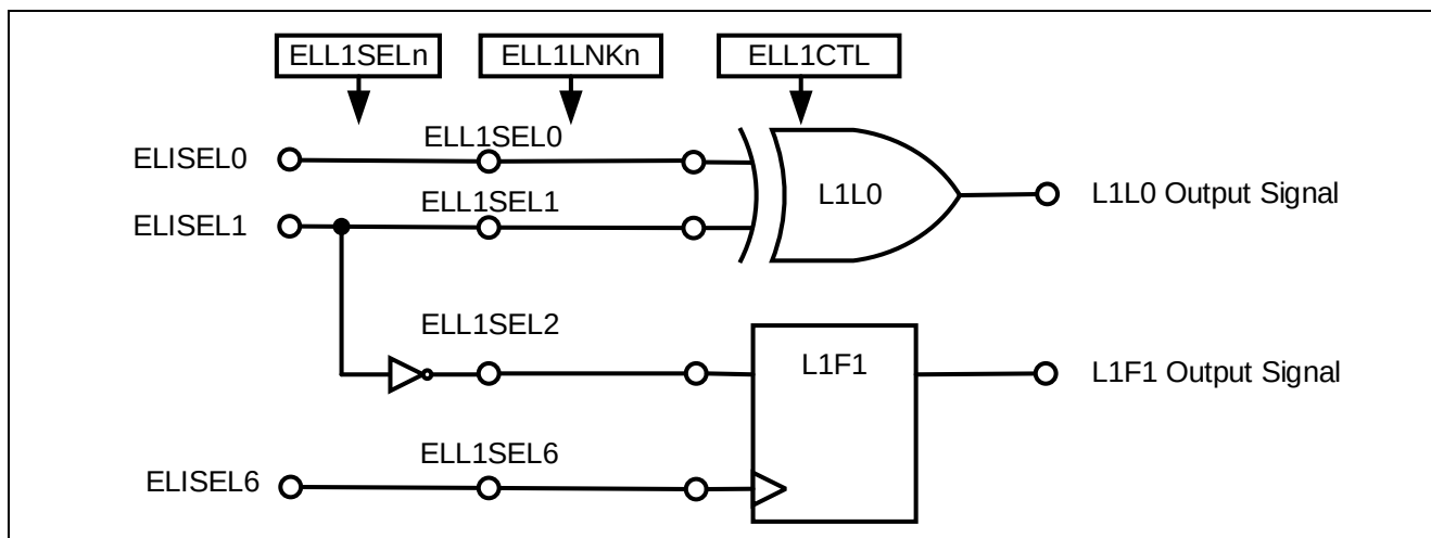
Figure 5-6 Setting of logic cells L1
