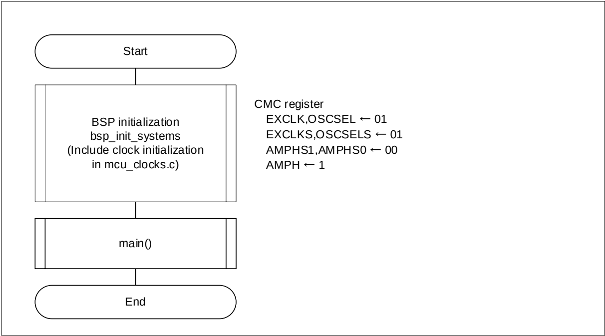
Figure 4-1 Overall Flowchart
