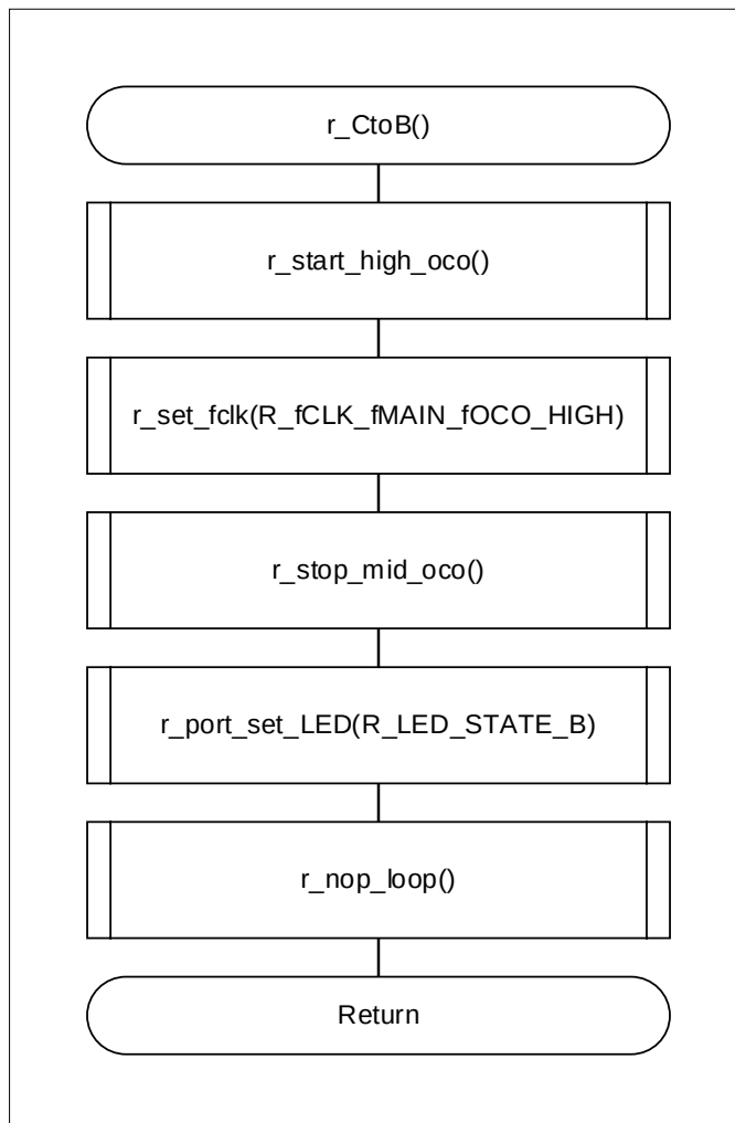
Figure 4-38 Status Transition CtoB
