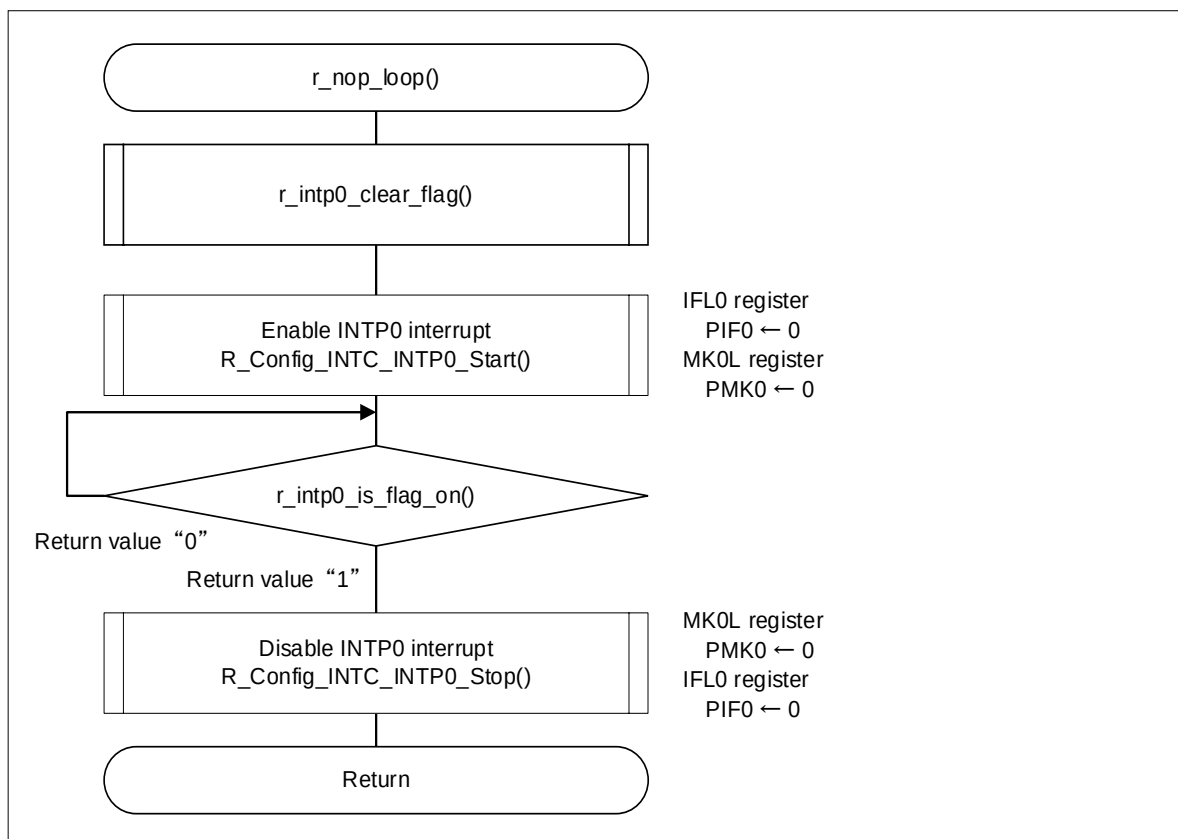
Figure 4-46 Waiting for an Interrupt (Repetition of NOP)
