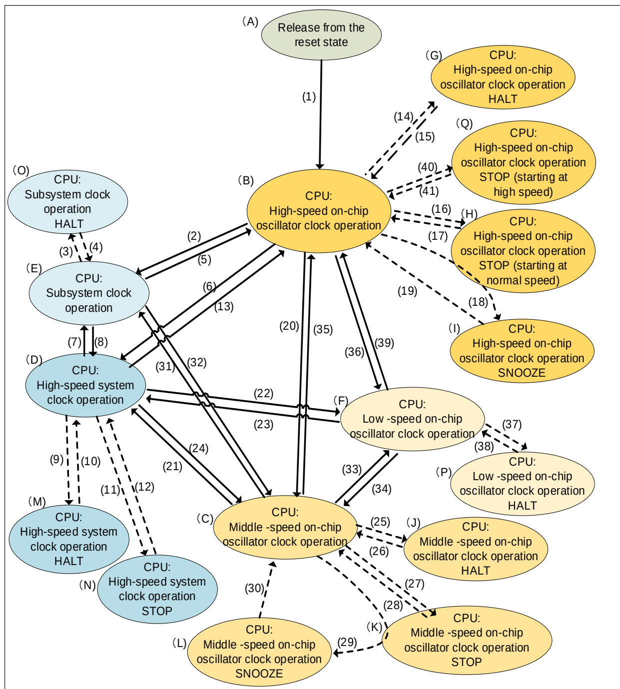
Figure 1-1 Operating Mode Status Transition Diagram
