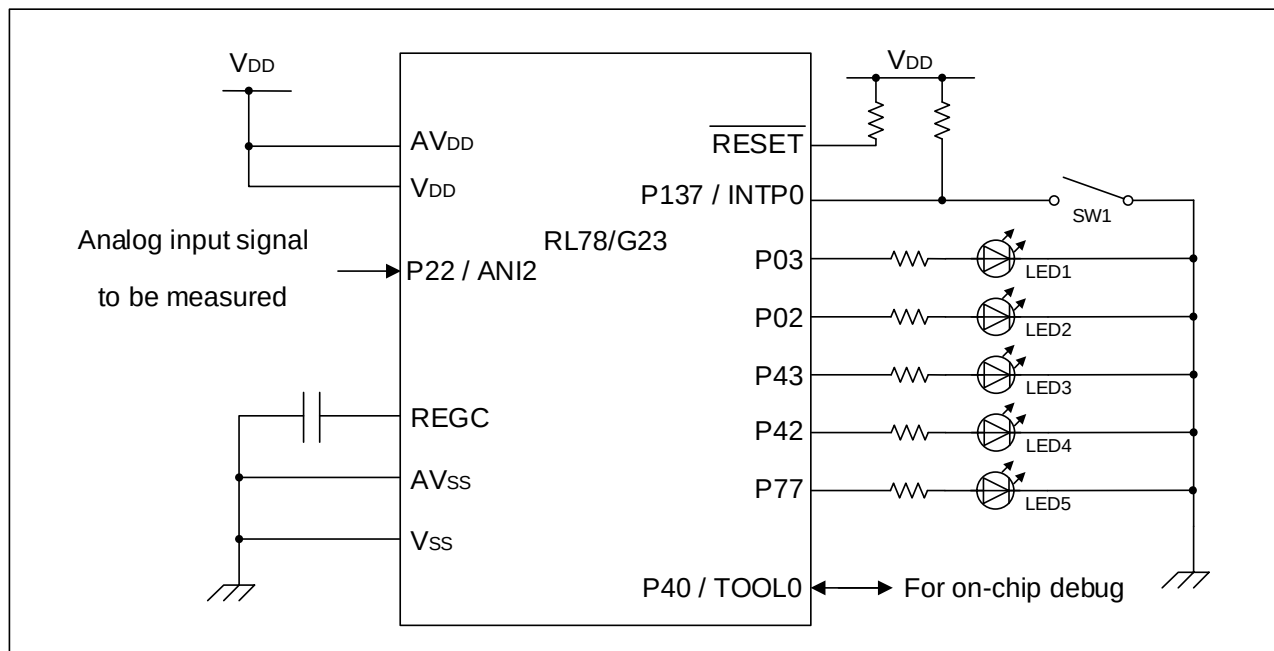
Figure 3-1 Hardware Configuration
