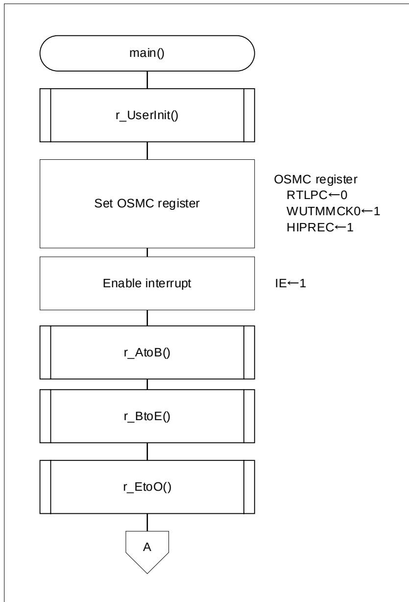
Figure 4-2 Main Processing (1/2)
