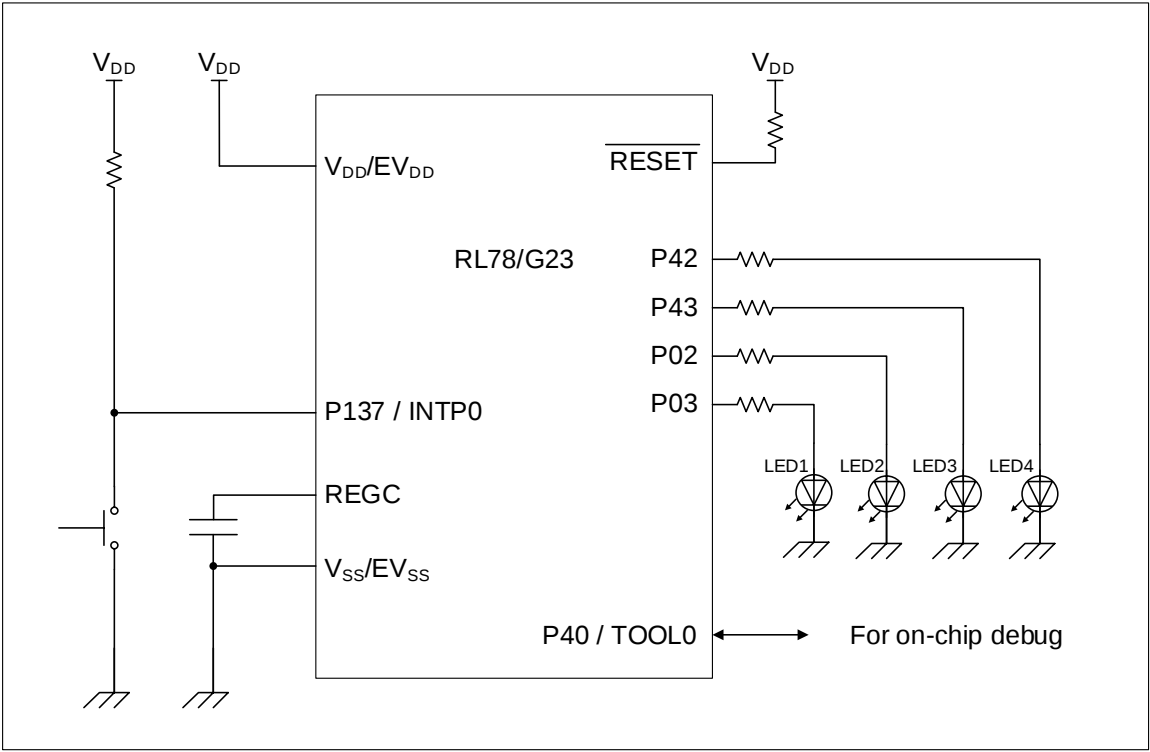
Figure 3-1 Hardware Configuration
