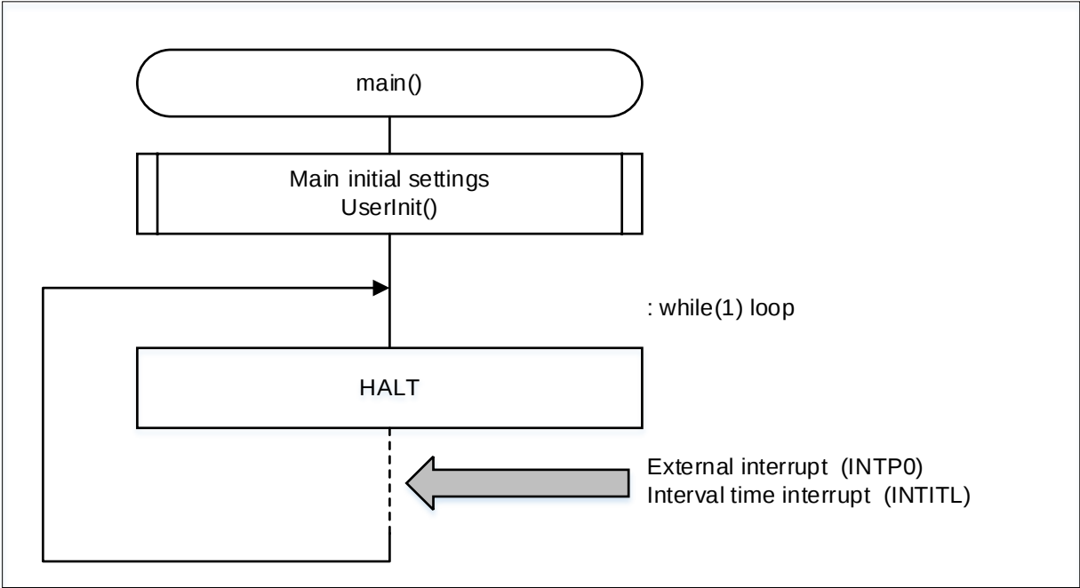
Figure 4-1 Main Processing
