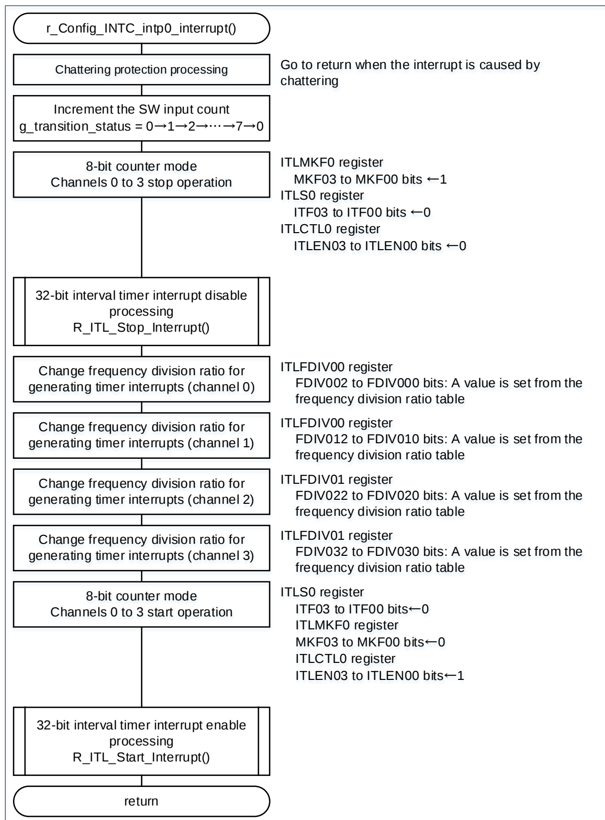
Figure 4-7 External Interrupt (INTP0) Processing
