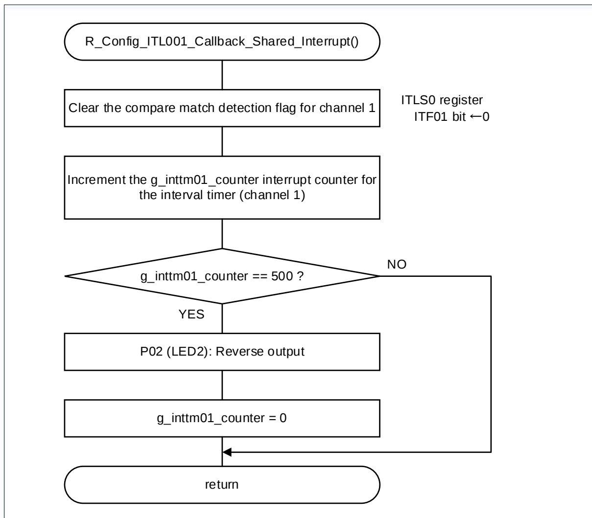
Figure 4-4 Interrupt Processing for Interval Timer Channel 1
