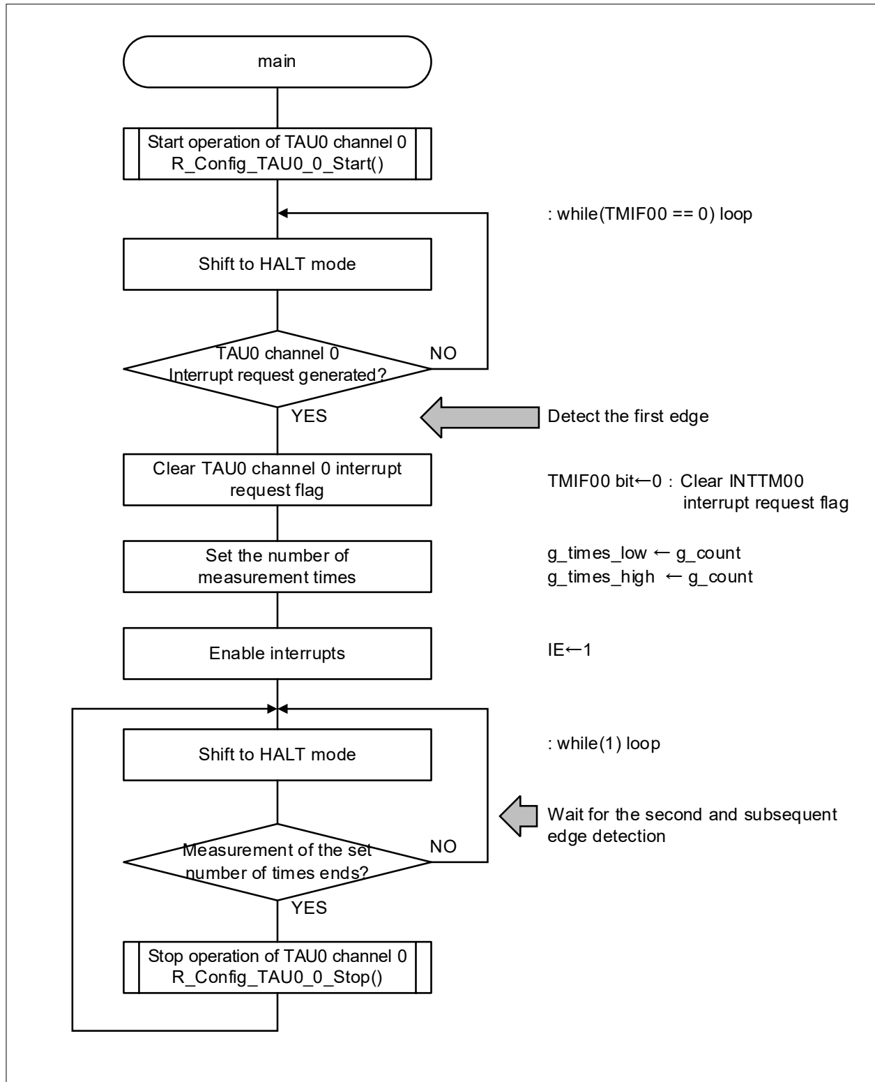
Figure 4-1 Main Processing
