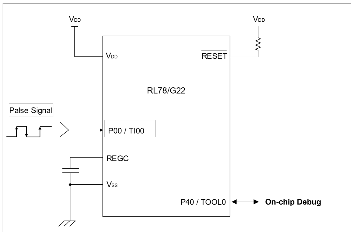
Figure 3-1 Hardware Configuration
