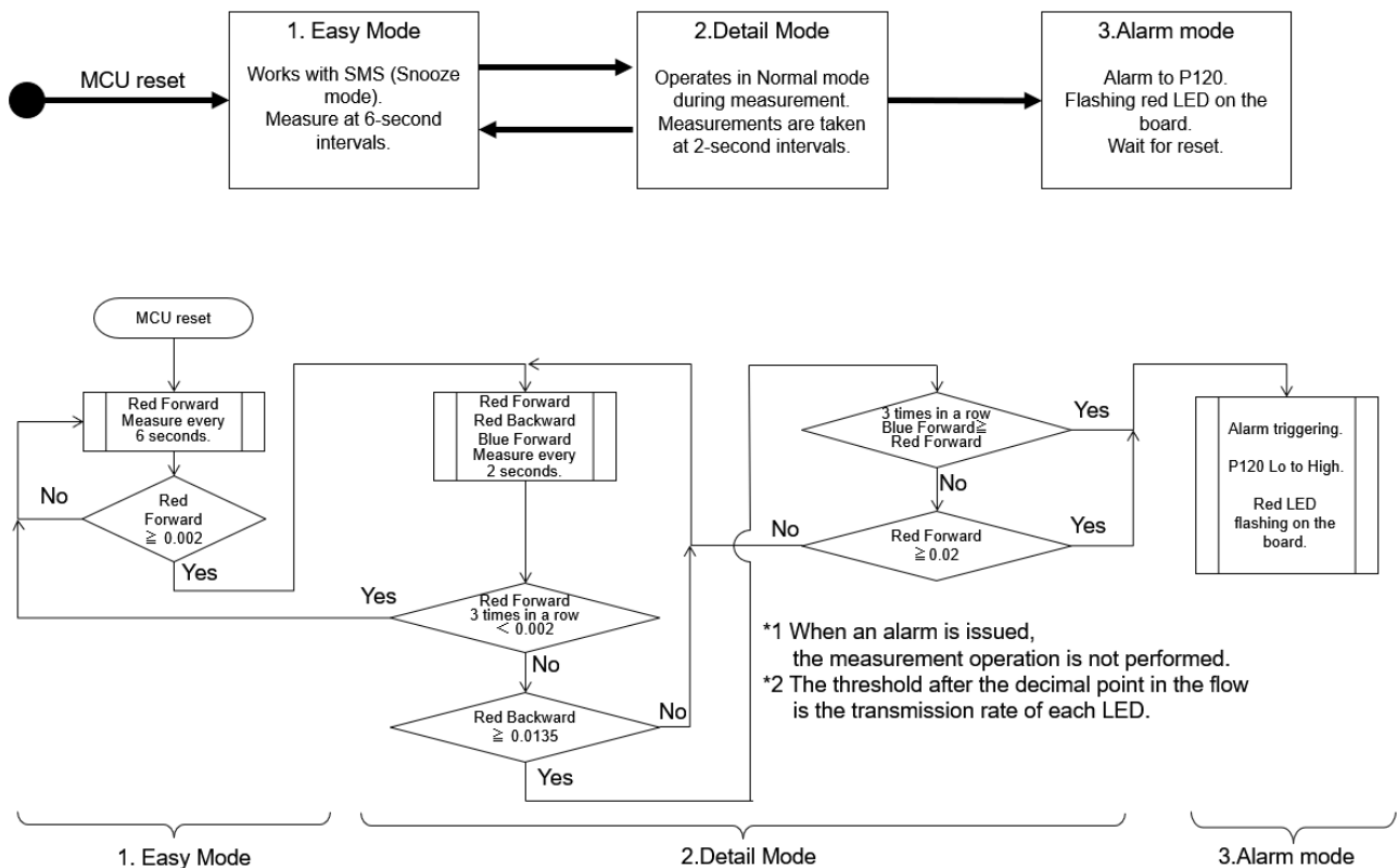
Figure 5-1. Judgment Flow Diagram of the Smoke Detection Algorithm
