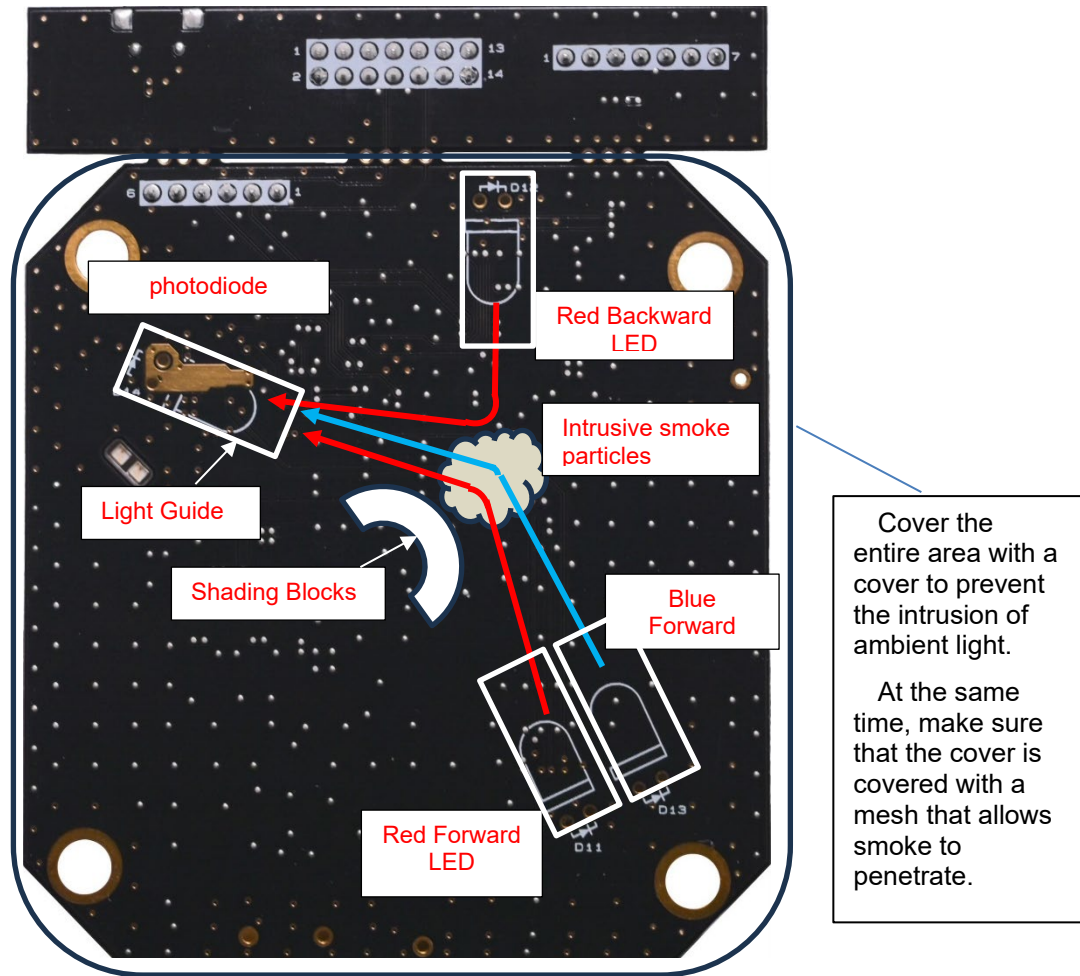
Figure 4-1. Smoke Chamber Structure
