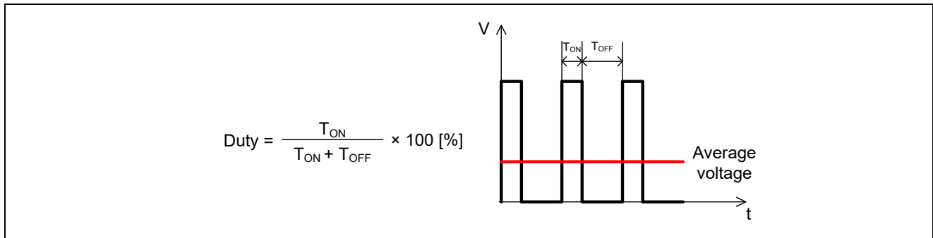
Figure 3-1 PWM Control
