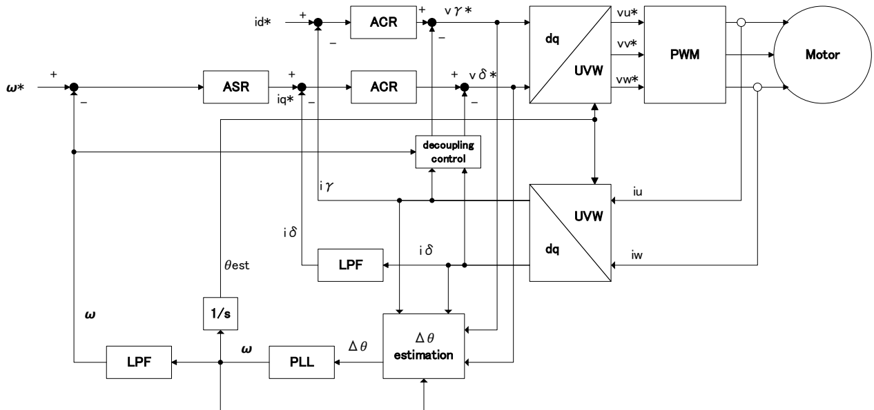
Figure 3-5 Control System Block Diagram
