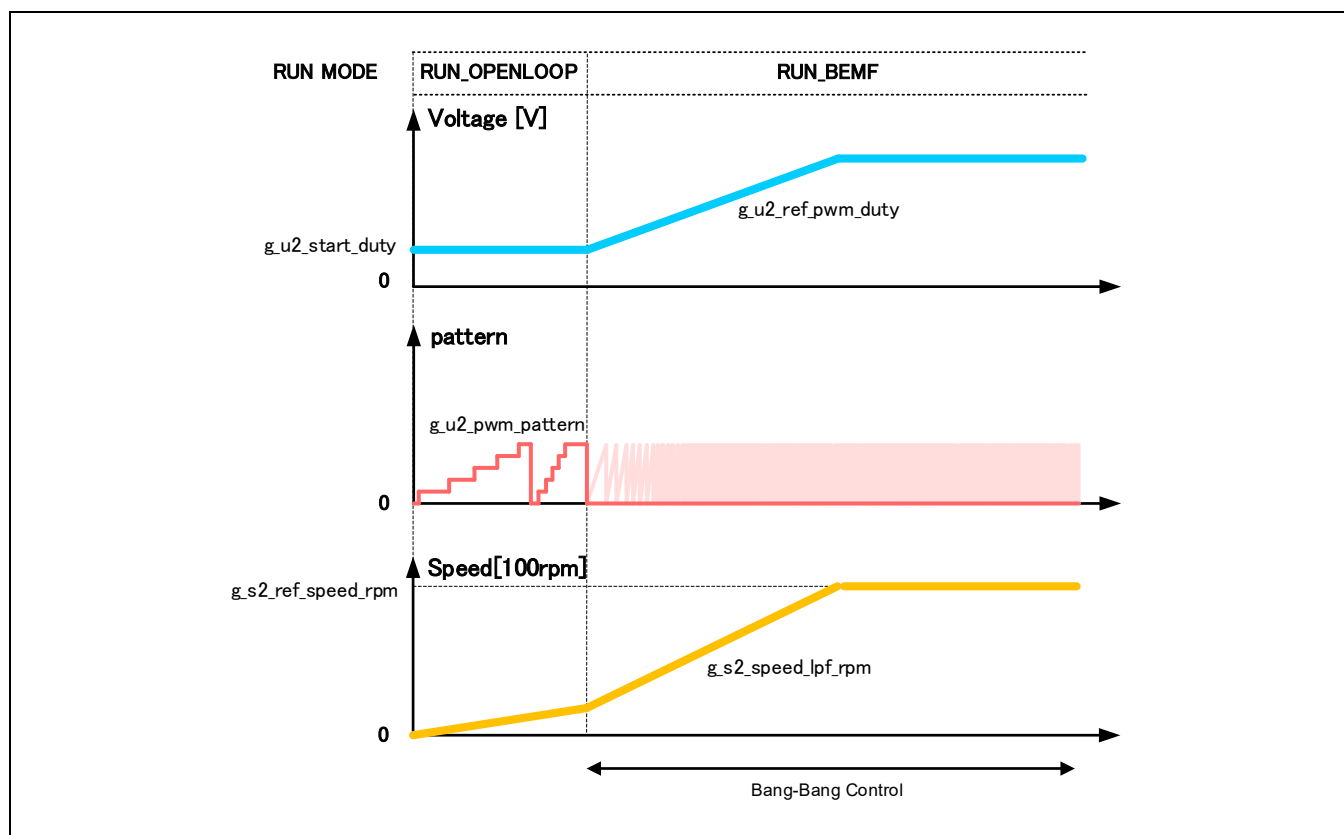
Figure 3-8 – Startup sequence
