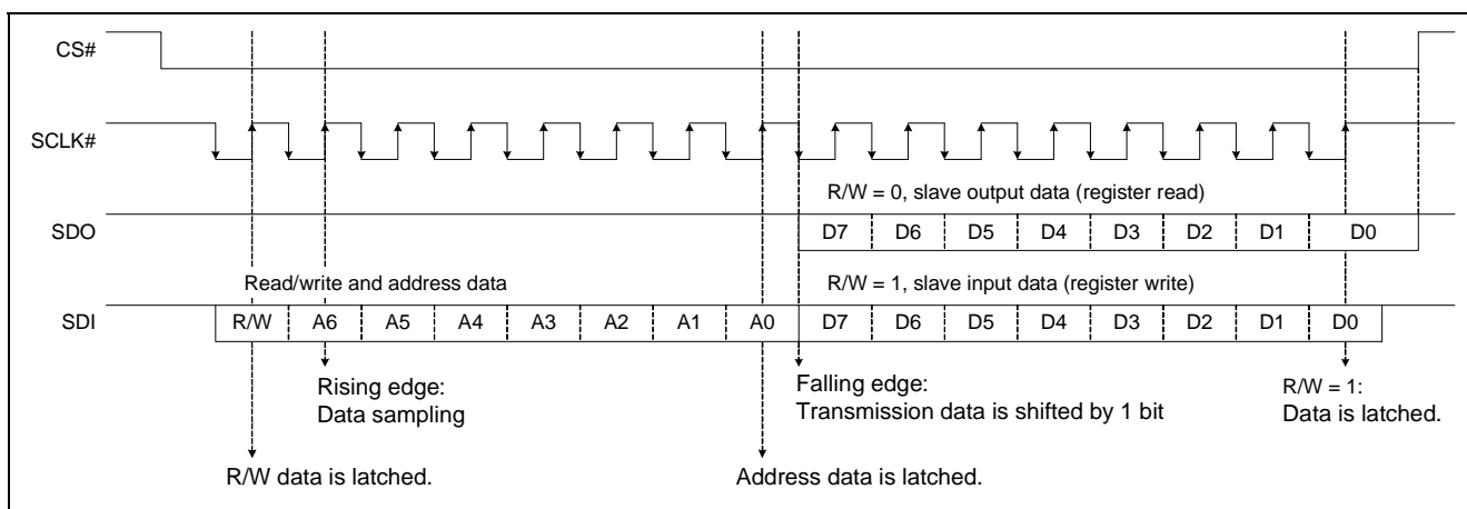
Figure 6.7 SPI Communication Timing
