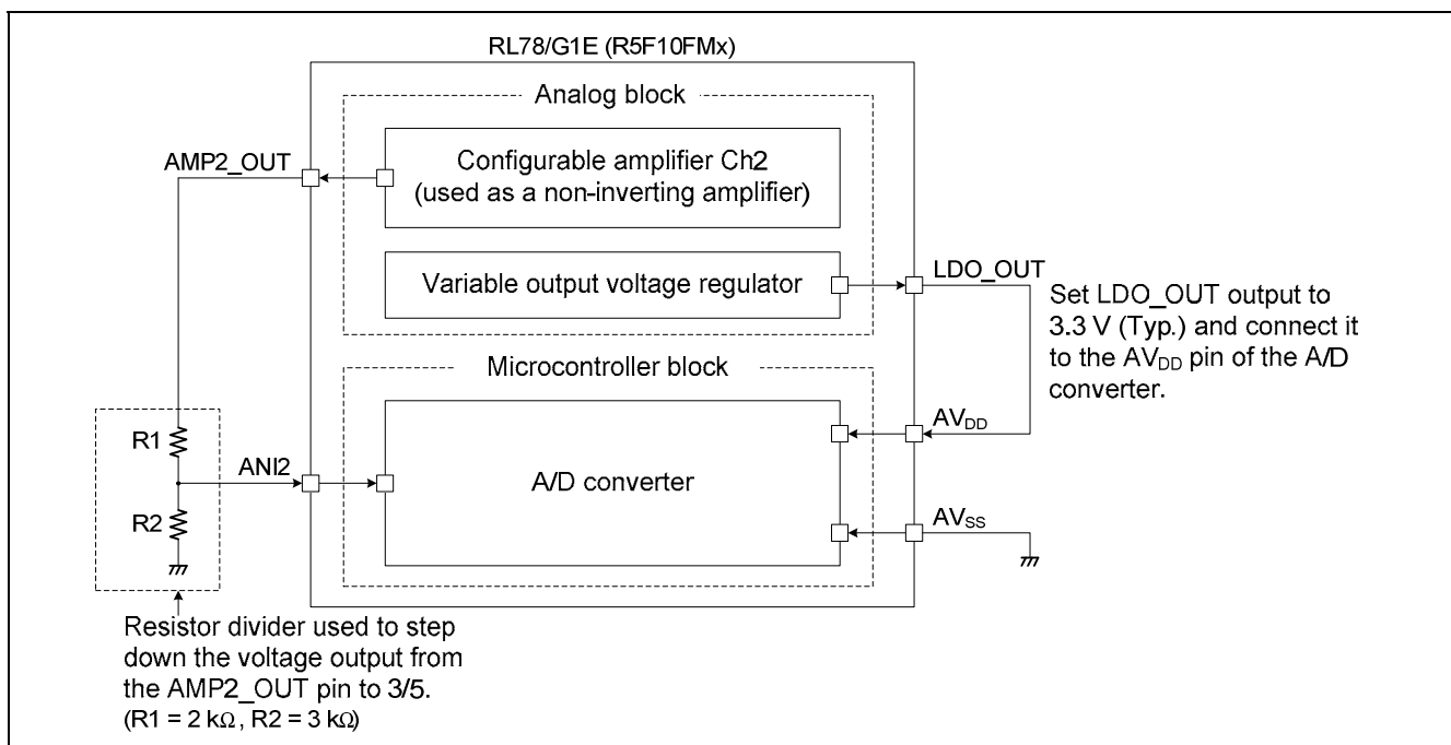
Figure 5.6 Connection Between Configurable Amplifier Ch2 (Used As a Non-Inverting Amplifier) and A/D Converter
