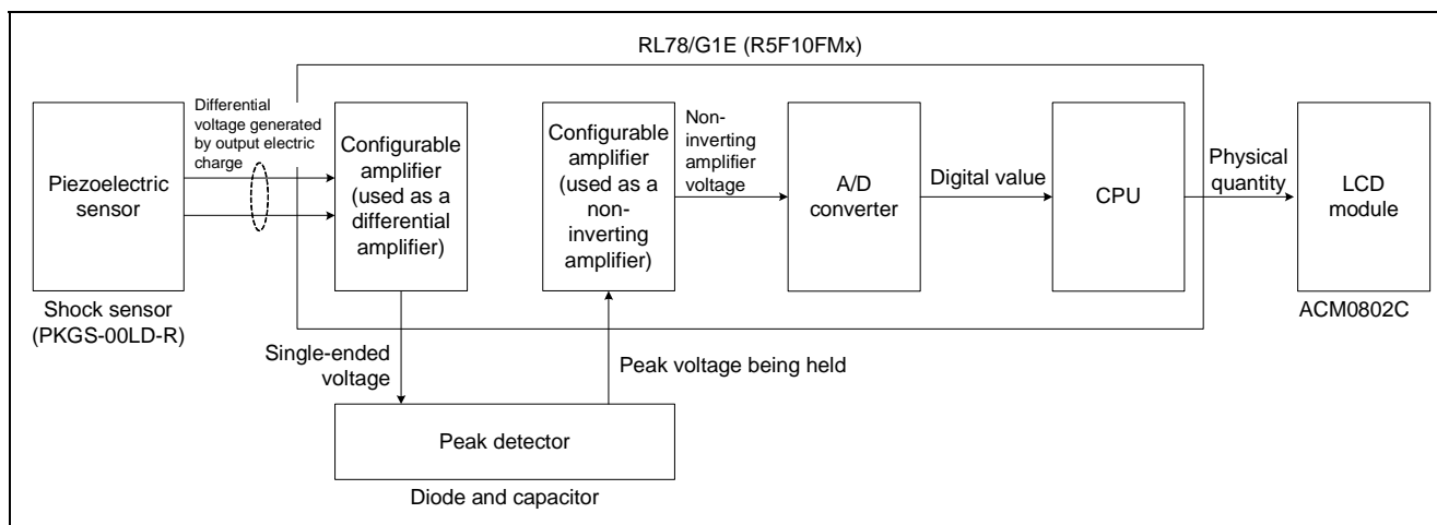
Figure 1.1 Block Diagram
