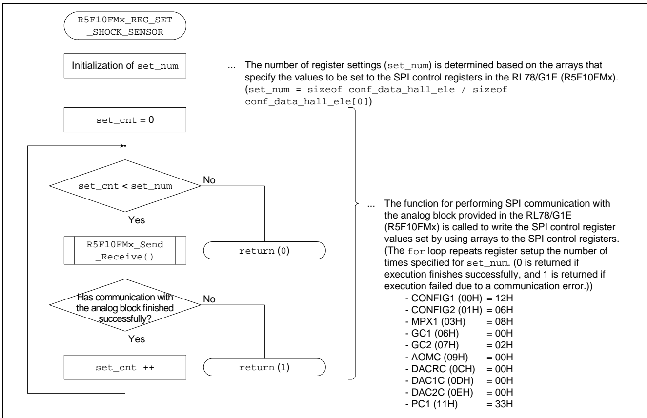
Figure 7.21 Flowchart of R5F10FMx_REG_SET_SHOCK_SENSOR Function
