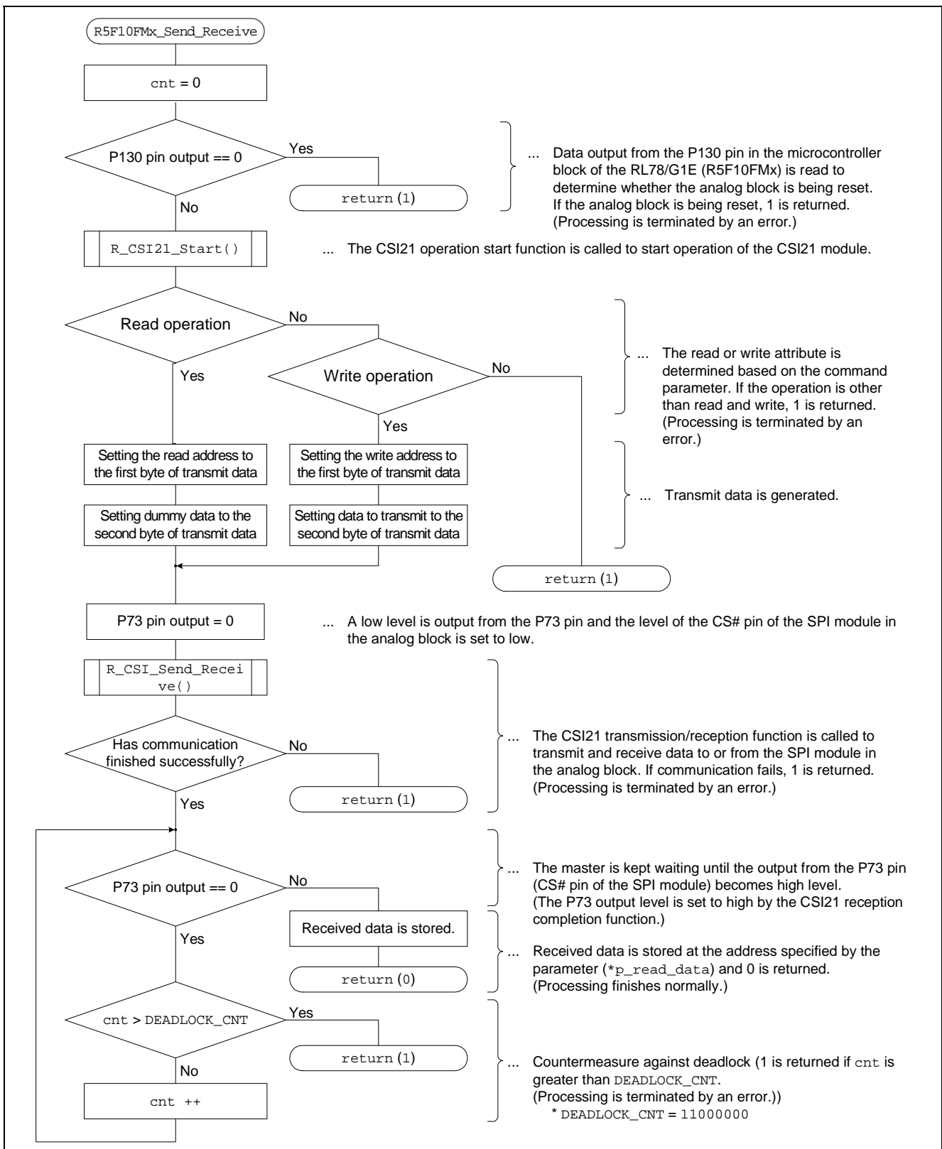
Figure 7.22 Flowchart of R5F10FMx_Send_Receive Function
