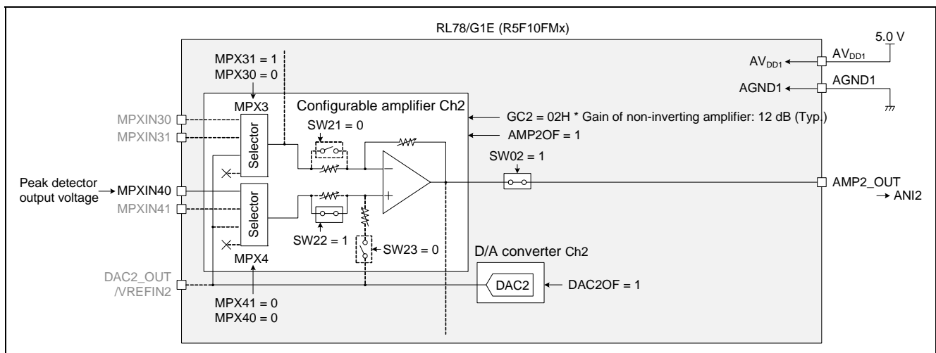
Figure 6.3 Block Diagram of Configurable Amplifier Ch2 (Used As a Non-Inverting Amplifier)
