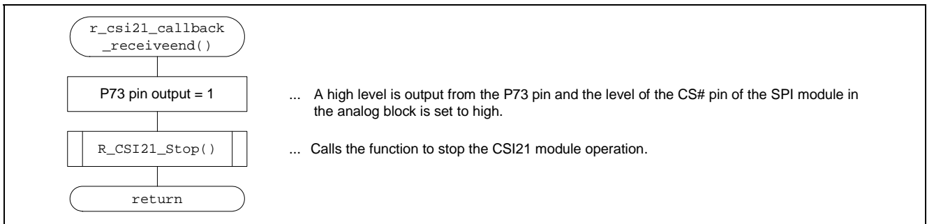
Figure 7.23 Flowchart of r_csi21_callback_receiveend Function
