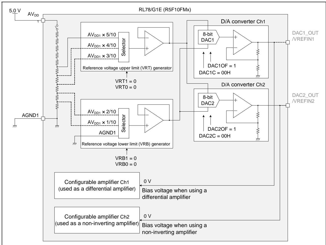
Figure 6.5 Block Diagram of D/A Converter
