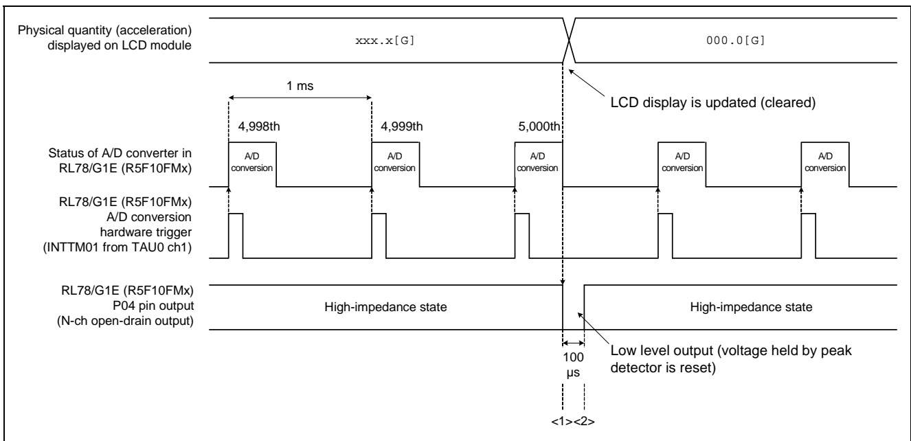
Figure 7.14 Timing of Resetting Voltage Held by Peak Detector
