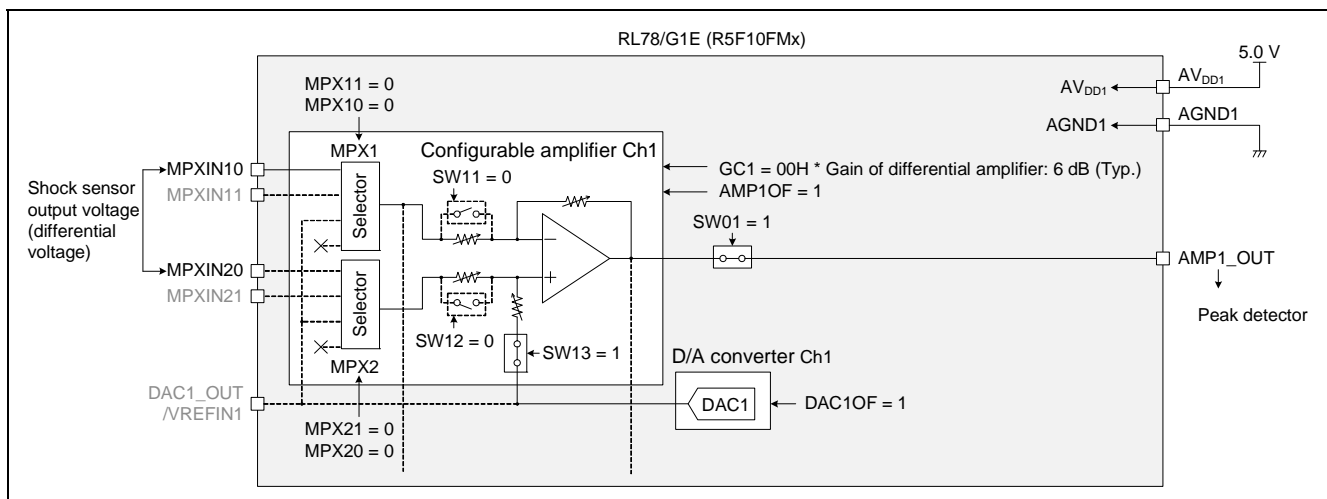
Figure 6.2 Block Diagram of Configurable Amplifier Ch1 (Used As a Differential Amplifier)
