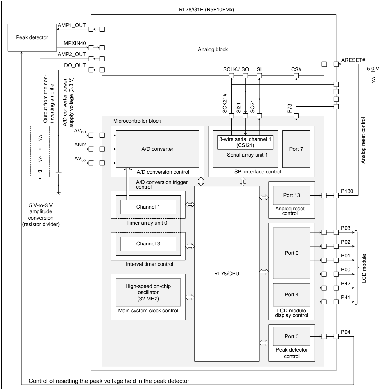
Figure 7.1 Function Blocks in the Microcontroller Block of the RL78/G1E (R5F10FMx)
