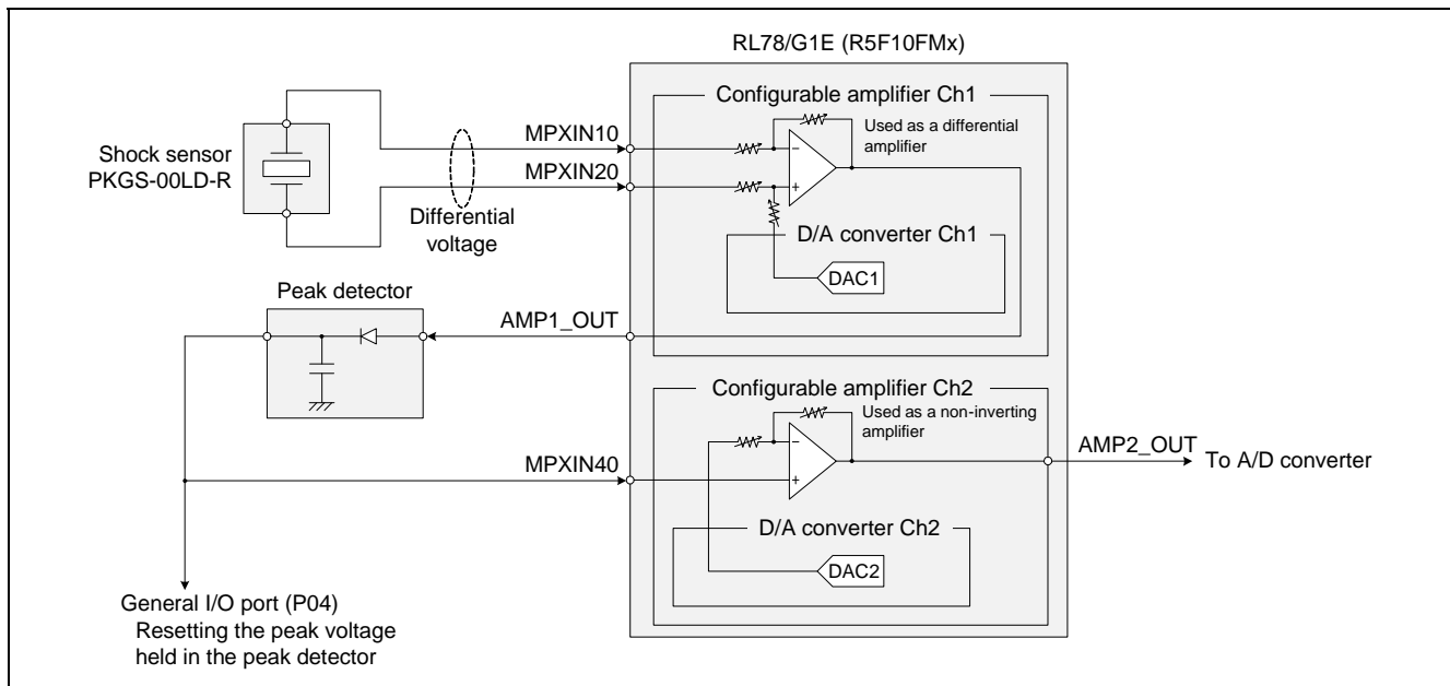
Figure 5.4 Amplifier and Signal Converter for Amplifying and Converting Shock Sensor Output Voltage
