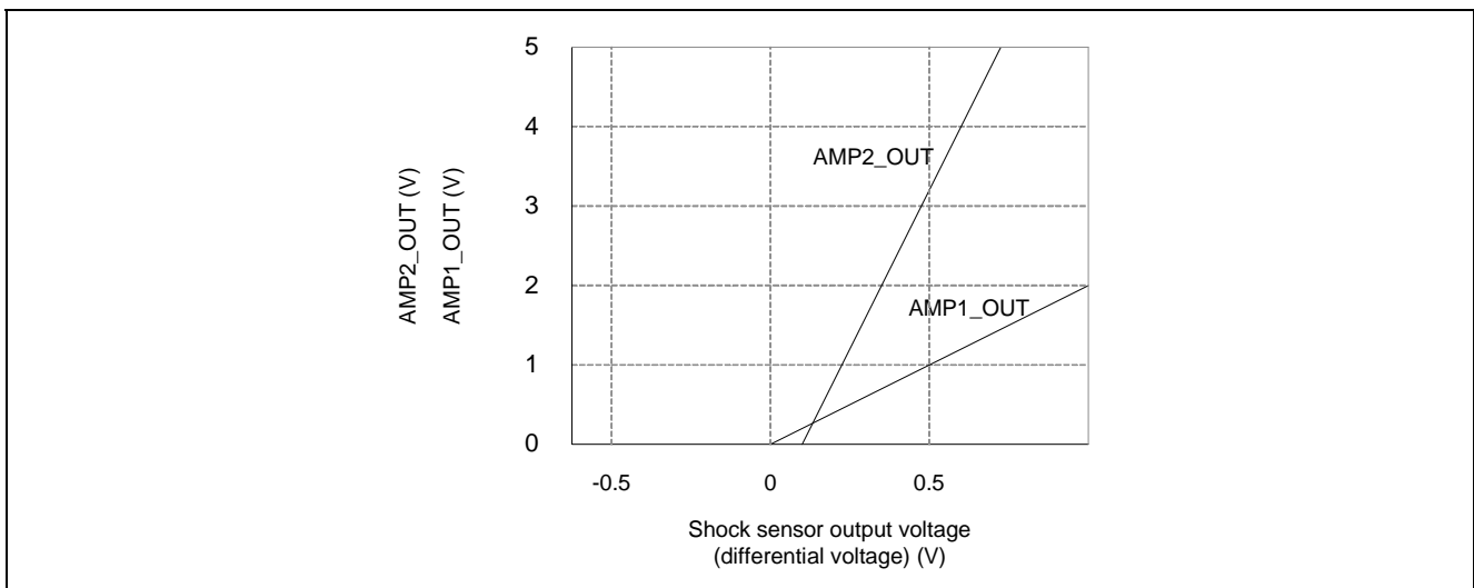
Figure 5.5 Shock Sensor Output Voltage (Differential Voltage) vs. Differential Amplifier Output (AMP1_OUT) and Non-Inverting Amplifier Output (AMP2_OUT)
