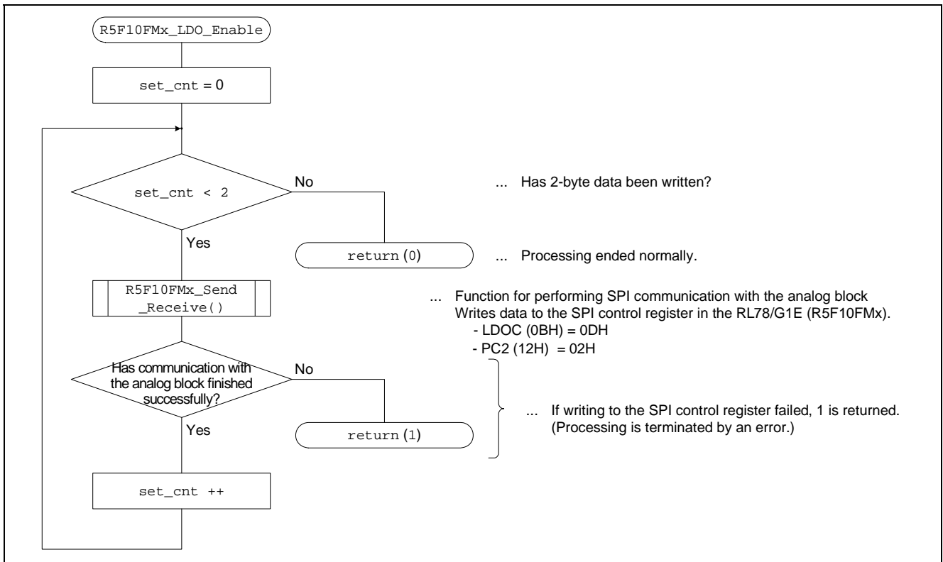
Figure 7.20 Flowchart of R5F10FMx_LDO_Enable Function
