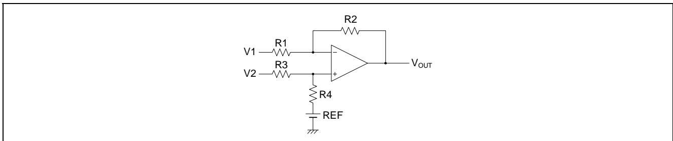
Figure 5.2 General Differential Amplifier
