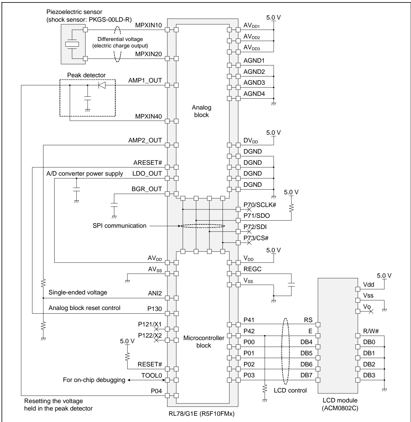
Figure 4.1 Hardware Configuration
