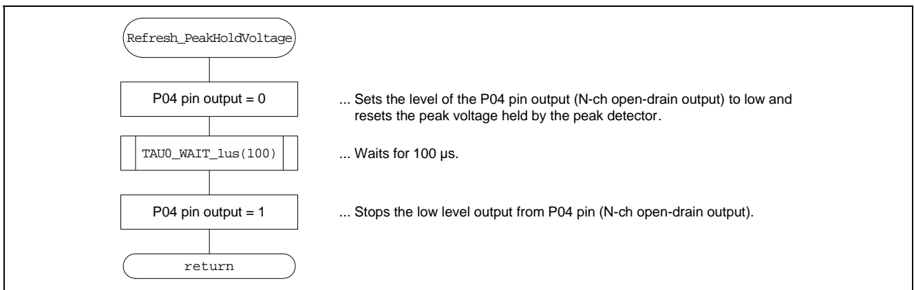
Figure 7.24 Flowchart of Refresh_PeakHoldVoltage Function
