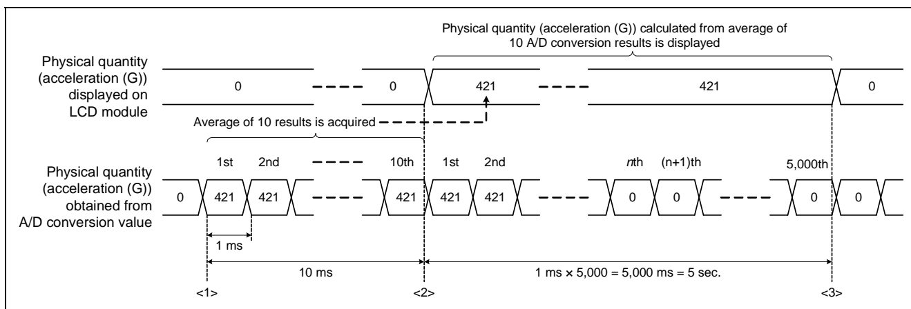
Figure 7.13 Timing of LCD Module Display Update
