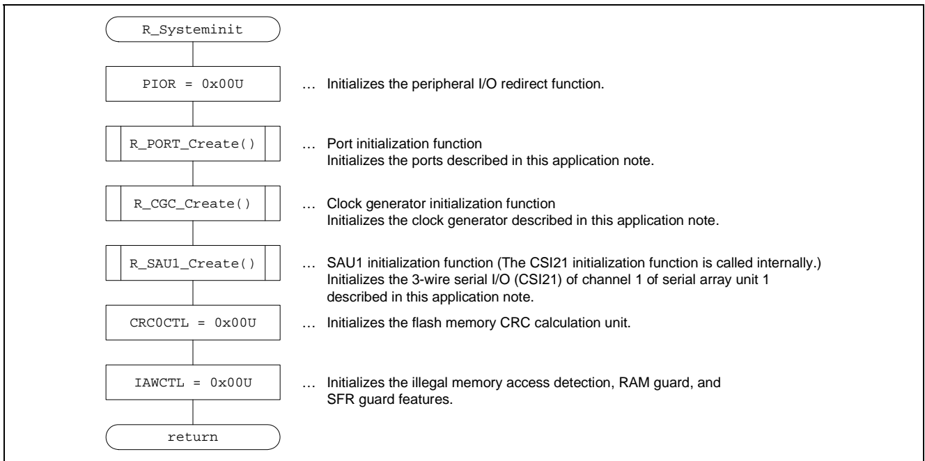
Figure 7.17 Flowchart of R_Systeminit Function
