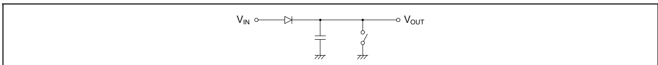
Figure 5.3 General Peak Detector
