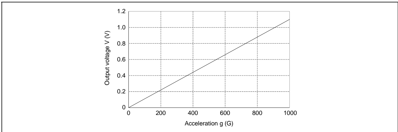
Figure 5.1 Sensitivity of Shock Sensor PKGS-00LD-R
