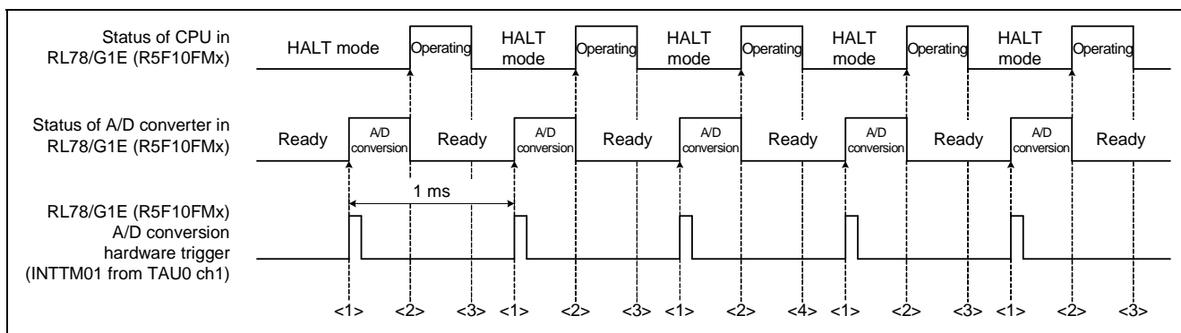
Figure 7.12 Timing of A/D Conversion
