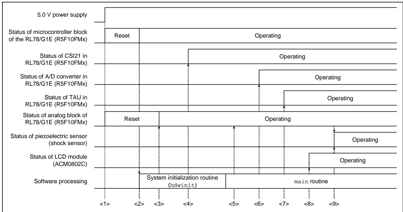
Figure 7.11 Timing Between Power Application and Initial Setup
