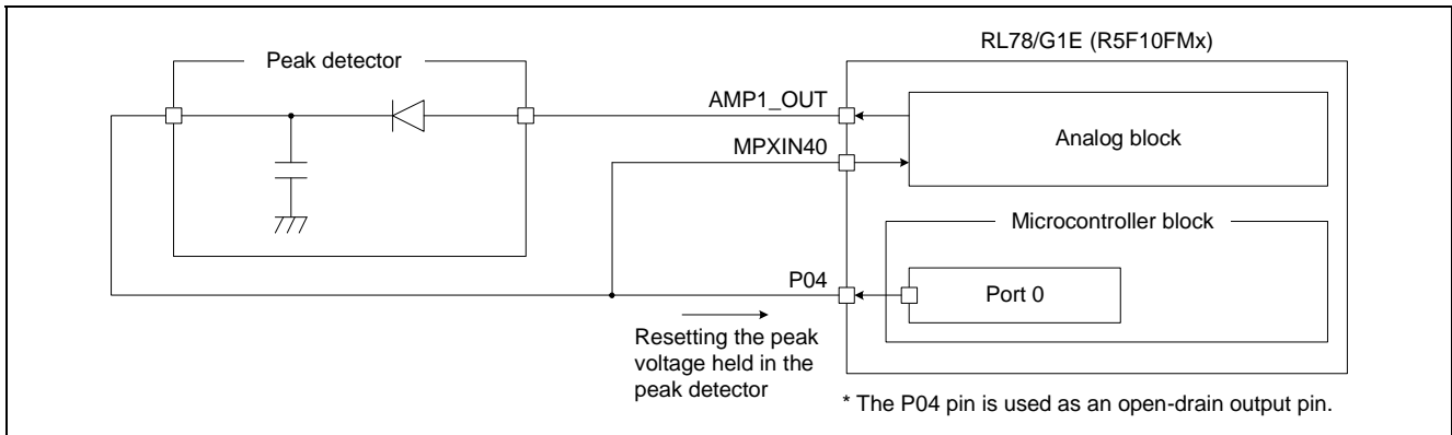
Figure 7.10 Connection Between Peak Detector and P04 Pin
