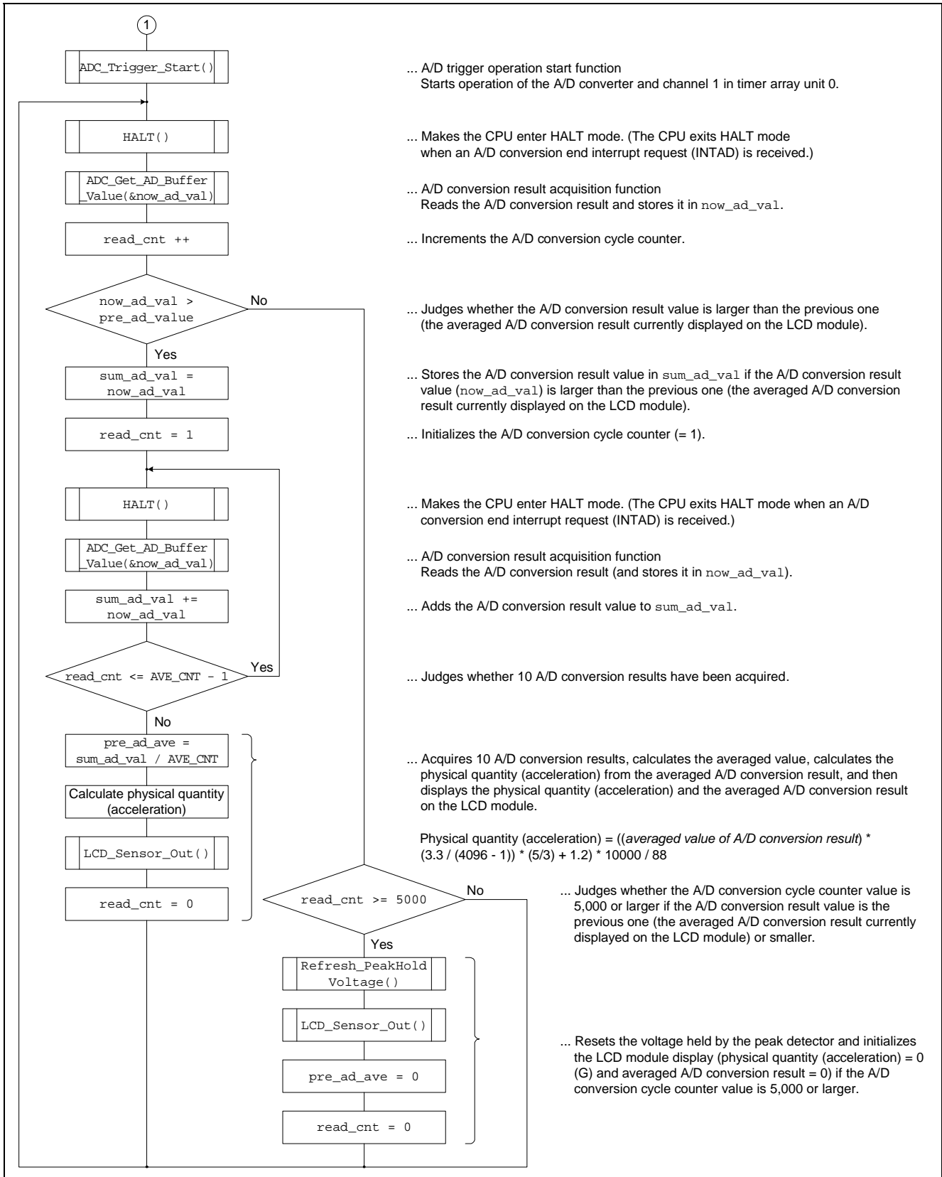
Figure 7.19 Flowchart of main Function (2)
