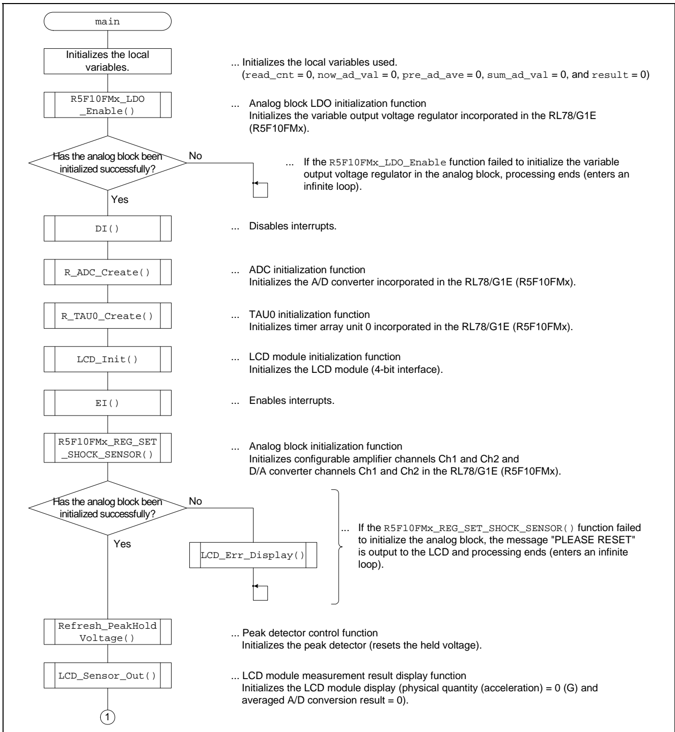
Figure 7.18 Flowchart of main Function (1)
