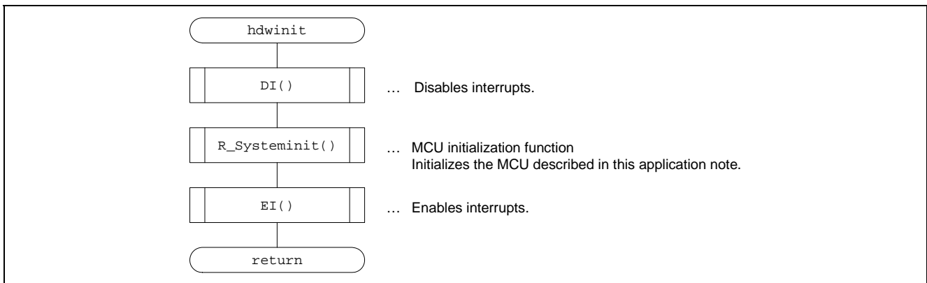
Figure 7.16 Flowchart of hdwinit Function
